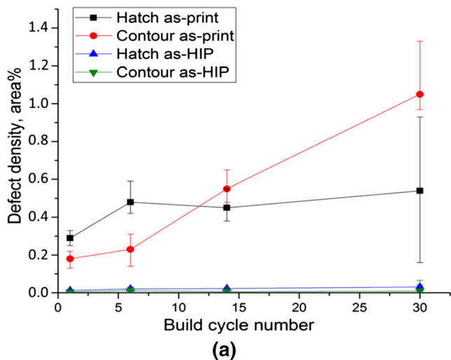
Fig. 9—Defect density in the hatch and contour region measured in (a) as-printed and as-HIP condition (b) as-HIP condition. The error bars indicate the actual measurement range. All data points are average values obtained from measurements in the cross-sections “bottom” and “below top”, as indicated in Fig. 1(b).
