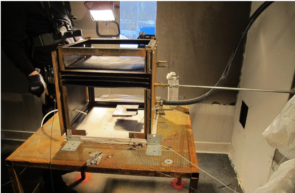
Figure 13 The connection of the nitrogen gas hose line to the side of the simulated battery module, as seen from the back side. With this approach the gas was not required to pass through the perforated steel sheet plates at the top of the module.
