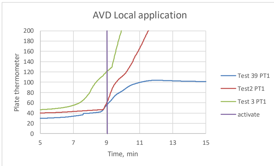
Figure A.14. AVD direct injection test
