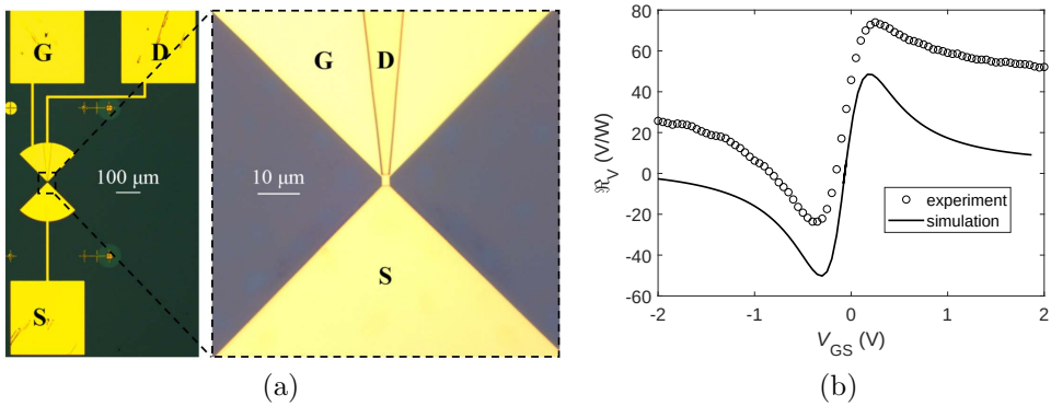
Figure 6.2: (a) Optical micrograph and (b) experimental (symbols) and simulated (solid line) voltage responsivity as a function of gate voltage of the GFET detector in [Paper D] at 400 \text{ GHz} .
