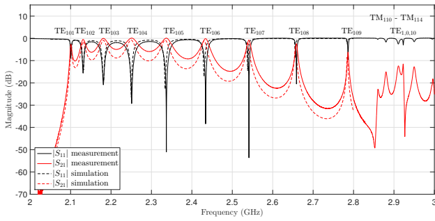
Figure 2. Measured and simulated S-parameters for the empty sensor.
