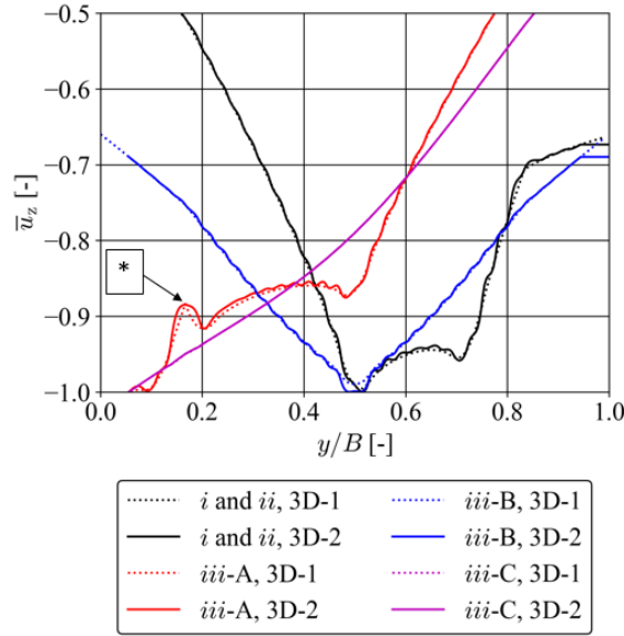
Figure 44. Vertical deflection of equivalent single layer model (3D-1) and 3D shell element model (3D-2) [Paper III].
