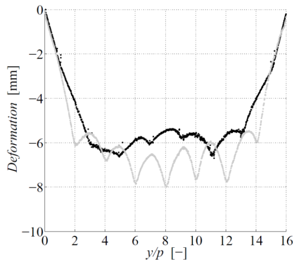
Figure 13. Face plate deformations of produced panel obtained from 3D scanning. Grey curve indicate measurement of the bottom face while the black curve show the top face. [Paper I].
