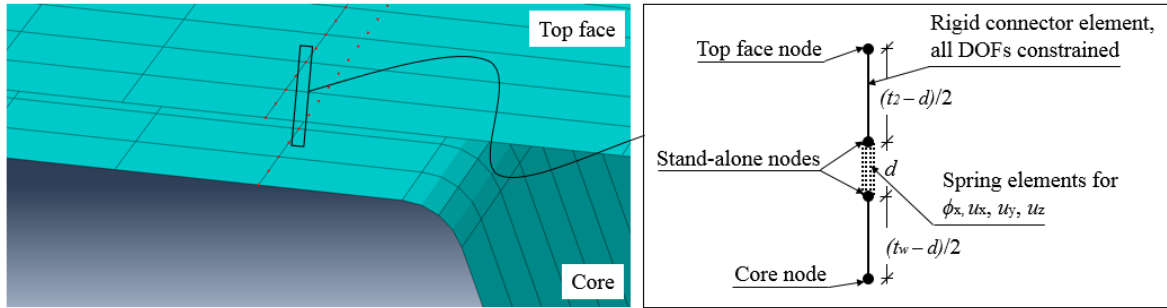
Figure 30. Modelling of weld region stiffness springs [Paper III].
