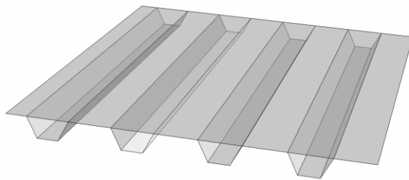
Figure 2. Conventional OSD with longitudinal trapezoidal stiffeners.
