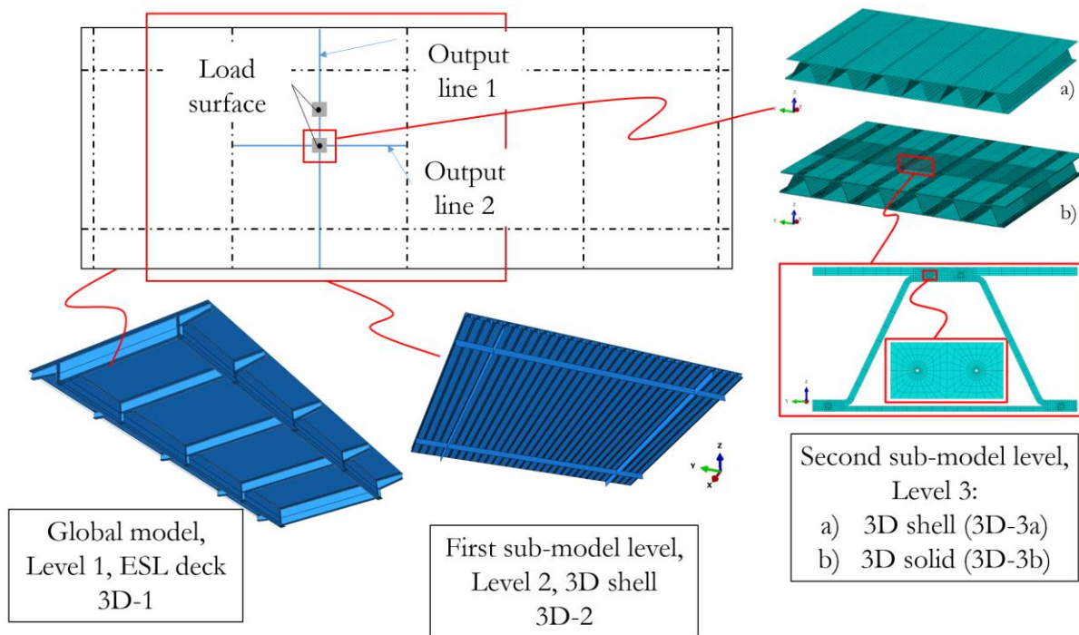
Figure 41. Three-level multiscale model for the ESL approach, and solid model 3D-3b for verification.
