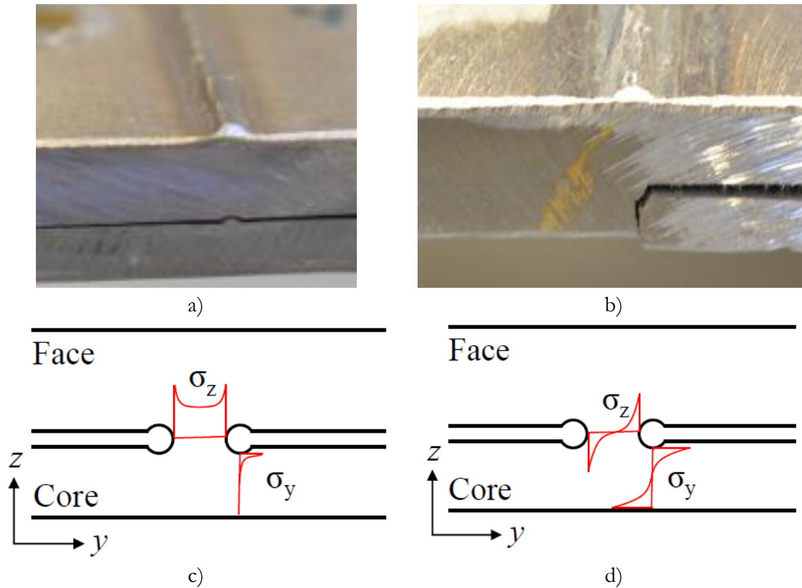
Figure 20. Photo of fractured part, a) weld-crack (LC1), b) core crack (LC2) and principal stress distributions for c) LC1, d) LC1 [Paper II].
