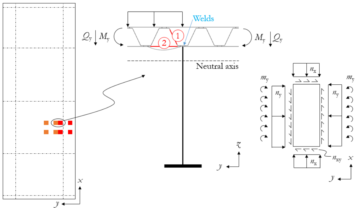
Figure 55. Load situation for Region iii-A .
