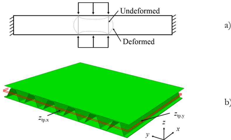
Figure 47. Sources of error in Equivalent Single Layer model for predictions of panel-level sectional forces; a) through thickness compression effect and b) effect of shape-orthotropy.
