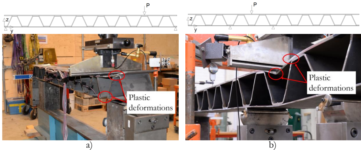
Figure 38. Failure load tests; a) failure at support where panel-level shear force drives the deformation b) failure of loaded plate.
