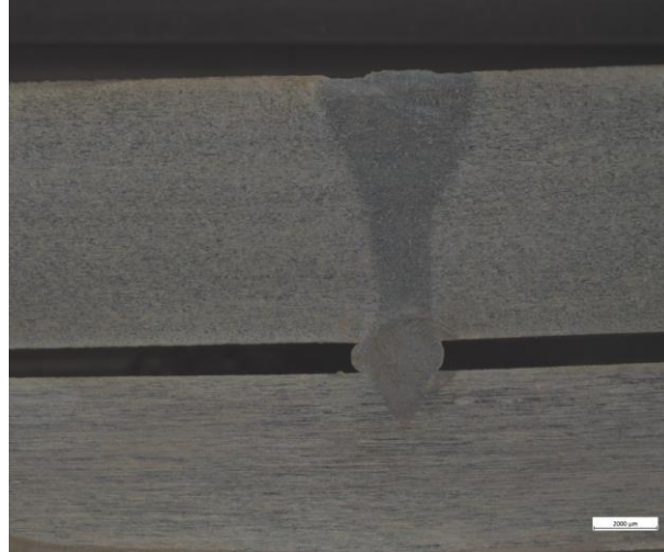
Figure 10. Miss-shaped weld due to large plate gap.
