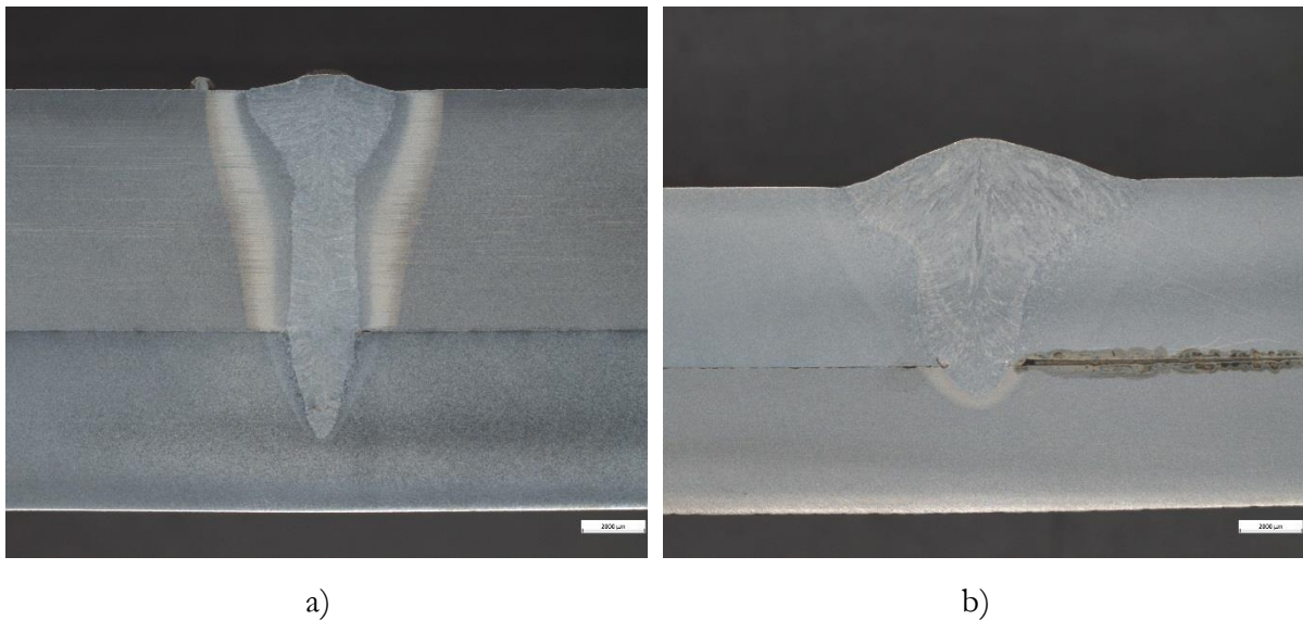
Figure 7. Microscopic images from stake-weld cross section; a) pure laser, b) hybrid laser-arc.
