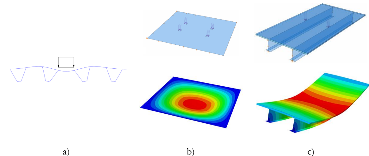
Figure 1. Bridge deck actions; a) local action due to wheel pressure, b) plate action for load distribution, c) flange action for global stiffness.
