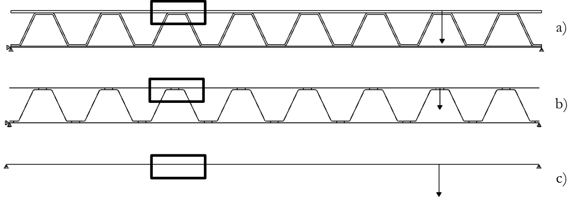
Figure 33. Three different levels of structural analysis; a) 2D solid element FEA, b) 2D beam element FEA, c) analytical homogenous beam analysis. The rectangular boxes indicate the investigated area/output region.
