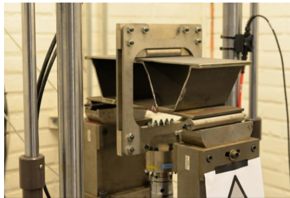
Figure 17. Fatigue test setup for cell specimens [Paper II]
