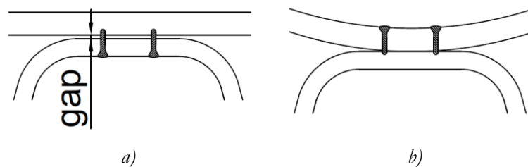
Figure 32. Sources for lack of plate interaction; a) gap, and b) welding deformation [Paper V].
