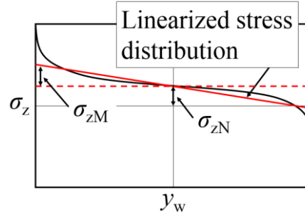
Figure 29. Calculation of nominal stresses from the stress distribution of the solid element model, [Paper III].
