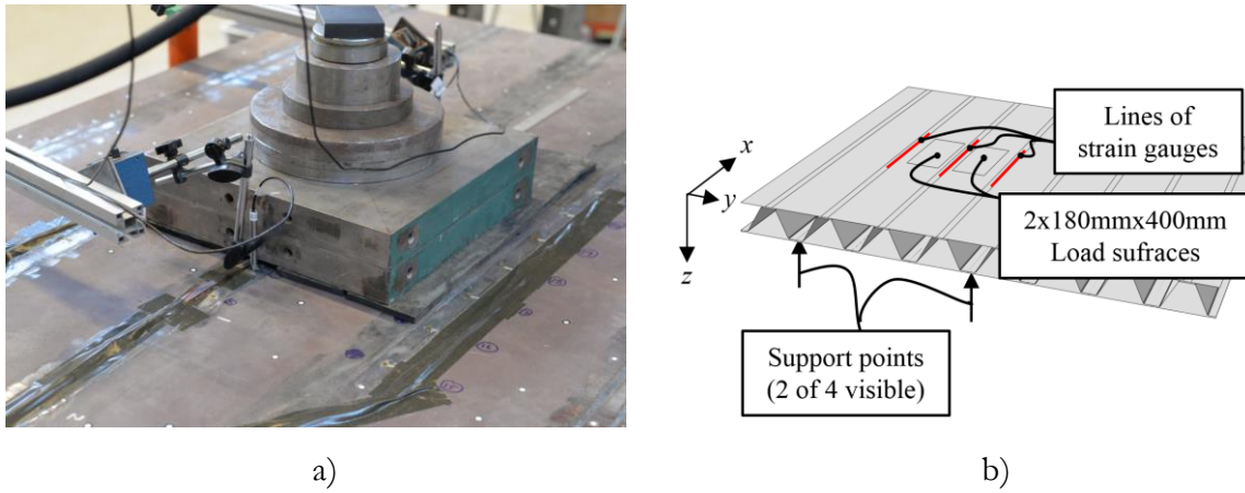
Figure 19. Panel test setup; a) load application, b) schematic of load, support and strain gauges. [Paper II]
