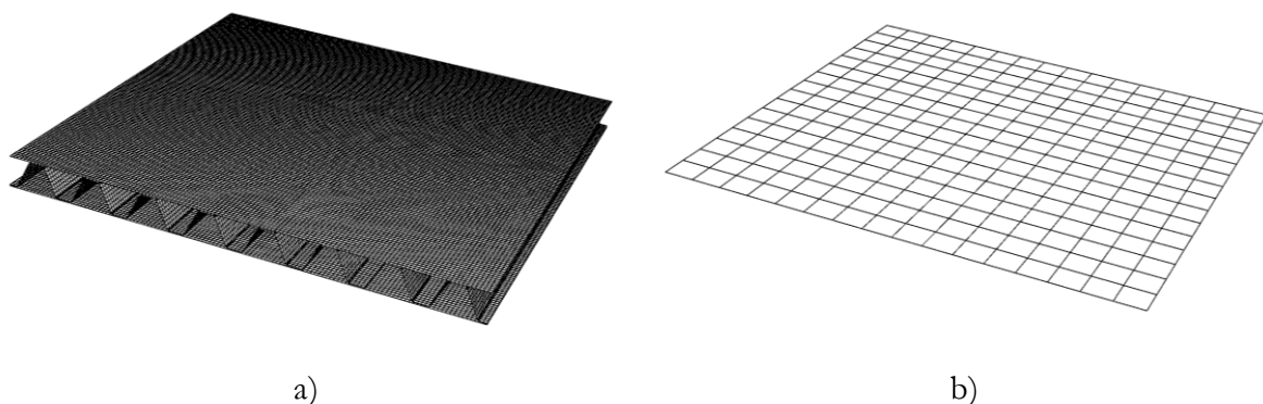
Figure 22. Principal mesh sketch; a) 3D shell element model, and b) ESL.
