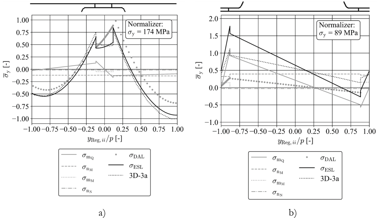
Figure 50. Comparison of stresses for the ESL-approach and a 3D shell element model (3D-3a) in a region subjected to panel-level sectional forces and directly applied load (DAL); a) top face, and b) bottom face [Paper III].
