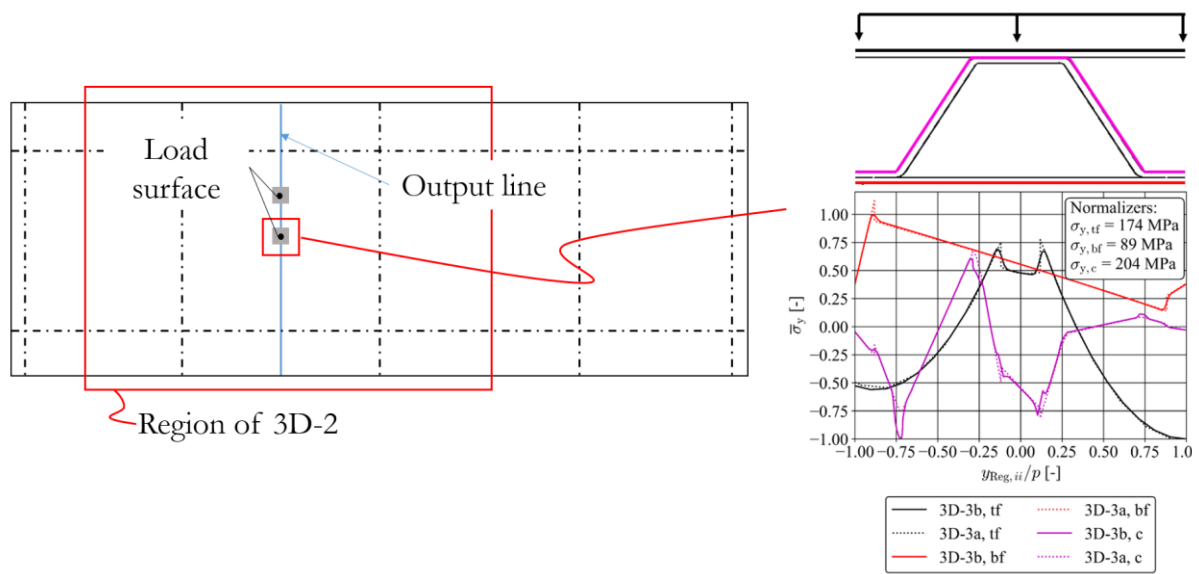
Figure 51. Position and load situation for Region ii and normal stress in the outer surface of the top and bottom face and the core for shell and solid models 3D-3a and 3D-3b, respectively [Paper III].
