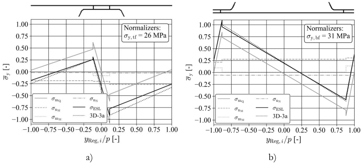
Figure 49. Comparison of stresses for the ESL-approach and a 3D shell element (3D-3a) model in a region subjected to panel-level sectional forces alone; a) top face, and b) bottom face [Paper III].
