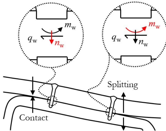
Figure 16. Contact and splitting action in corrugated core steel sandwich panels with dual weld lines.
