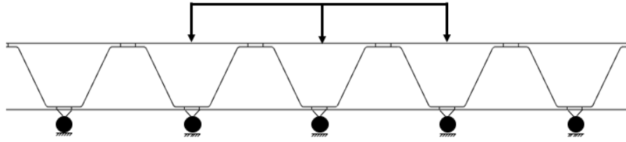
Figure 42. DAL-model for ESL-approach [Paper III].
