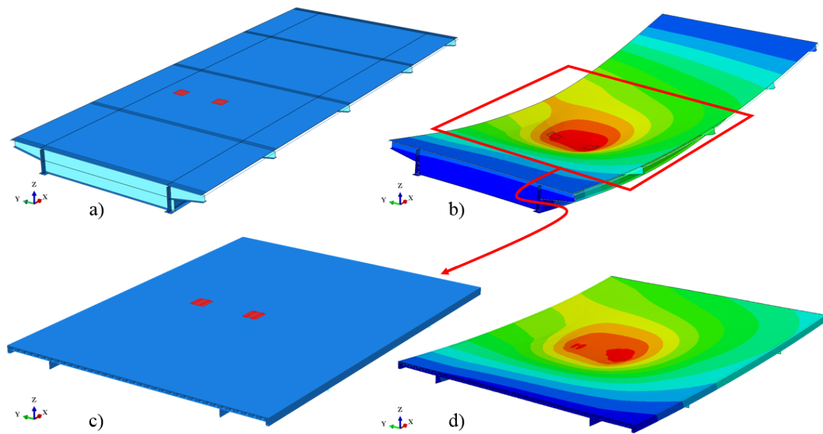
Figure 23. Principle sketch of sub-model approach; a) Level 1 undeformed (red highlighted regions are patch loads), b) Level 1 deformed, deformations in the highlighted region are used as boundary condition for Level 2, c) Level 2 undeformed (red highlighted regions are patch loads), and d) Level 2 deformed shape.
