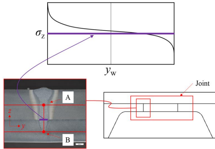
Figure 28. Core-to-face joint and weld region.
