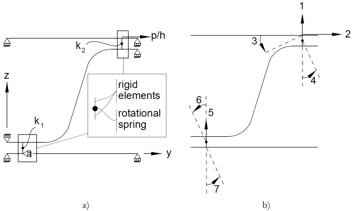
Figure 27. a) Structural setup for derivation of the transverse shear stiffness b) included degrees of freedom. [Paper IV].
