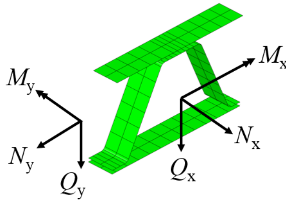
Figure 45. Orientations for panel-level sectional force, [Paper III].
