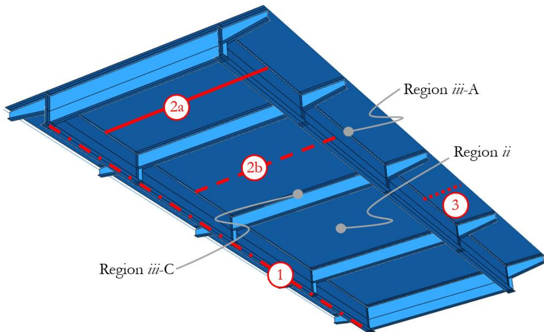
Figure 53. Parts of the bridge that are controlled for deformations; 1) main girder, 2) deck, and 3) cantilever.
