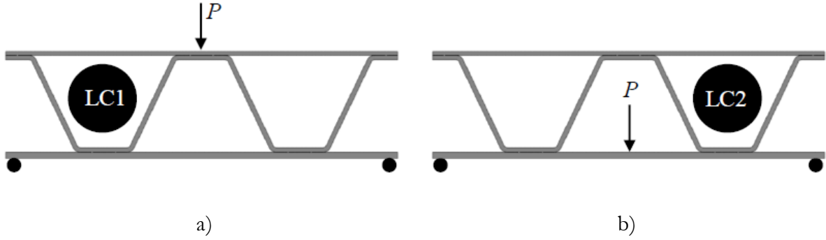
Figure 18. Load-cases for fatigue tests of cell-specimens; a) LC1 and b) LC2 [Paper II]
