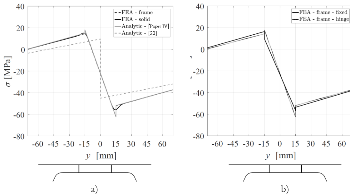
Figure 34. Normal stress distribution in the top fiber of the top face; a) comparison between 2D solid and frame numerical models and 1D analytical models and b) 2D numerical model with rotationally fixed core-to-face plate interaction at the welds compared to equivalent model with rotational hinge.
