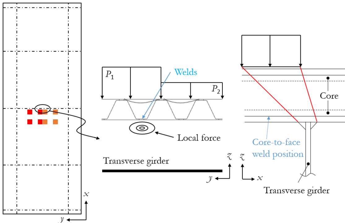
Figure 56. Load situation for Region iii-C .
