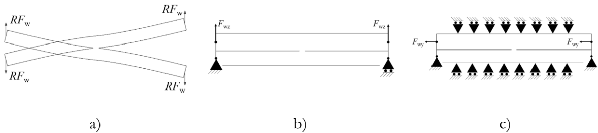
Figure 31. Structural setups for calculation of spring stiffness components with respect to; a) rotational spring, b) z -direction spring (axial), and c) y -direction spring (perpendicular shear).
