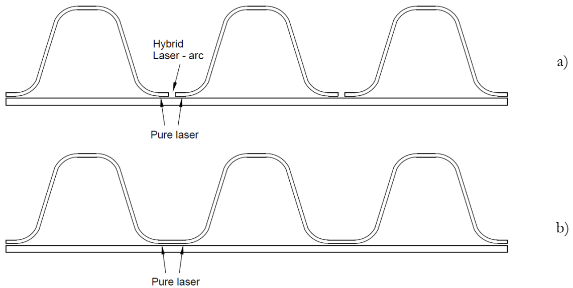
Figure 8. Two ways of manufacturing the continuous core; a) multiple single-wave channels (continuity is created by hybrid laser-arc), and b) continuous cold-formed core plate [Paper I].
