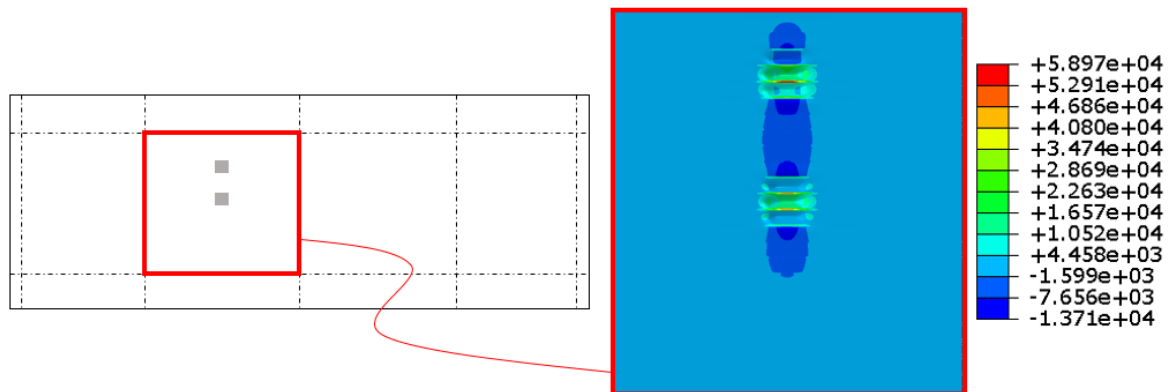
Figure 48. Membrane force, N_y -distribution in top face from 3D shell element model loaded by patch-loads and with restrained vertical deformations.
