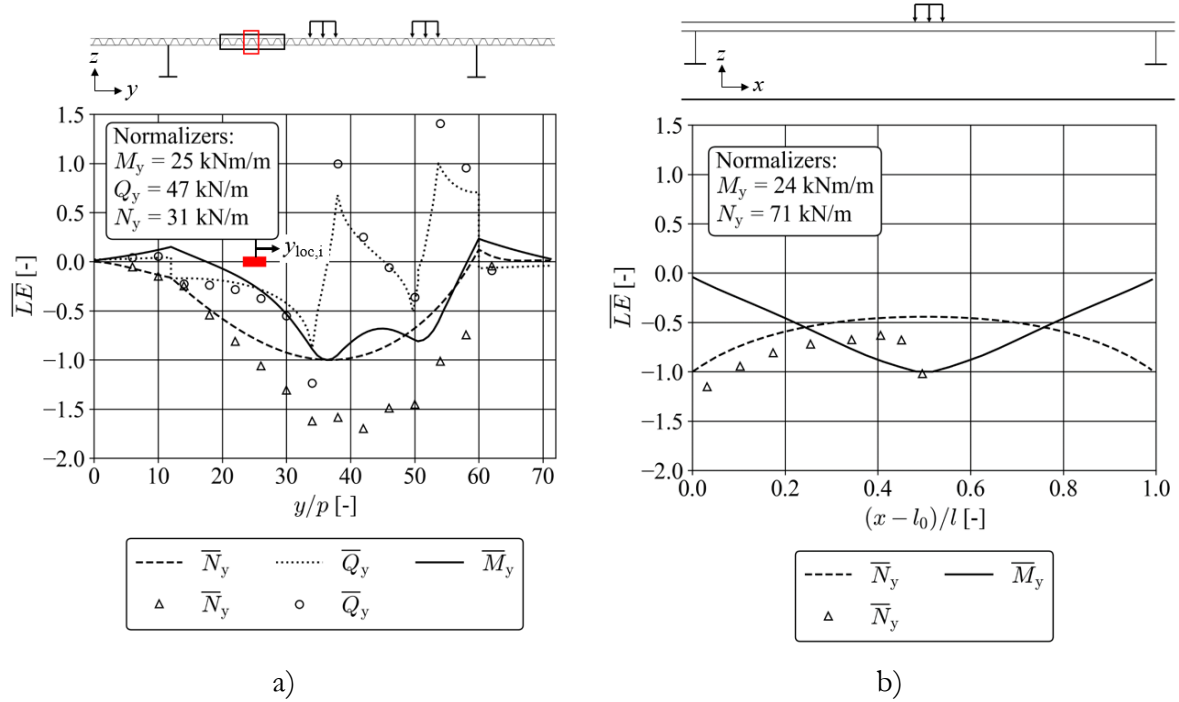
Figure 46. Panel-level membrane force in the weak direction of the panel, N_y ; a) Output line 1 and b) Output line 2, [Paper III].
