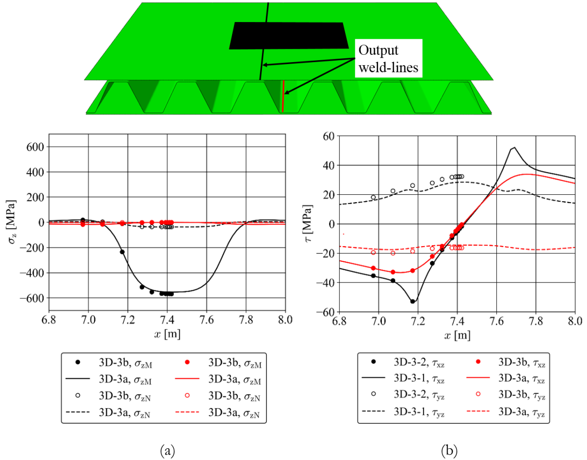
Figure 52. Comparison between shell element model 3D-3a and solid element model 3D-3b with respect to weld stresses; a) normal stress from axial force and bending, and b) shear stress parallel and perpendicular to the weld line [Paper III].
