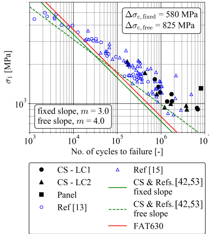
Figure 21. Fatigue test data from the literature and present fatigue tests [Paper II].
