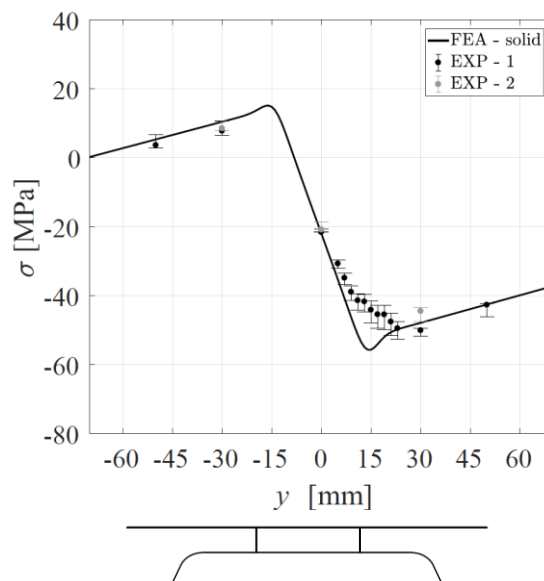
Figure 37. Stress distribution for the case study beam by numerical analysis and experiments.
