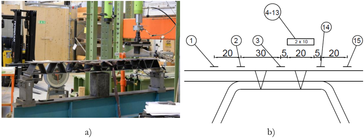
Figure 35. Experiments; a) test setup, b) strain gauges at output joint.
