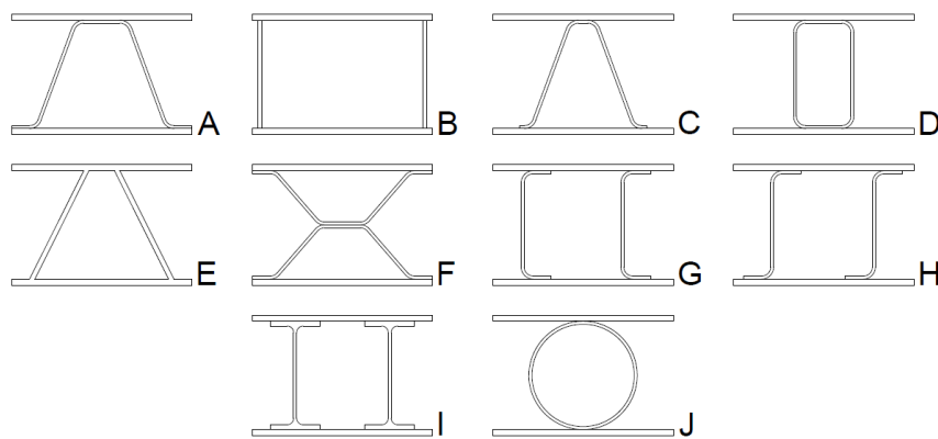
Figure 3. 10 possible structural core sandwich panel geometries [13].
