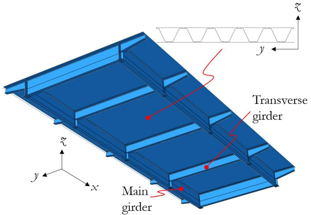
Figure 39. CCSSP in interaction with a supporting structure of longitudinal and transversal girders forming a full structure.
