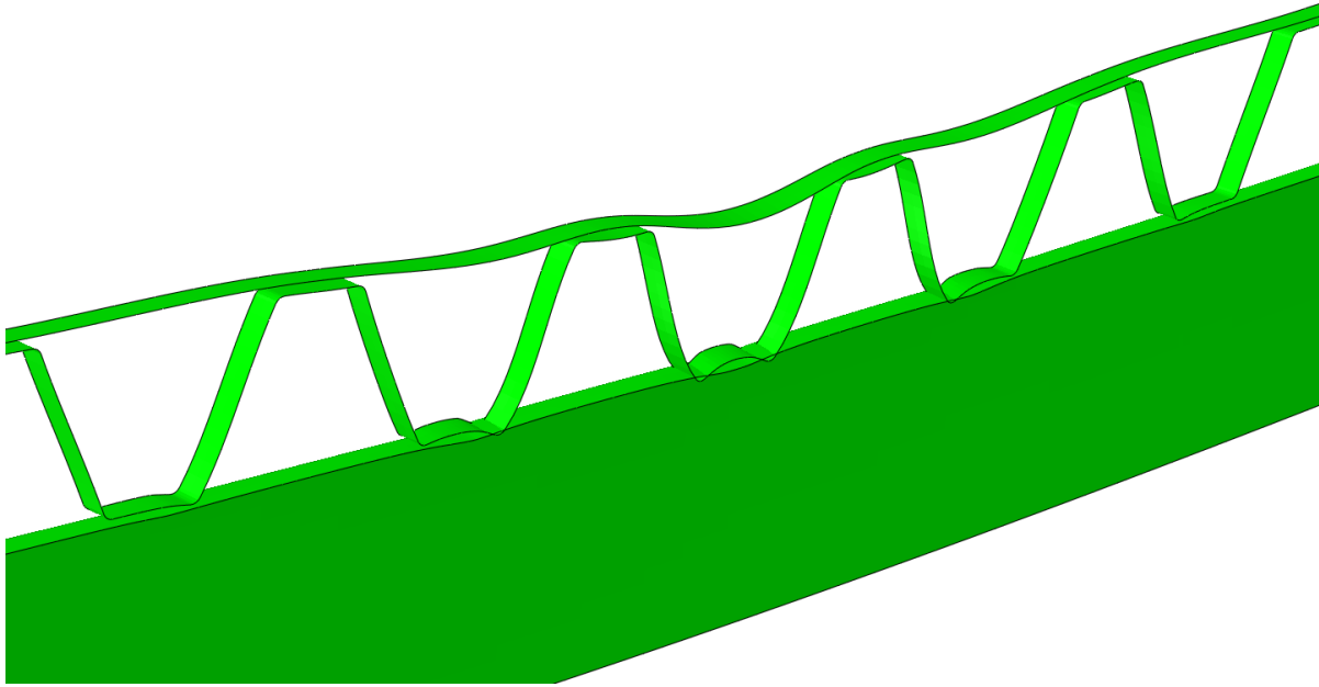
Figure 57. Deformed shape at transverse girder, scale factor = 50.
