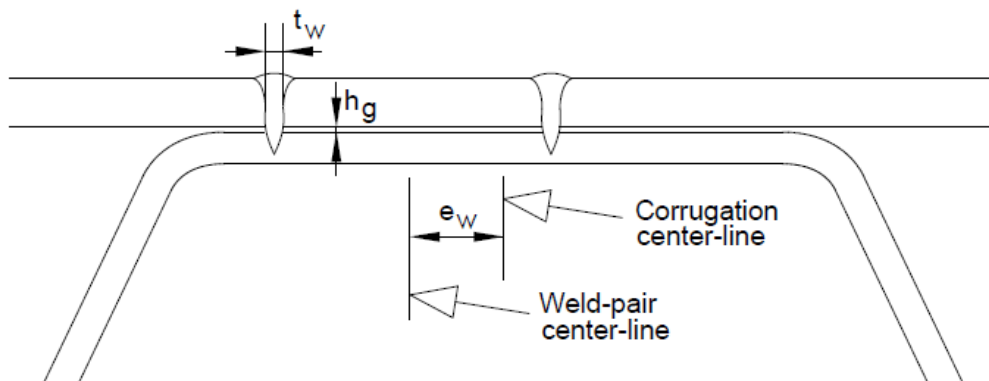
Figure 12. Joint region production-dependent geometric properties [Paper I].
