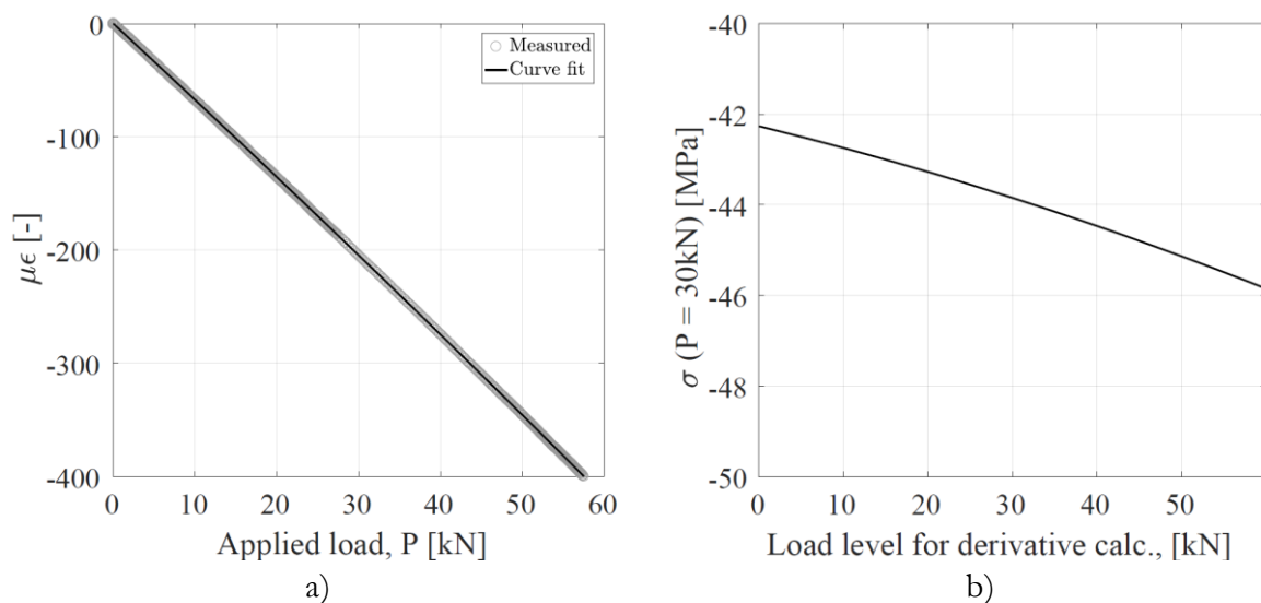
Figure 36. a) Measured micro-strain as a function of applied load and curve-fitted function, b) final stress at a load level of 30kN as a function of the load-level for the derivative calculation.
