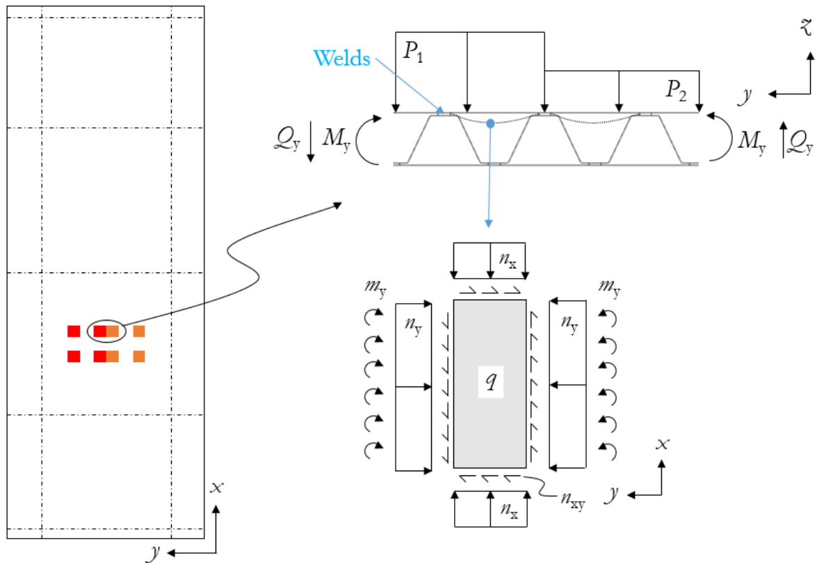
Figure 54. Load situation for Region ii .
