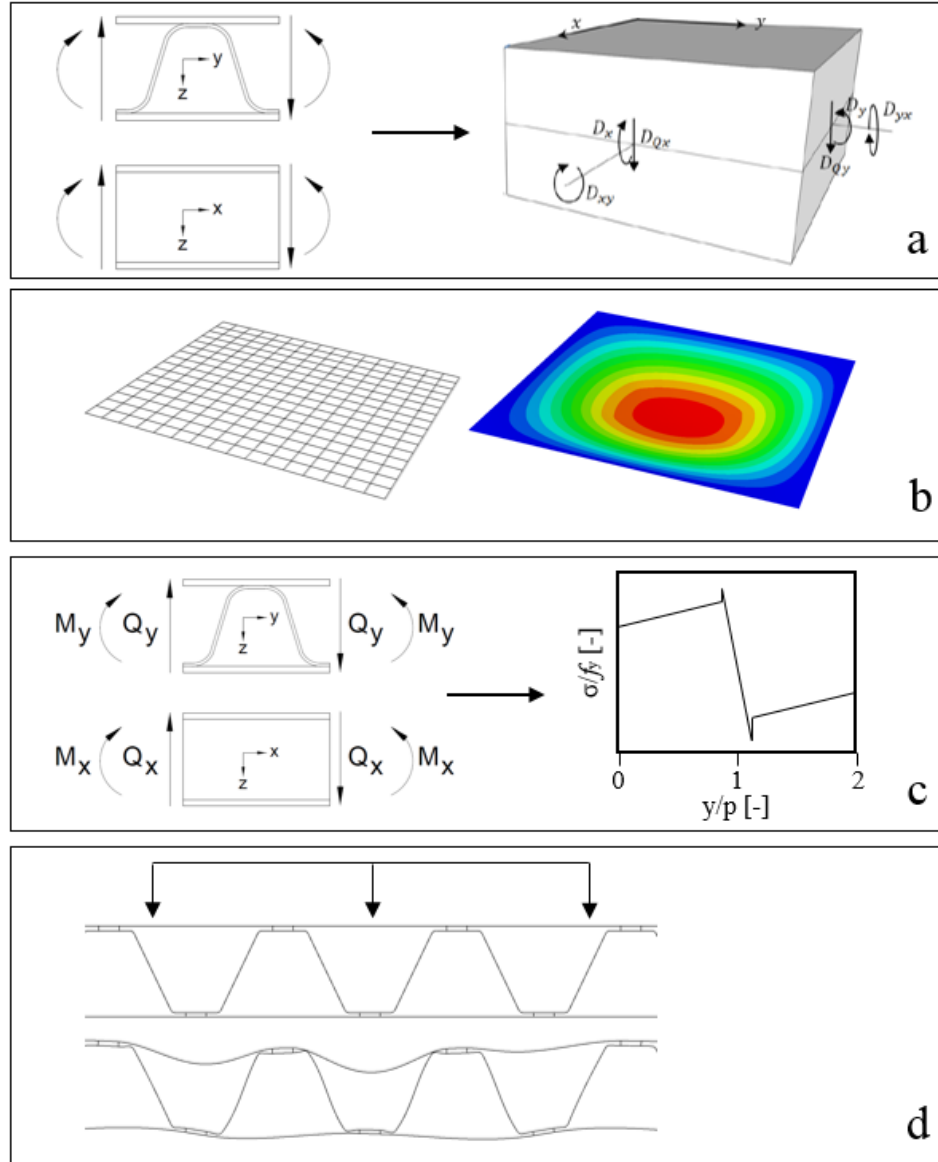
Figure 24. Schematic view of the ESL approach; a) derivation of equivalent stiffness properties, b) analysis of ESL, c) panel-level sectional forces causing local plate deformations yielding stress distribution in the constituent members of the cross section, and d) effect of directly applied loads (DAL) [Paper III].
