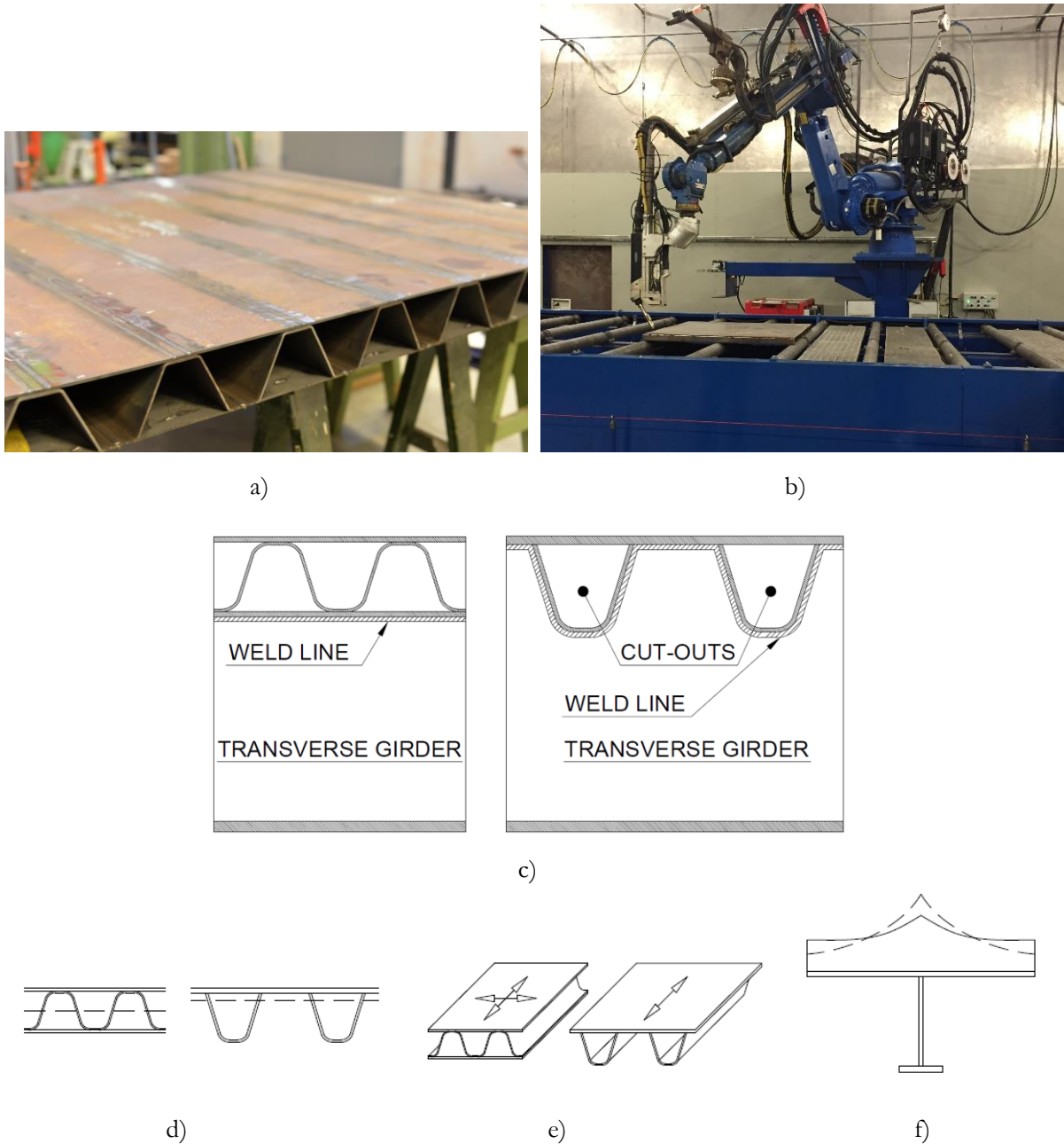
Figure 5. a) Laser-welded corrugated core steel sandwich panel, Nilsson et al. [40], b) laser-welding equipment, photo: Kleven Verft AS, c) comparison of deck to transvers girder connection between all-steel sandwich panel (left) and conventional stiffened plate (right) [13] d) increased bending-stiffness in the main direction, e) increased 2-way load distribution f) shear-lag comparison (dashed = conventional, solid = sandwich panel).
