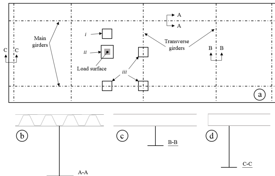
Figure 40. Investigated regions; i ) area subjected to panel-level sectional forces alone, ii ) loaded region and iii ) at connection to supporting structure. a) View from above, b) section at main girder, c) section at intermediate cross-beam and d) section at end cross-beam [Paper III].
