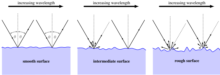
Figure 2.2: Impact of increasing surface roughness on surface scattering at different frequencies.
