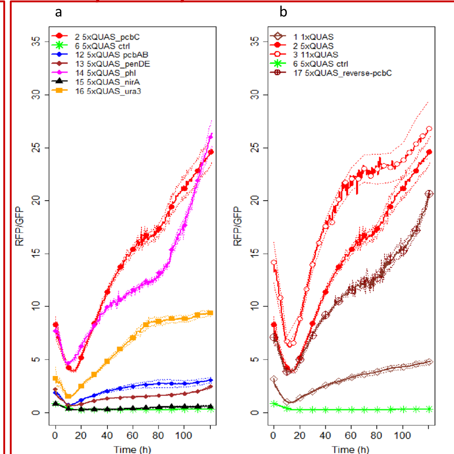
Fig.4. Development of DsRed/GFP fluorescence over time during growth of P. chrysogenum strains (a) Effect of different CPs driving DsRed with 5xQUAS. (b) Strains expressing DsRed under a synthetic promoter containing 0, 1, 5 or 11 QUAS elements upstream the pcbC CP.
