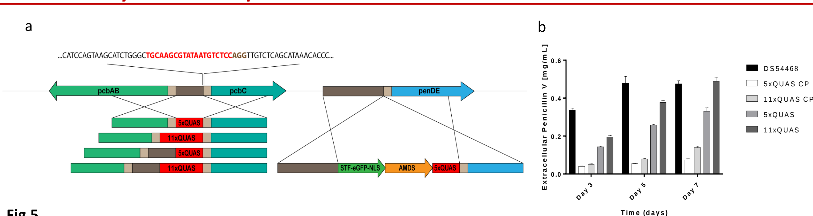
Fig.5. (a) Schematic representation of CRISPR/Cas9 based integration and co-transformation of the synthetic control device and QUAS elements into the penicillin cluster of DS54468. Designed sgRNA targets boundary between the promoter of pcbAB and the core promoter of pcbC . (b) Extracellular Penicillin V production of strains where the penicillin biosynthesis cluster is under control of the control device and parental strain DS54468 in shake flask cultivation in penicillin producing medium. Data shows 3 independent cultures, measured in replicates.
