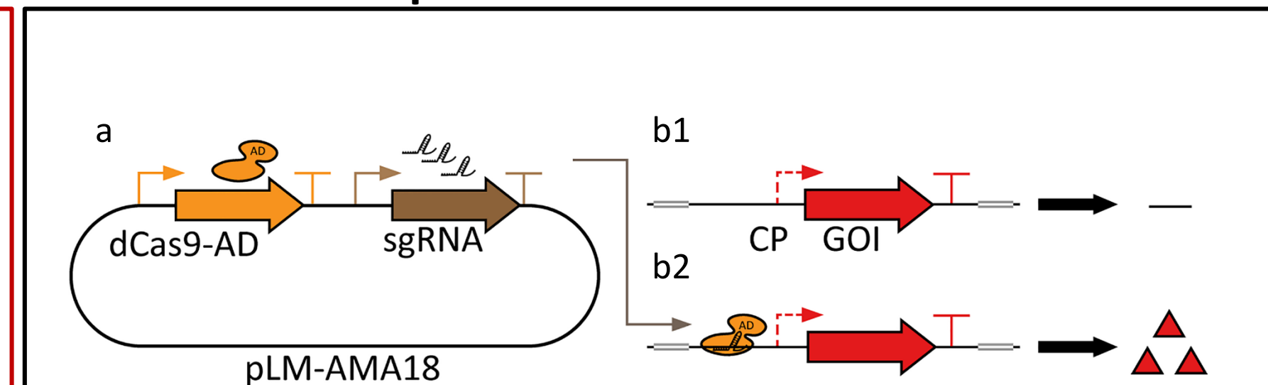
Fig.6. (a) Schematic representation of plasmid delivery of the CRISPRa components (dCas9m4-AD and sgRNA) where AD stands for transcriptional activator domain. (b1) Representation of synthetic silent promoter: no transcription from the gene of interest (GOI) without the integrated QUAS sequences (Figure 1). (b2) sgRNA guided dCas9-AD binding upstream the synthetic silent promoter, promoting transcriptional activation.
