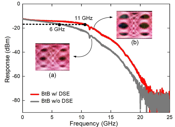
Fig. 5. Measured frequency response of a 10 Gb/s DML and APD based system at BtB with and without DSE. Inset: Optical eye-diagram of 25 Gb/s PAM-4 signal. (a) without DSE. (b) with DSE.
