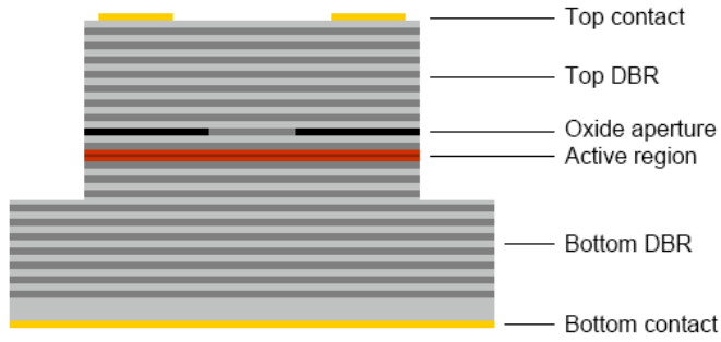
Figure 2.5: Oxide-confined VCSEL.
