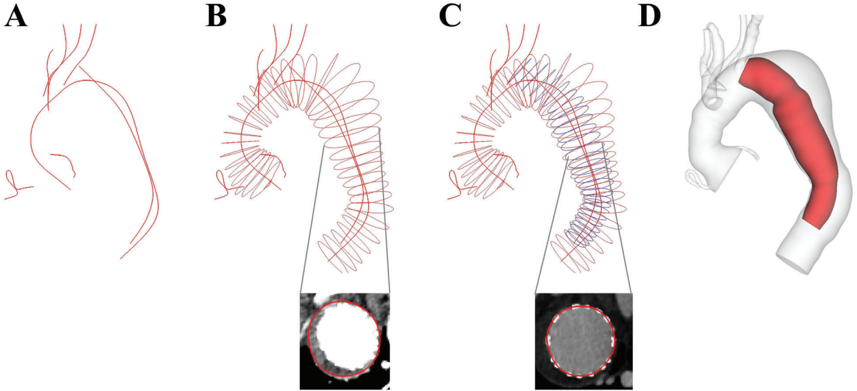
Figure 2.1: Figure presenting an overview of the steps used in the semi-manual modeling tool SimVascular. A shows 3D centerlines for a thoracic aorta, relevant branches and an endograft in the descending segment. B and C show 2D cross sections of the thoracic aorta and endograft, with examples from modeling of respective cross sections. D shows a rendering of lofted surfaces based on contours (intraluminal aortic surface in light grey, and endograft surface in red). Figure is taken from [6].
