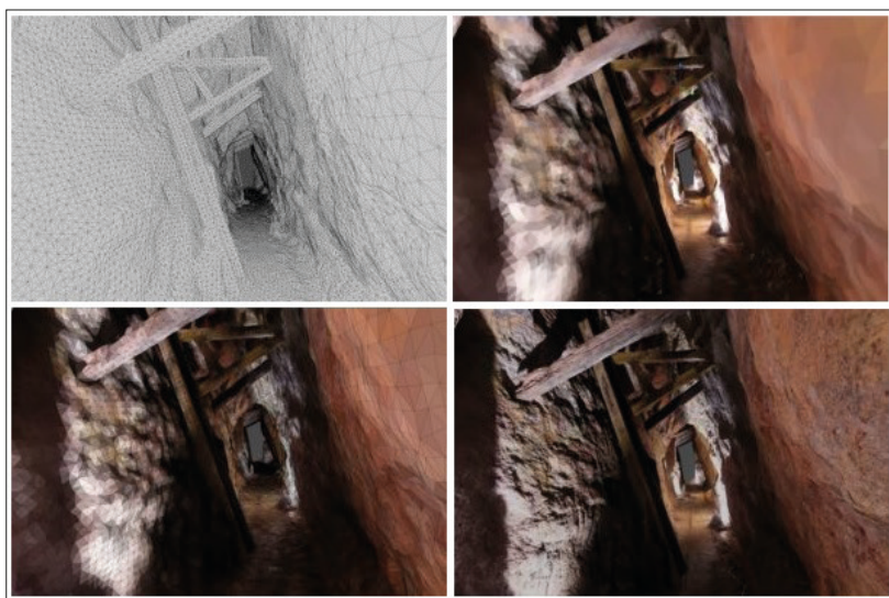
Figure 3. Stages of rendering a 3D model of a tin mine tunnel. Source: EESAB.
