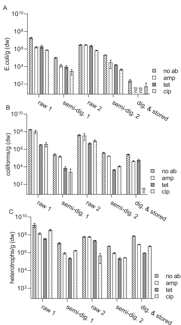
Fig. 2. Average CFUs/g sludge (dw) of presumptive E. coli (A), other coliforms (B) and heterotrophs (C) on plates without antibiotics or supplemented with ampicillin 8 \mu\text{g}/\text{ml} (amp), tetracycline 8 \mu\text{g}/\text{ml} (tet) or ciprofloxacin 0.5 \mu\text{g}/\text{ml} (cip). Raw and semi-digested sludge were sampled on two occasions (grab samples) and the digested and long-term stored sludge was sampled on the same day it was spread on fields by mixing several sub-samples. Error bars represent the standard deviation of three technical replicates. nd- no colonies detected.
