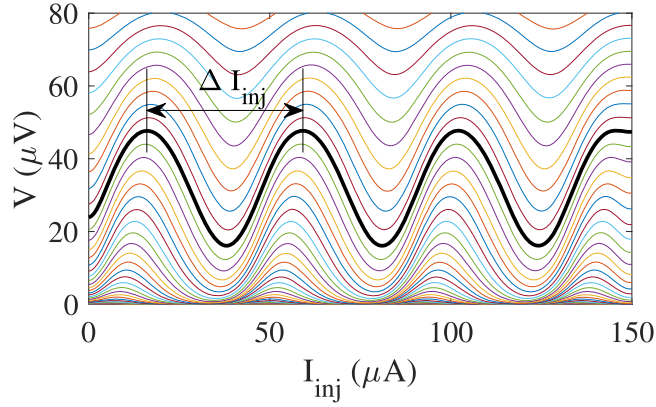
Figure 4. SQUID voltage V as a function of injected current I_{inj} (effectively flux bias) for different bias currents. The curve with the highest voltage modulation amplitude \Delta V is marked in black. The voltage modulation period \Delta I_{inj} is used to extract the coupling inductance L_c .
