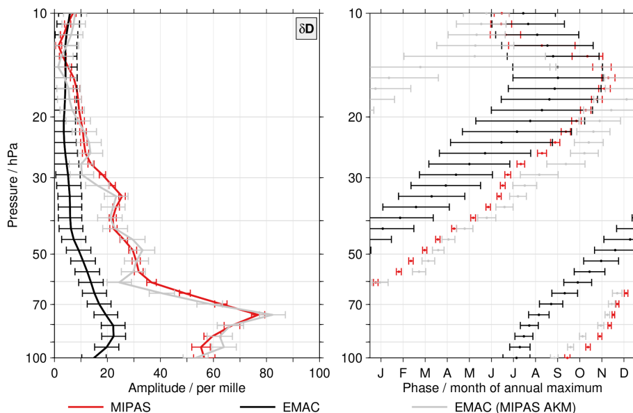
Figure 14. As for Figs. 3 and 4 but here focusing on EMAC results. For the original EMAC data, the results are shown in black; the results based on the convolution with the MIPAS averaging kernels are presented in grey. The original MIPAS results are shown in red.
