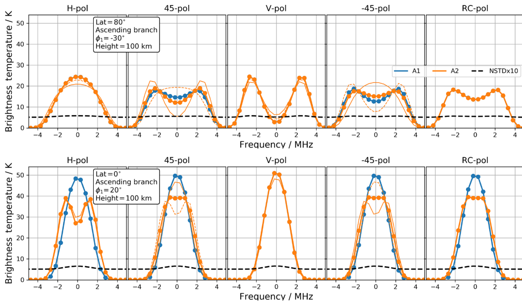
Figure 5. Upper panels: O_2 lines simulated for antenna-1 (blue) and antenna-2 (yellow) at 80^\circ N over the ascending orbit. Panels from left to right show the results for a detector with horizontal, +45^\circ , vertical, -45^\circ and right-circular polarization. The dashed and full yellow thin lines are spectra calculated with an angular tilt of the antenna-2 detector of -20 and +20^\circ . The black dashed lines are the measurement noise STD \times 10 for antenna-1. Lower panels: same as upper panels but for the Equator.
