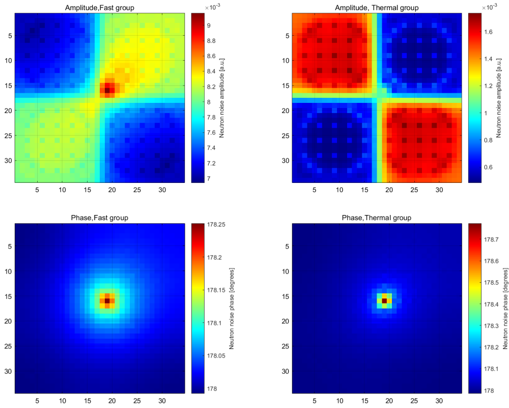
Figure 4.5 Neutron noise obtained from the DSA solver for the C3 case; fast (top-left) and thermal (top-right) amplitude and fast (bottom-left) and thermal (bottom-right) phase
