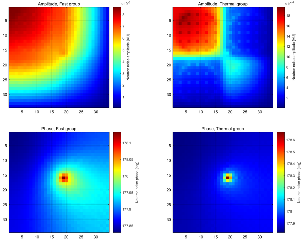
Figure 4.6 Neutron noise obtained from the DSA solver for the C4V case; fast (top-left) and thermal (top-right) amplitude and fast (bottom-left) and thermal (bottom-right) phase
