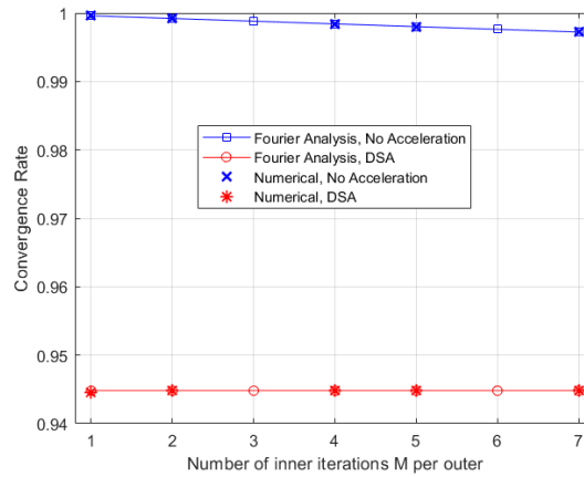
Figure 4.2 Convergence rate as a function of the number of inner iterations M for the accelerated and DSA schemes
