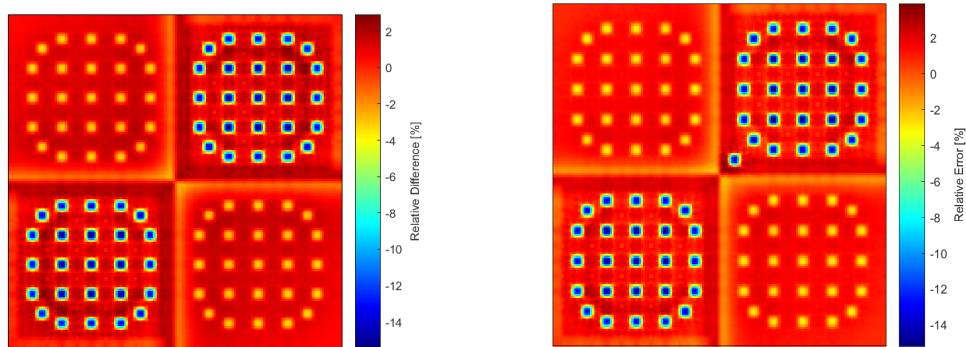
Figure 4.8 Spatial distribution of the relative differences between the two simulators, in the thermal neutron static flux (left) and in the thermal neutron noise (right)
