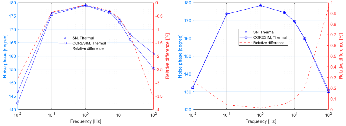
Figure 4.10 Phase of the thermal neutron noise calculated with the two solvers and relative differences, at the location of the neutron noise source (left) and at the location (17,18) (right)
