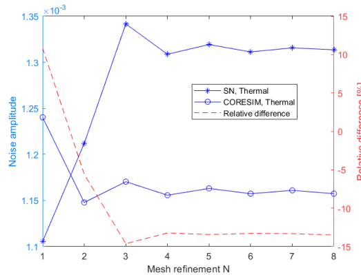
Figure 4.7 Effect of the spatial grid resolution on the amplitude of the thermal neutron noise at the location of the noise source
