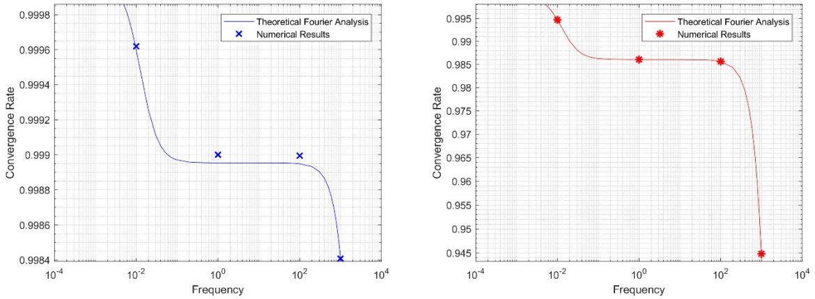
Figure 4.3 Convergence rate as a function of frequency for the unaccelerated scheme (left) and for the DSA scheme (right)
