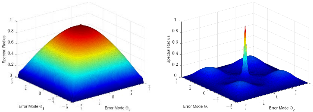
Figure 4.1 Theoretical spectral radius associated with the unaccelerated scheme (left) and the DSA scheme (right), for a neutron noise calculation in a 2-D homogeneous system.
