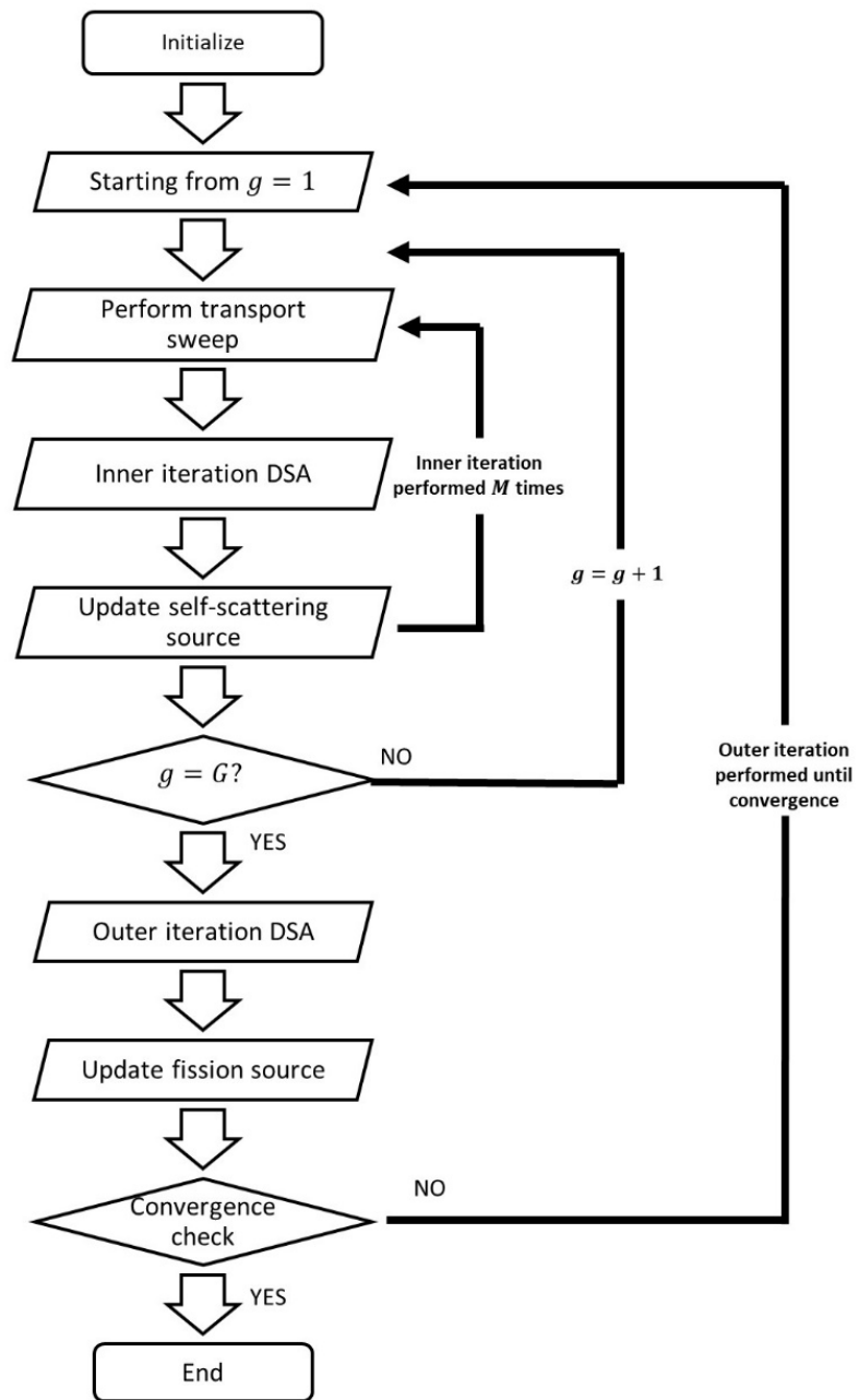
Figure 3.3 The DSA-based scheme for both static and dynamic module of the simulator
