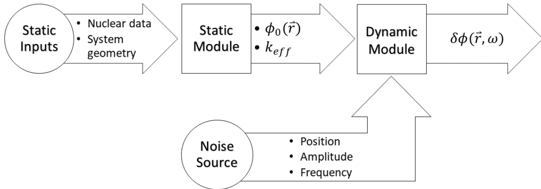
Figure 3.1 Overall calculation scheme of the discrete ordinates solver
