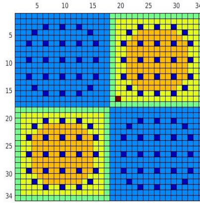
Figure 4.4 System configuration of C3 and C4V benchmark problems with the neutron noise source location labelled in red.
