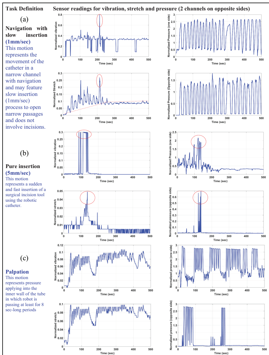
Figure 11. Sensor outputs from vibration, stretch and two pressure channels located at the opposing sides of the endoscope for (a) navigation featuring a slow insertion, (b) pure insertion and (c) palpation.
