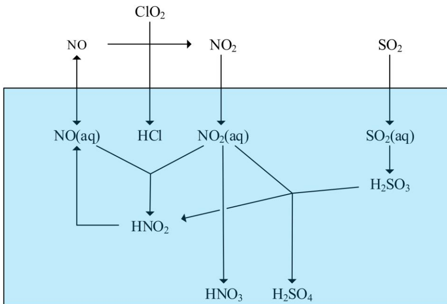
Figure 4: Schematic overview of the chemistry used to describe the simultaneous absorption of NO x and SO x after enhanced NO oxidation to NO 2 using ClO 2 .
