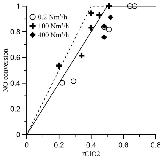
Figure 12: NO conversion rate versus r_{\text{ClO}_2} (as defined by (4.2) and (4.1) respectively). Comparisons of the 0.2 Nm 3 /h, 100 Nm 3 /h and 400 Nm 3 /h scales. The solid line shows the theoretical NO conversion rate given a stoichiometry of 0.5 for the ClO 2 and NO ratio (Reactions 1 and 2). The dashed line indicates the maximum theoretical conversion rate (Reaction 3). The results for the 0.2 Nm 3 /h setup correspond to those shown in Figure 10 c).
