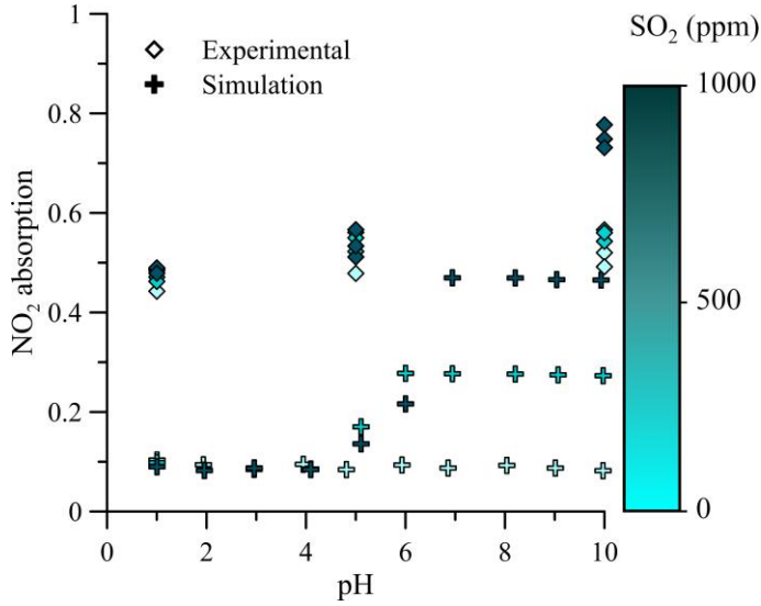
Figure 16: Comparison of the modeling and experimental results presented in Figure 14 for the 0.2 Nm 3 /h setup. The three inlet concentrations of SO 2 are: 0 ppm, 200 ppm, and 1,000 ppm. NO 2 absorption is defined by (4.4).
