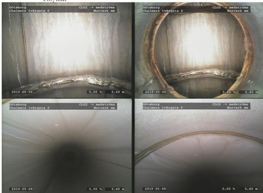
Figure 13: Photographs acquired during the inspection of the oxidation reactor of the 100 Nm 3 /h setup, together with color-coded legend. Upper-left panel (green): Pipe wall and welding joint at the start of the pipe expansion from 10-cm to 20-cm diameter. A zoomed view of the upper-right image. Upper-right panel (pink): Pipe wall and welding joint at the start of the pipe expansion, as well as the welding joint for the pipe surrounding the ClO 2 injection nozzle (5-cm diameter). Lower-left panel (yellow): Expanded section of the oxidation reactor. Lower-right panel (blue): Welding joint at the end of the pipe expansion.
