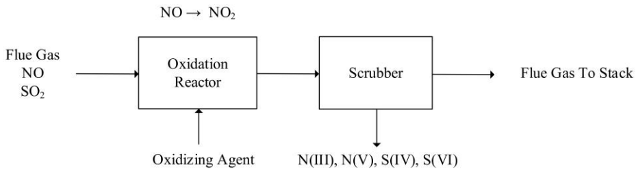
Figure 3: Overview of the discussed concept for simultaneous removal of \text{NO}_x and \text{SO}_x from flue gases in a process that employs enhanced oxidation of \text{NO} .
