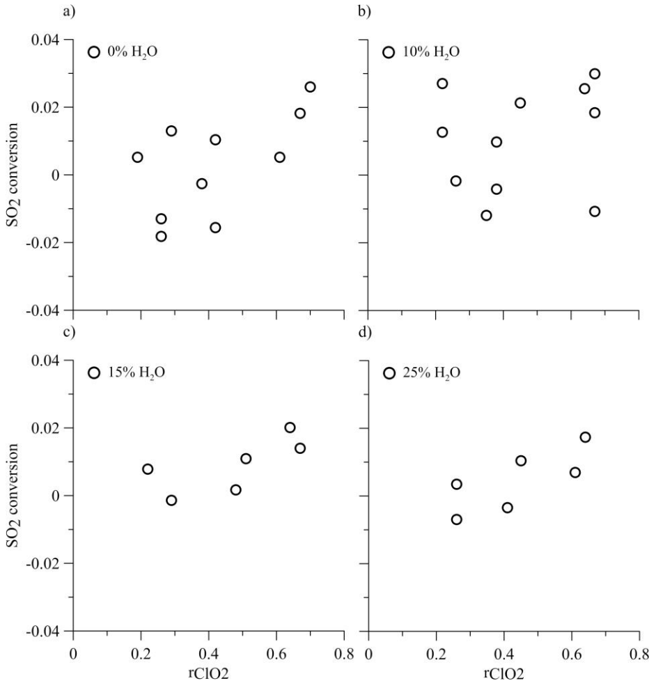
Figure 11: Measured rates of SO 2 conversion (as defined by (4.6)) between experiments with and without ClO 2 injection at different humidity levels: (a) 0% H 2 O; (b) 10% H 2 O; (c) 15% H 2 O; and (d) 25% H 2 O at the inlet. The experimental conditions were according to Table 1.
