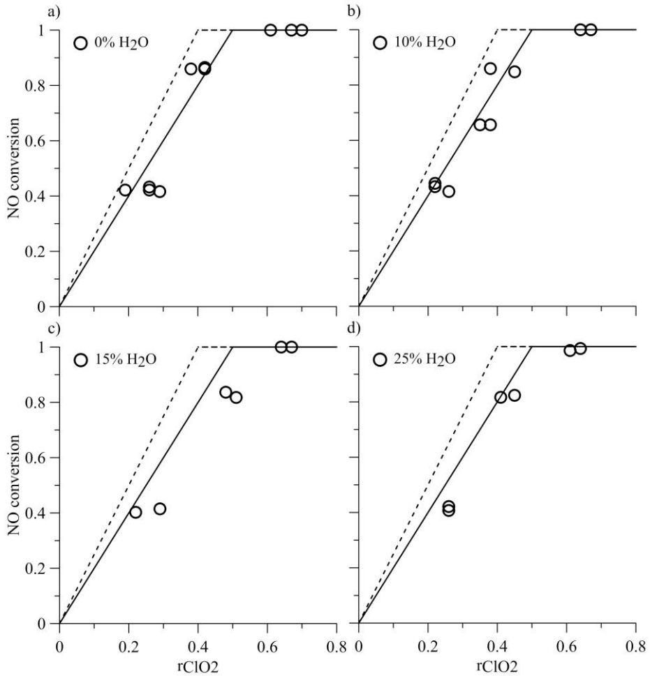
Figure 10: Conversion of NO (as defined by (4.2)) after ClO_2 injection at the humidity levels: (a) 0% H_2O ; (b) 10% H_2O ; (c) 15% H_2O ; and (d) 25% H_2O at the inlet. Measurements are indicated by circles, and the theoretical dry-basis conversion rate is shown with a solid line in each panel. The theoretical wet-basis conversion is indicated with a dashed line in each panel. Experimental conditions were according to Table 1.
