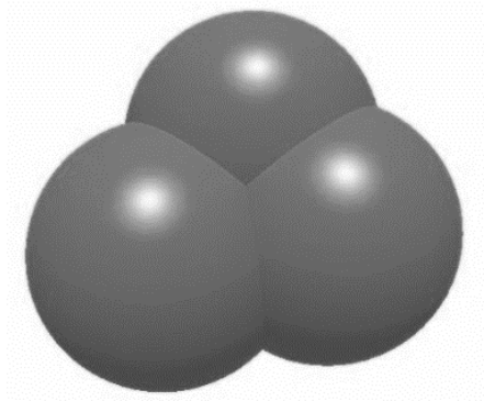
Figure 3. Three spheres particle used in simulations.
