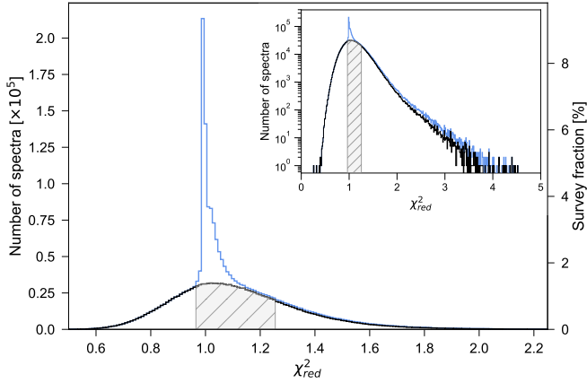
Fig. B.4. Histogram of \chi_{\text{red}}^2 values for all GRS spectra (blue) and GRS spectra with at least one fit component (black). The inset shows the same distribution on a logarithmic scale. The grey-shaded area marks the IQR for the distribution of spectra with fitted components, ranging from about 0.96–1.25. The bin width is 0.01.
