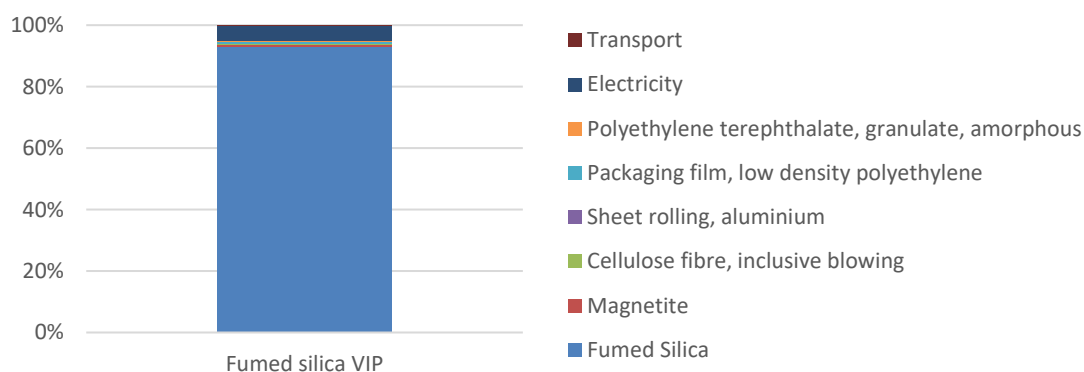
Figure 8. The result of the composition analysis of cradle-to-gate LCIA of fumed silica VIP in GWP IPCC2013 100a (IPCC, 2013)
