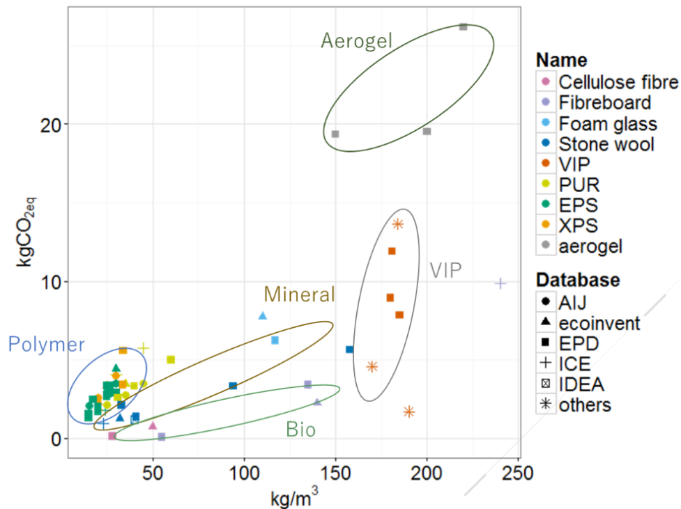
Figure 2. The mapping of GHG-emissions from various insulation materials with aligned thermal performance (identical thermal resistance ( 1 \text{ m}^2\text{K/W} )) ( n=57 )
