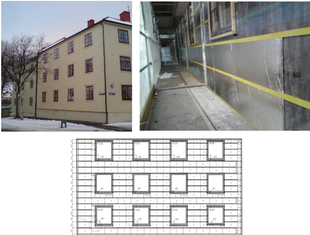
Figure 3-16: 1930s building in Gothenburg with VIPs (Photo: Pär Johansson).
