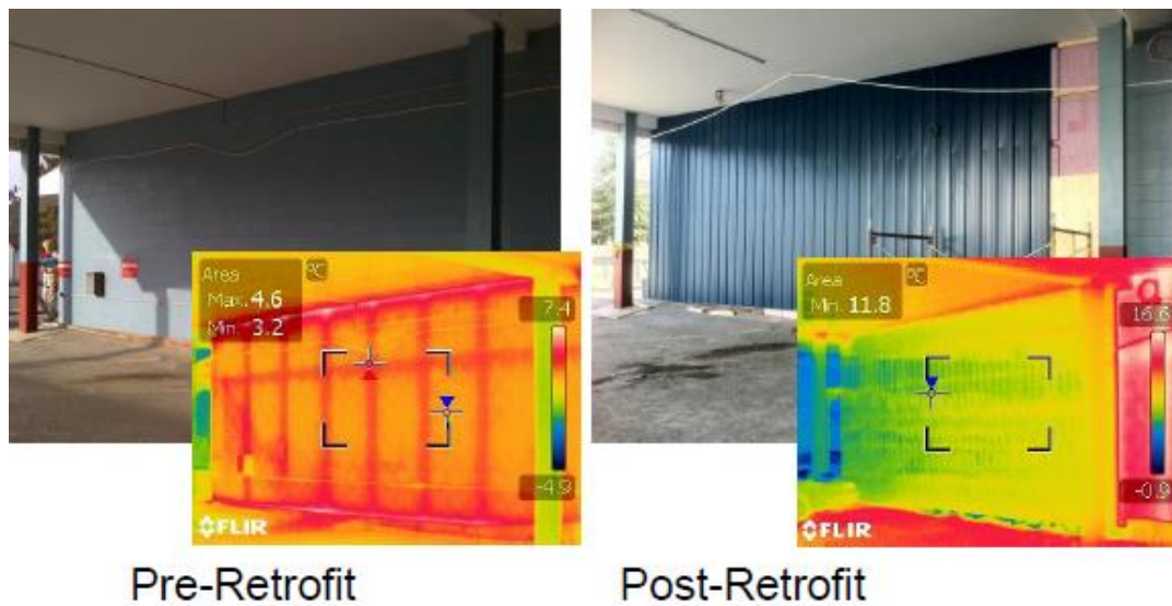
Figure 3-19: Infrared image of the retrofitted wall [68].
