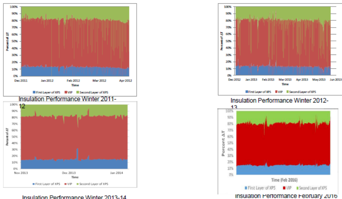
Figure 3-26: Insulation performance in the retrofitted wall in 2011-2016 [68].
