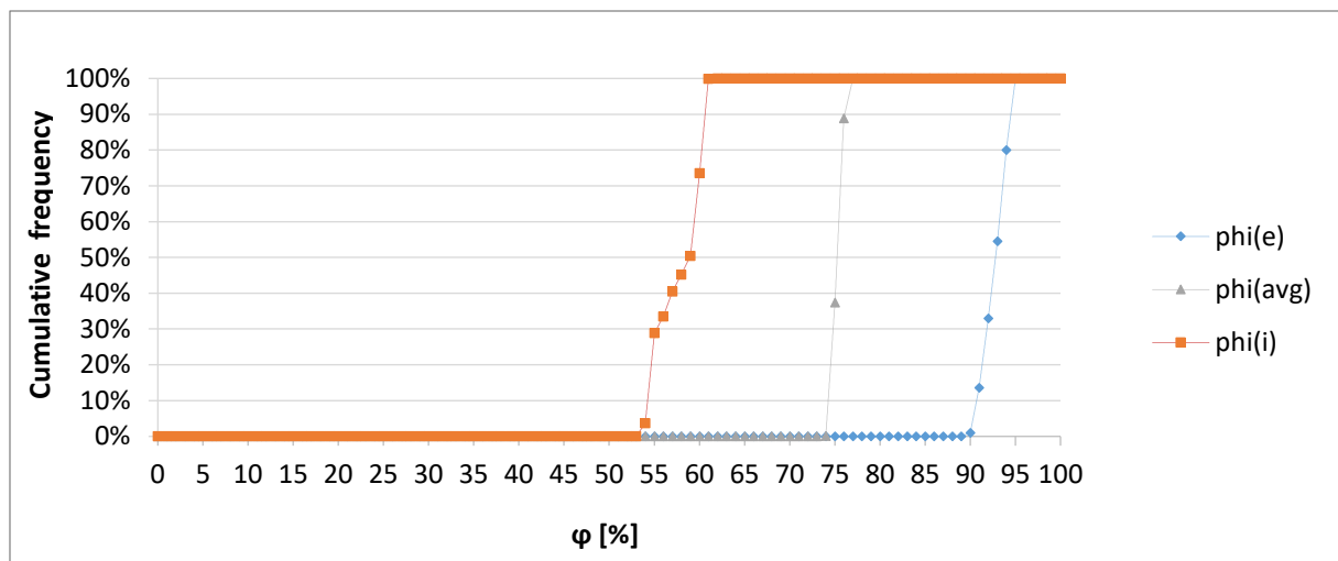
Figure -56. Relative humidity cumulative functions for Configuration C6-HO-NM-SO.
