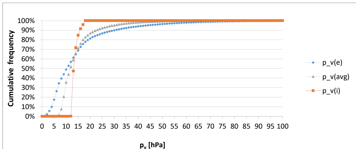
Figure -57. Water vapour pressure cumulative functions for Configuration C6-HO-NM-SO.
