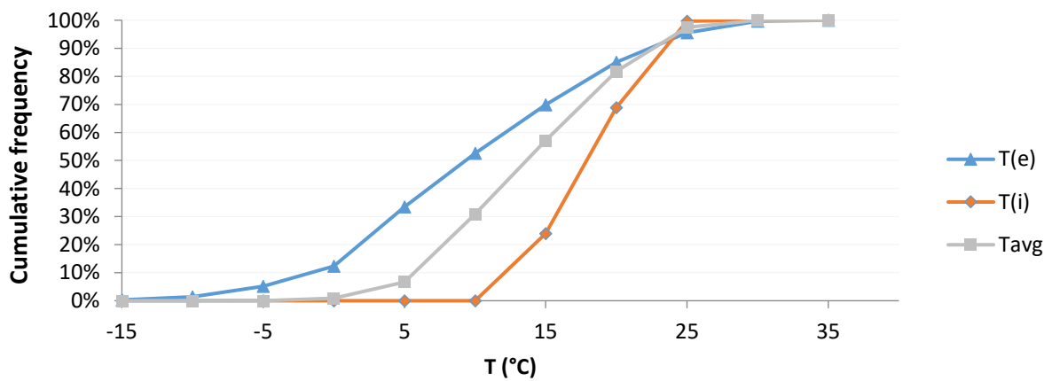
Figure 35. Temperature cumulative functions for the inside and outside of the VIP panel for the façade towards North.
