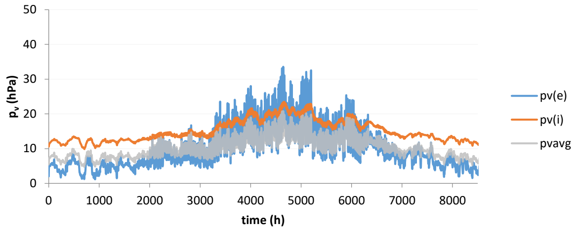
Figure 34. Yearly time profile of vapour pressure on the inside and outside of the VIP panel for the façade towards North.
