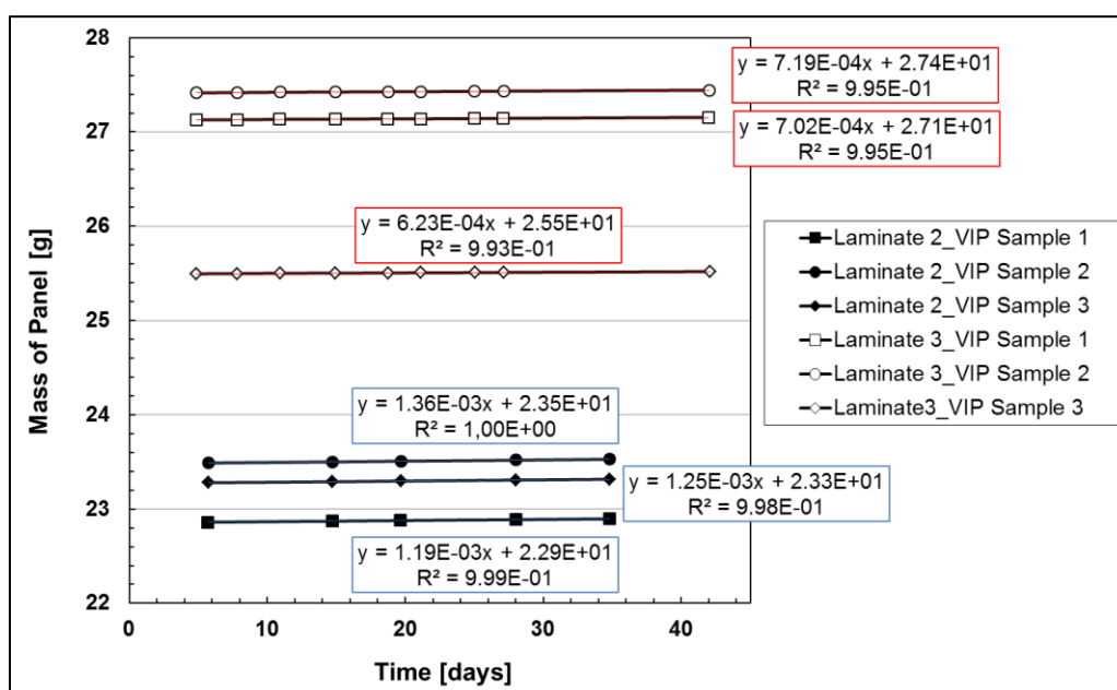
Figure 78: Water intake tests for the VIPs prepared using Laminate-2 and Laminate-3 as VIP envelope, measured at 40^\circ\text{C} and 90% RH by Lab-2.
