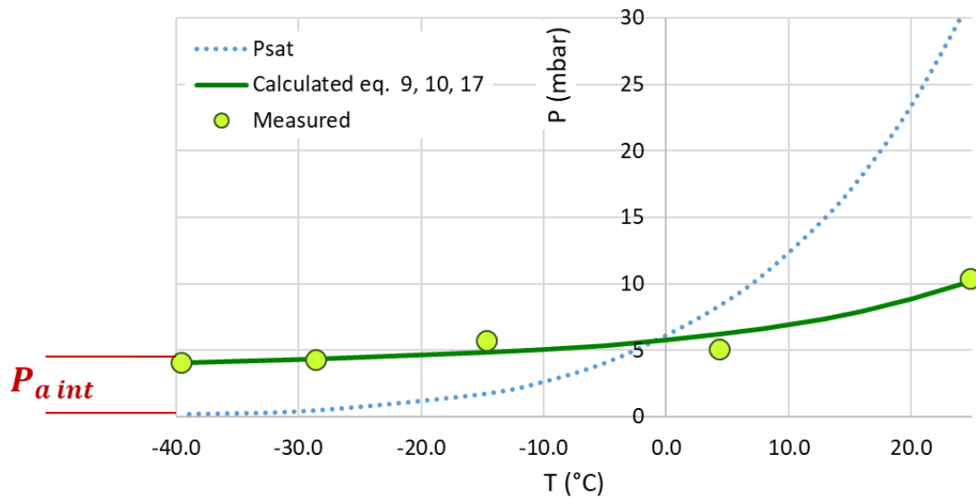
Figure 76: Example of the multiple measurements option of the cold lift-off method, comparison between matched calculation and measurements
