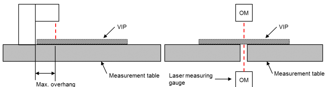
Figure 134: Left: standard equipment for thickness determination with limited possibilities to measure the thickness in the measurement area; right: alternative setup of measurement equipment for thickness determination of VIP allowing a thickness determination on any position.
