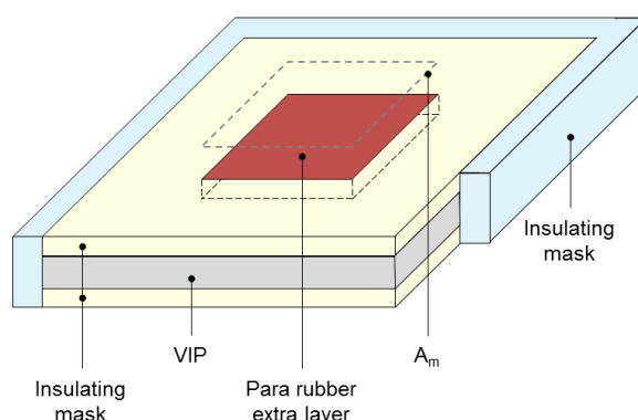
Figure 133: Adoption of thick rubber extra layer.
