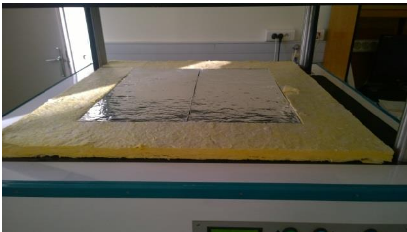
Figure 16: VIP in the heat flow meter apparatus with a guard of mineral wool around the specimen. Source: Centre Scientifique et Technique du Bâtiment.
