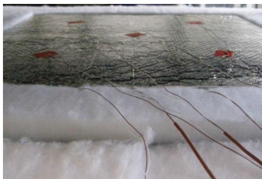
Figure 17: VIP in the heat flow meter apparatus with a guard of fibre based padding around the specimen (left) and mineral wool (right). The padding is thicker than the panel to ensure a proper insulation during measurement. Left: source: FIW München; right: source: KTH Royal Institute of Technology.
