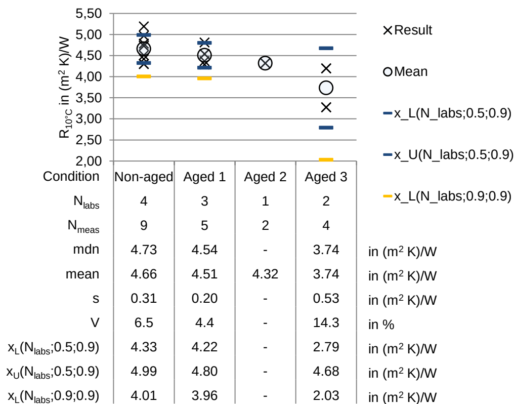
Figure 38: Results of thermal resistance ( R ) at 10^\circ\text{C} mean temperature in COP in (\text{m}^2 \text{K})/\text{W} for material VIP 1.
