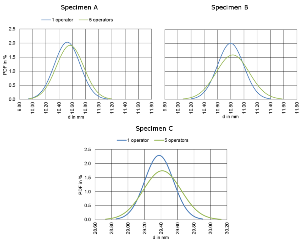
Figure 123: Comparison of Gaussian distributions between measures taken by one operator and five operators, measurement equipment 1 (ME 1), specimen A, specimen B, specimen C, 9 measuring points.
