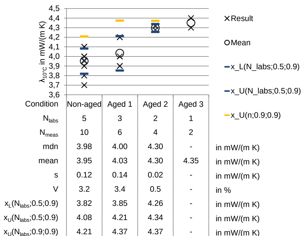
Figure 42: Results of thermal conductivity ( \lambda ) at 10°C mean temperature in COP in \text{W}/(\text{m K}) for material VIP 3.
