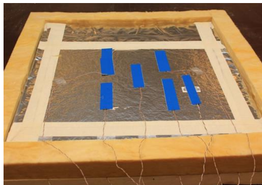
Figure 17: VIP in the heat flow meter apparatus with a guard of fibre based padding around the specimen (left) and mineral wool (right). The padding is thicker than the panel to ensure a proper insulation during measurement. Left: source: FIW München; right: source: KTH Royal Institute of Technology.
