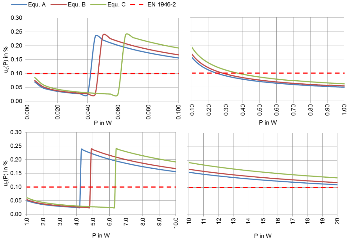
Figure 127: Combined uncertainty of the electrical power in between 0.005-20W assuming measurement uncertainty of voltage and current according to Table 60, top left: P = 0.005-0.100\text{W} ; top right: P = 0.10-1.0\text{W} ; bottom left: P = 1.0-10\text{W} ; bottom right: P = 10-20\text{W} .
