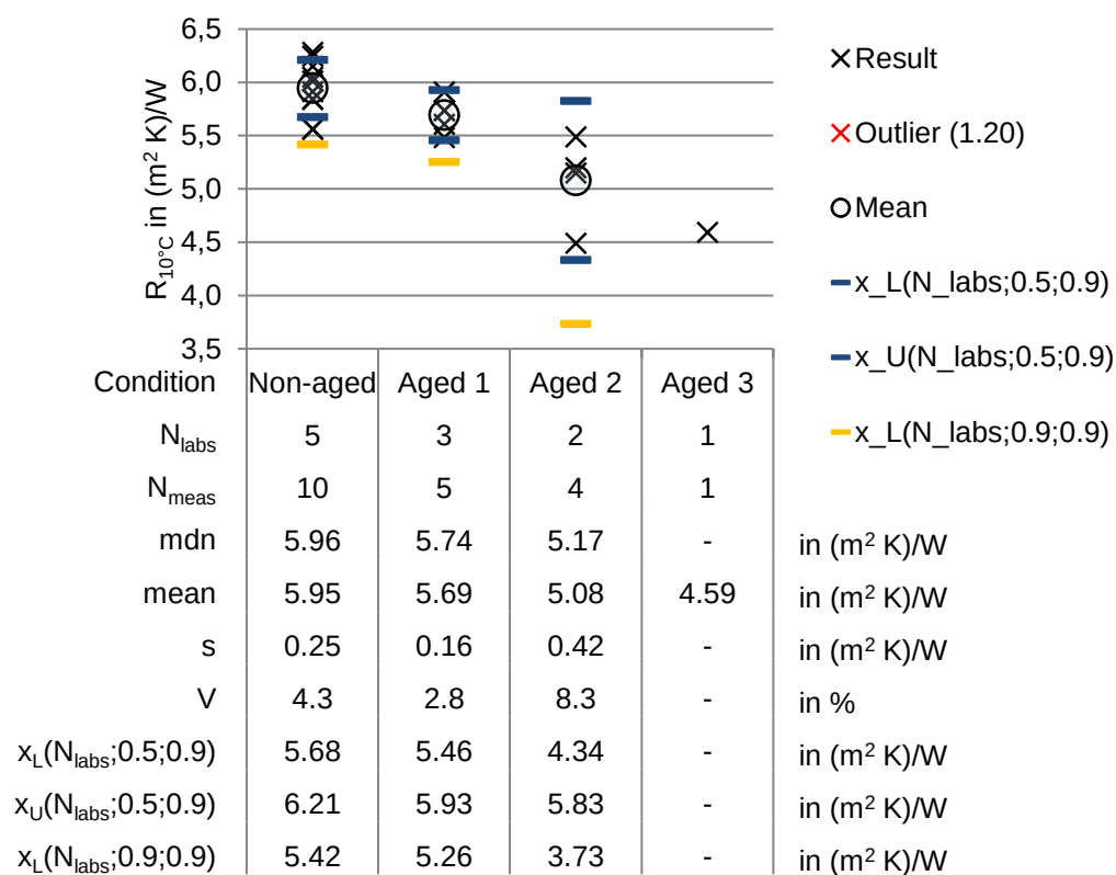
Figure 44: Results of thermal resistance ( R ) at 10°C mean temperature in COP in (m² K)/W for material VIP 4.
