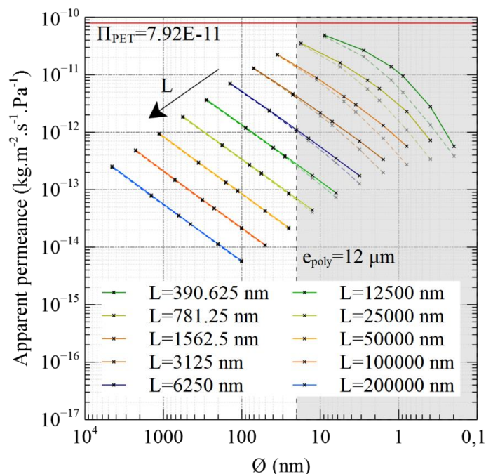
Figure 85: Calculated apparent permeance on PETM1F as a function of the defects size for 10 distances between defects. Source: EDF.
