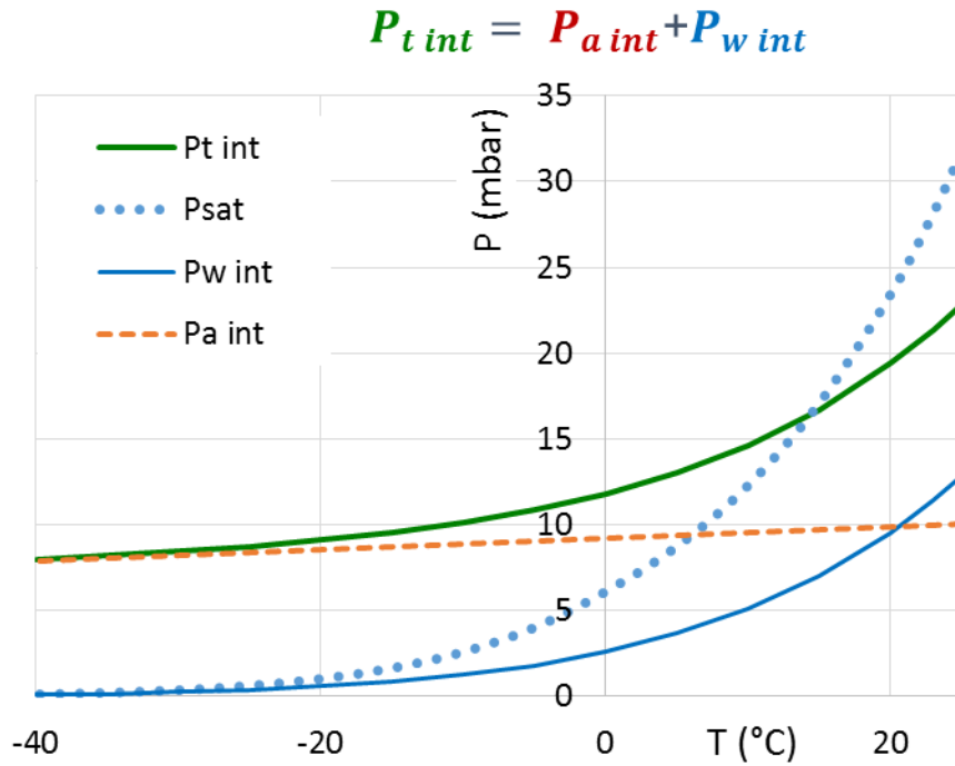
Figure 75: Schematic behaviour of the internal pressure as a function of the temperature for a VIP where the partial pressures at room temperature for air and water are respectively 10 and 12 mbar.
