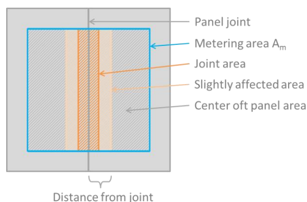
Figure 3: Highly affected (joint area), slightly affected and centre of panel area of two VIPs arranged for determination of \psi values. Source: FIW München.
