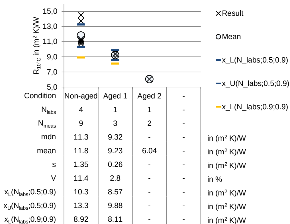
Figure 47: Results of thermal resistance ( R ) at 10^\circ\text{C} mean temperature in COP in \text{m}^2 \text{K}/\text{W} for material VIP 5.
