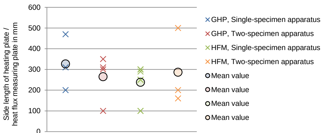
Figure 29: Side length of heating plate / heat flux measuring plate in mm of the apparatus for thermal conductivity measurement distinct to type of apparatus.
