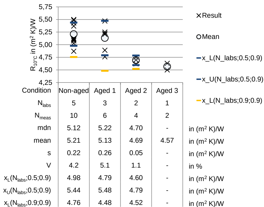
Figure 41: Results of thermal resistance ( R ) at 10^\circ\text{C} mean temperature in COP in \text{m}^2 \text{K}/\text{W} for material VIP 3.
