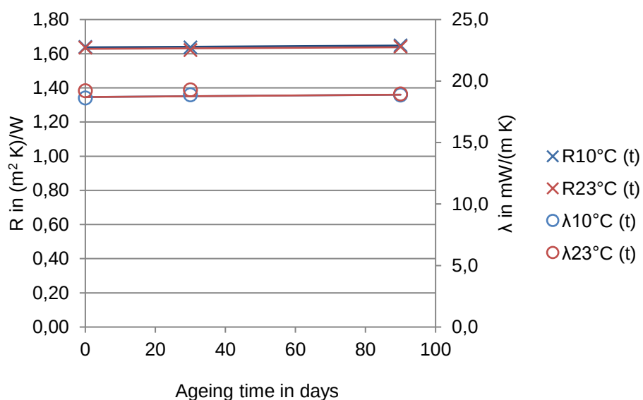
Figure 37: Results of thermal resistance ( R ) and thermal conductivity ( \lambda ) at 10°C and 23°C as a function of ageing time for material APM 2.
