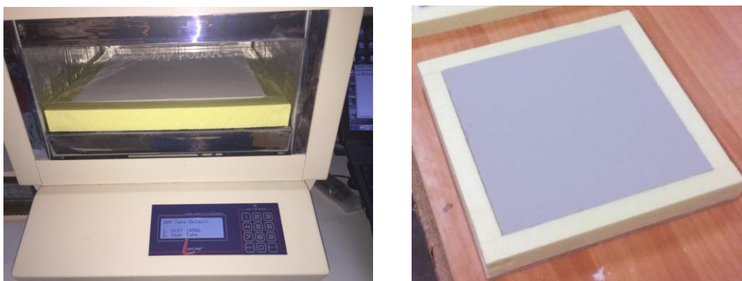
Figure 11: Rigid APM board installed in the heat flow meter apparatus with PU foam frame. Source: Università di Perugia.
