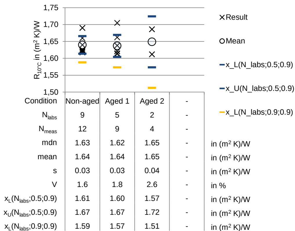
Figure 35: Results of thermal resistance ( R ) at 10^\circ\text{C} mean temperature in (\text{m}^2 \text{ K})/\text{W} for material APM 2.
