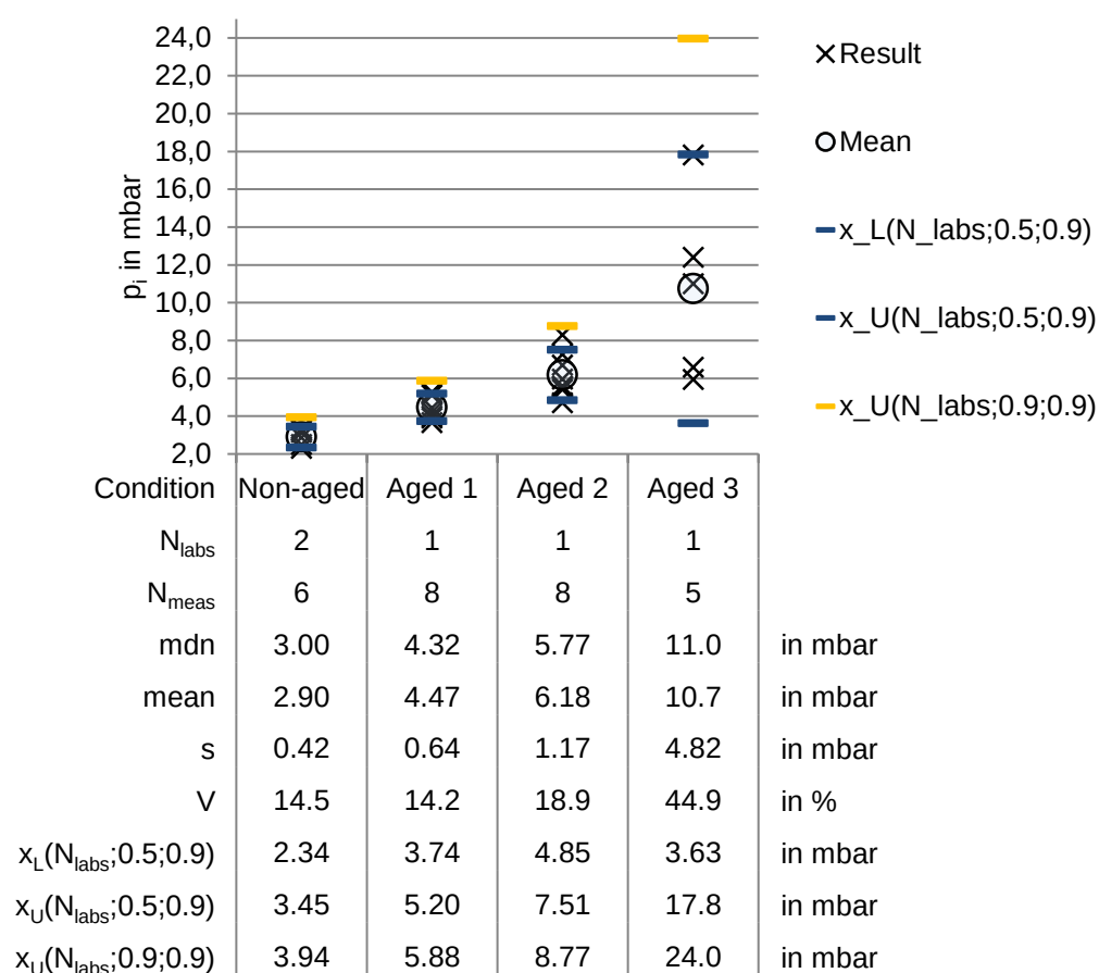
Figure 61: Results of internal pressure determination of material VIP 4.
