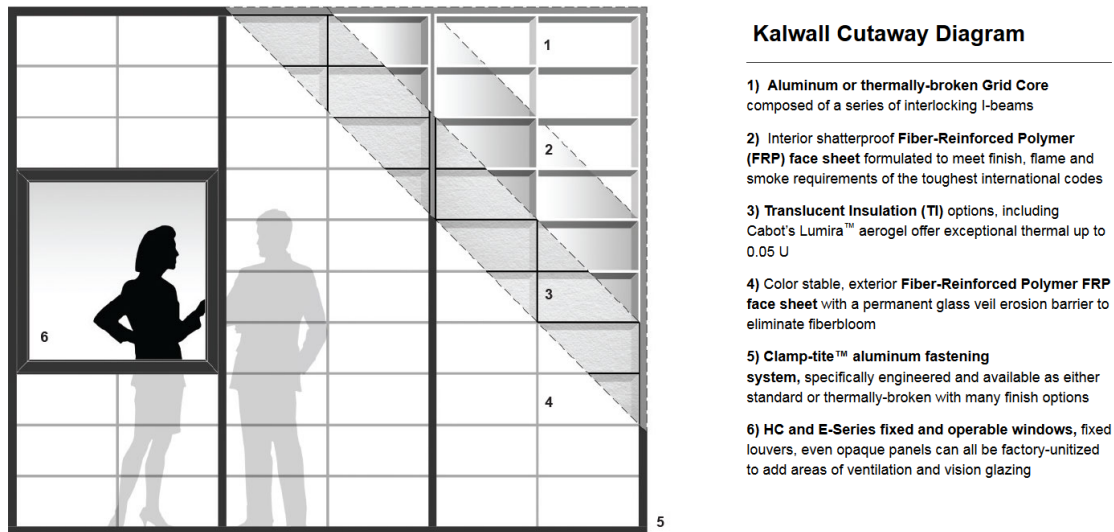
Figure 75: Kalwall translucent structural sandwich panel.
