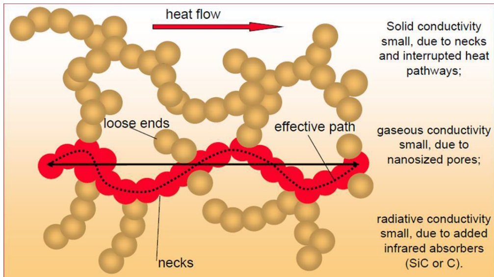
Figure 3: Sketch of the three heat transfer paths in nano-structured aerogels or fumed silica (Fricke, 2005).
