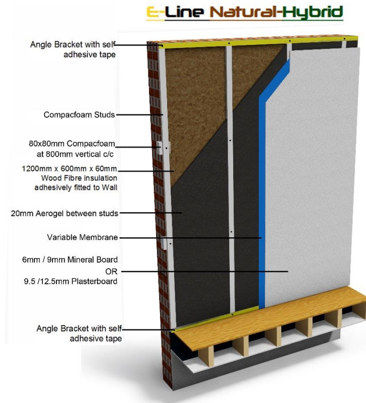
Figure 76: E-Line Natural Hybrid wall assembly.
