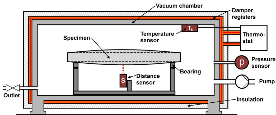
Figure 51: Principal sketch of the measurement device in a vacuum chamber - linear bearings, temperature and distance sensor (laser device) (illustration FIW).
