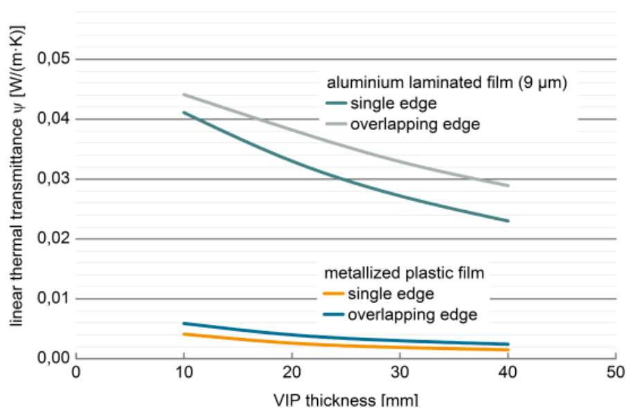
Figure 4: Comparison of linear thermal transmittance calculated for aluminium-laminated films (9 \mu\text{m} AL) and metallised plastics films (3 x 60 nm AL) for two edge designs (Sprengard & Holm, 2014).
