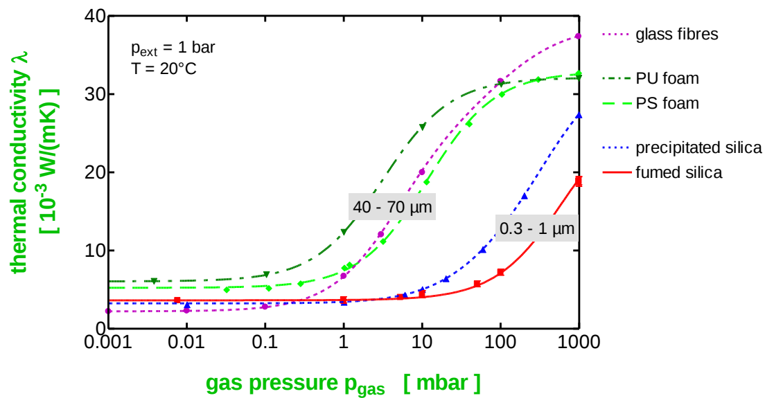
Figure 15: Thermal conductivity of different filler materials more or less optimised for the application in vacuum insulation panels. External pressure is 1 bar, the temperature 20^\circ\text{C} (Heinemann et al., 1999; Heinemann, 2008).
