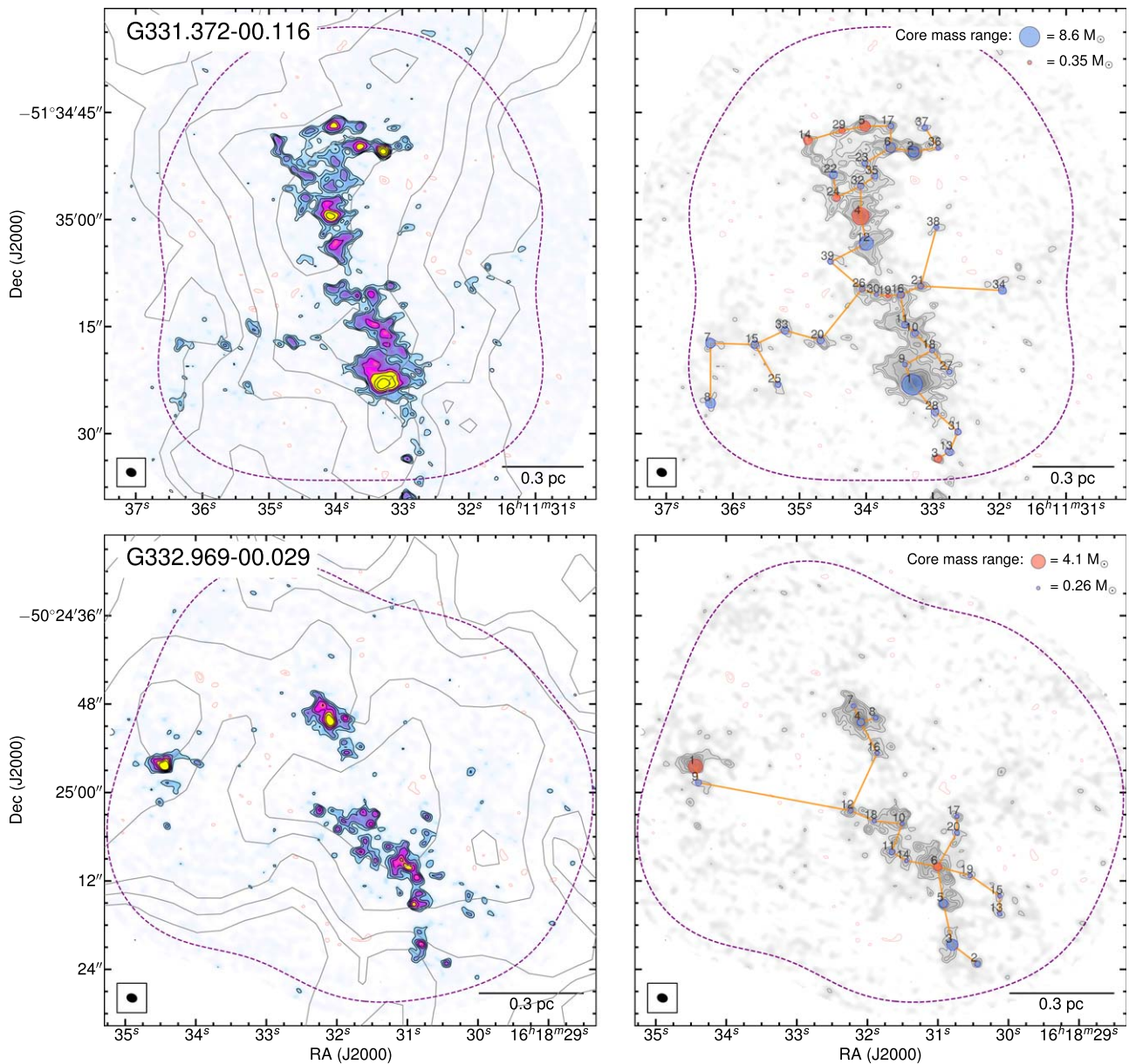
Figure 7. Same as in Figure 5, except for ALMA contour levels of -4 , -3 , 3 , 4 , 5 , 7 , 9 , 12 , and 16 \times \sigma , with \sigma = 0.083 mJy beam ^{-1} , for G331.372–00.116 ( 1'' angular resolution); and -4 , -3 , 3 , 4 , 5 , 6 , 7 , and 8 \times \sigma , with \sigma = 0.080 mJy beam ^{-1} , for G332.969–00.029 ( 1'' angular resolution).
