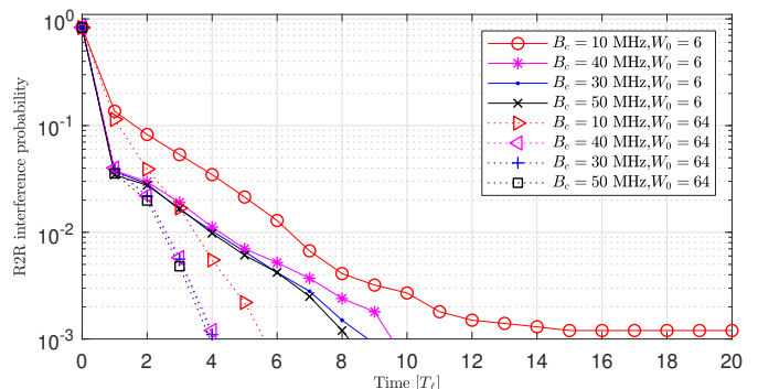
Fig. 15: R2R interference probability versus time for changing B_c and W_0 for M = 70 .
