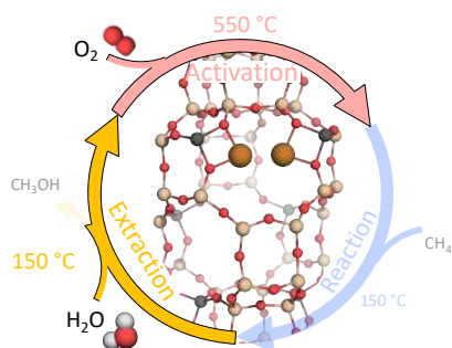
(a) Paper I: The stability of different Cu 2 -cluster structures are investigated in the context of direct methane-to-methanol conversion.
