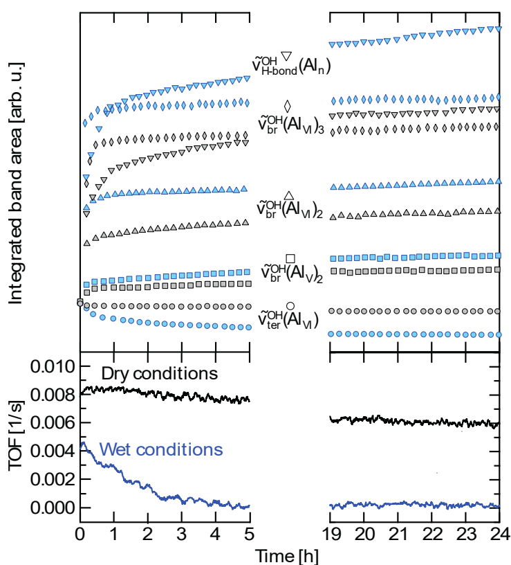
Figure 4.7: 24 h exposure of Pd/ \gamma -Al 2 O 3 -500 to dry (black) and wet (blue) methane oxidation conditions at 330 °C. Hydroxyl build-up is monitored in the top panel for the \tilde{\nu}_{\text{ter}}^{\text{OH}}(\text{Al}_{\text{VI}}) (○), \tilde{\nu}_{\text{br}}^{\text{OH}}(\text{Al}_{\text{V}})_2 (□), \tilde{\nu}_{\text{br}}^{\text{OH}}(\text{Al}_{\text{VI}})_2 (△), \tilde{\nu}_{\text{br}}^{\text{OH}}(\text{Al}_{\text{VI}})_3 (◇) and \tilde{\nu}_{\text{H-bond}}^{\text{OH}}(\text{Al}_n) (▽) absorption bands. Catalytic activity is monitored as methane TOF in the bottom panel.
