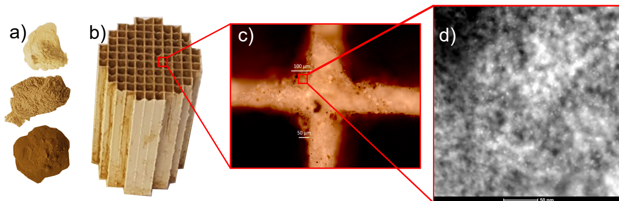
Figure 2.1: a) Pd/Al 2 O 3 powders samples with 0.25, 1 and 2 wt% palladium, b) a ceramic monolith substrate coated with Pd/Al 2 O 3 , c) optical microscopy image of the coated monolith cross-section, and d) electron microscopy image of a Pd/Al 2 O 3 washcoat used in reactor experiments.
