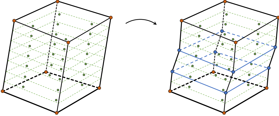
Figure 4.3: Example of how an unrefined element with seven plies, with one layer of integration points each (left), is subdivided into sublaminates when the element is refined in interface two and four (right). The bottom two plies will be associated with the bottom sublaminates, plies three and four with the second sublaminates and the top three with a third and topmost sublaminates. This particular example shows refinement enrichments via the AFEM, where the element base (vertex) nodes are indicated with orange and the extra nodes with blue.
