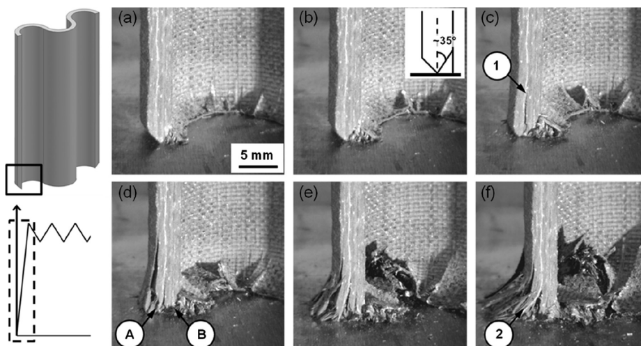
Figure 2.3: Example reproduced from [15] on crushing of laminated composites; including bending of plies (A), compressive failure (B), delamination in mode I (1) and in mixed mode (2). The upper left image illustrates the test geometry and the location of the specimen in (a-f). The lower left image illustrates the corresponding location in a typical force versus displacement curve. © 2013 Elsevier Ltd. Reprinted with permission.
