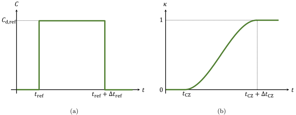
Figure 4.7: Stabilisation of refinement. (a): Damping function employed to stabilise the weak refinement, where C_{d,ref} is the damping value, t_{ref} is the time of refinement and \Delta t_{ref} is the duration of the damping. (b): Weight function (1 - \kappa) to gradually release the node pairs of the strong refinement, where t_{CZ} is the time of refinement (CZ element introduction) and \Delta t_{CZ} is the duration of the transition.
