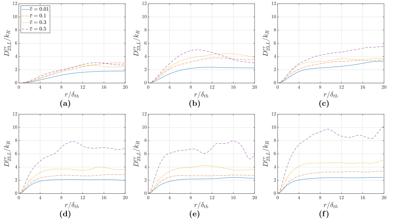
Fig. 9: Variations of D_{23,L}^{rr}/k_R with r/\delta_{th} for different values of \bar{c} for (a-f) cases A-F.
