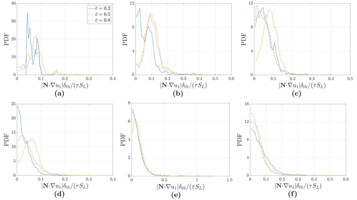
Fig. 8: PDFs of |\bar{\mathbf{N}} \cdot \nabla u_1| \delta_{th} / \tau S_L for either |N_2| \geq 0.95 or |N_3| \geq 0.95 for different values of \bar{c} for (a-f) cases A-F.
