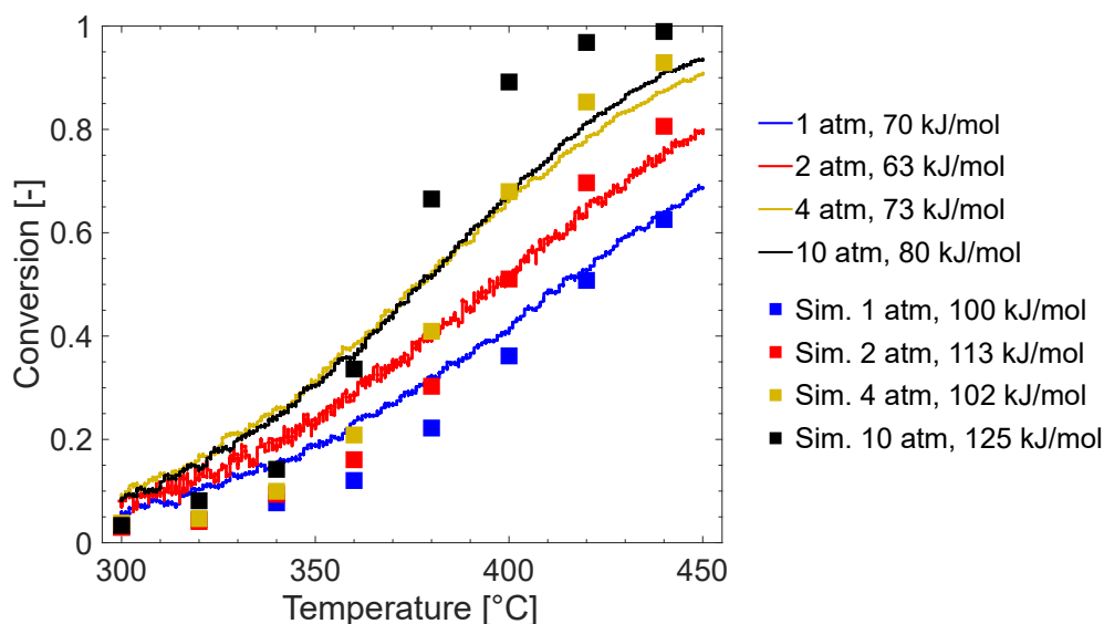
Figure 4.1: Experimental (lines) and simulated methane conversion (squares) at 1 (blue), 2 (red), 4 (yellow) and 10 (black) atm in dry conditions (0.1 vol.-% CH 4 + 2 vol.-% O 2 ) and activation energies. The gas flow was balanced in Ar with an inlet space velocity of 100 mL min -1 , which corresponds to a GHSV of 3500 h -1 at atmospheric total pressure.
