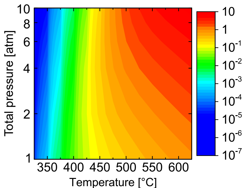
Figure 4.5: Simulated intrinsic turnover frequencies for complete methane oxidation over a Pd/Al 2 O 3 catalyst at varying temperature and total pressure. The simulated exhaust gas is comprised of 0.1 vol.-% CH 4 , 10 vol.-% O 2 , 5 vol.-% H 2 O and 5 vol.-% CO 2 .
