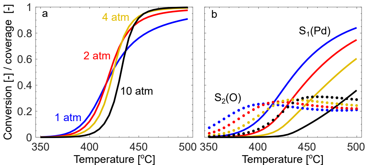
Figure 4.9: The simulated methane conversion profiles (a) with the corresponding fraction of available S_1(\text{Pd}) and S_2(\text{O}) sites on the palladium oxide surface (b). The simulated exhaust gas is comprised of 0.1 vol.-% \text{CH}_4 , 10 vol.-% \text{O}_2 , 10 vol.-% \text{H}_2\text{O} and 5 vol.-% \text{CO}_2 balanced in Ar with an inlet space velocity of 1500 \text{ mL min}^{-1} . The flow rate corresponds to a GHSV of 53\,000 \text{ h}^{-1} .
