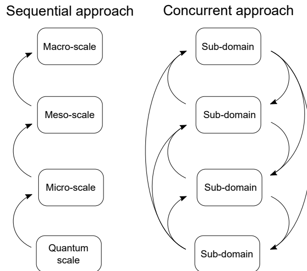
Figure 3.2: Illustration of the sequential and the concurrent approaches to model multiscale systems. The sequential approach passes the results upwards iteratively from the smallest to the largest scale in a straightforward methodology. The concurrent approach passes the results between different sub-domains which are characterised by their scale and physics.
