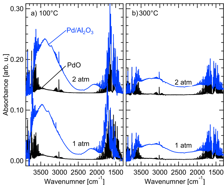
Figure 4.12: Diffusive reflectance infrared Fourier transform spectra during exposure of Pd/Al 2 O 3 (blue) and PdO (black) for 0.1 vol.% CH 4 + 10 vol.% H 2 O at 100 and 300 °C . The difference spectra were first taken at a total pressure of 1 atm followed by 2 atm.
