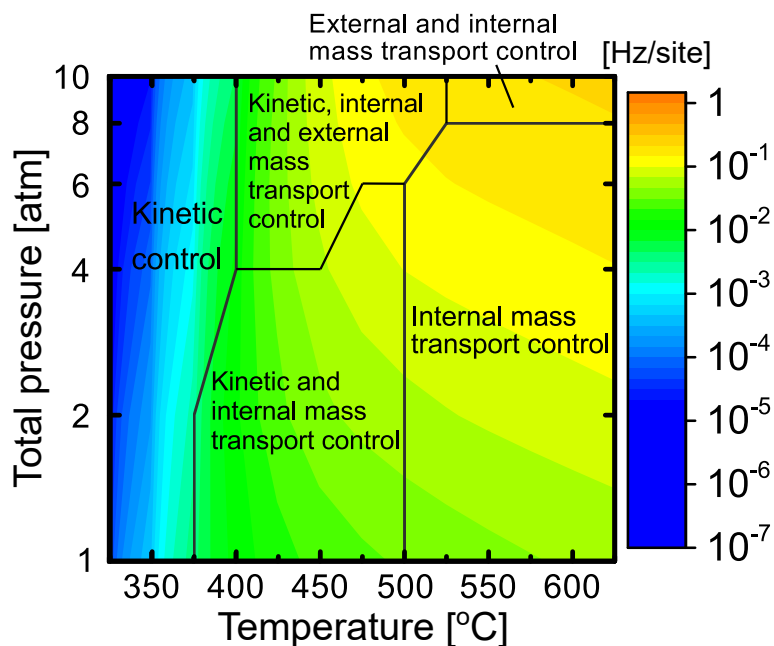
Figure 4.8: The volume averaged simulated turnover frequencies with determined controlling regions in the Pd/Al 2 O 3 catalyst for methane oxidation at varying temperature and total pressure. The simulated exhaust gas is comprised of 0.1 vol.-% CH 4 , 10 vol.-% O 2 , 5 vol.-% H 2 O and 5 vol.-% CO 2 .
