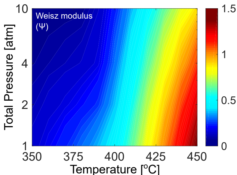
Figure 4.2: The Weisz modulus calculated at experimental inlet conditions for varying total pressures and temperatures. An average catalyst coating of 30 \mu\text{m} is estimated from optical microscopy while the reaction rate and effective diffusivity is taken from the multiscale model. Values are taken from the multiscale model since differential conditions can not be assumed at all examined conditions.
