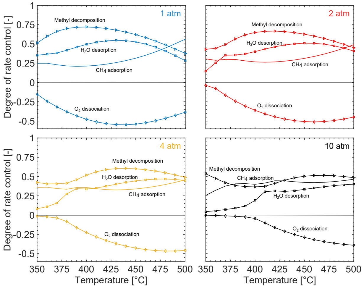
Figure 4.10: The temperature and total pressure dependent degree of rate control determined from simulations at inlet gas conditions of 0.1 vol.-% CH 4 , 10 vol.-% O 2 , 10 vol.-% H 2 O and 5 vol.-% CO 2 .
