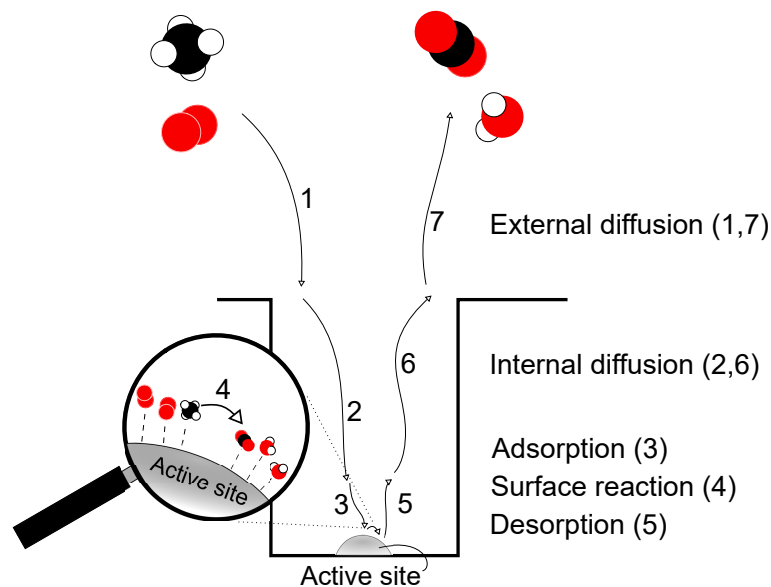
Figure 2.2: Illustration of the sub-processes of catalysed heterogeneous reaction over a solid particle in a porous support. The slowest step is called the rate-limiting or rate determining step.
