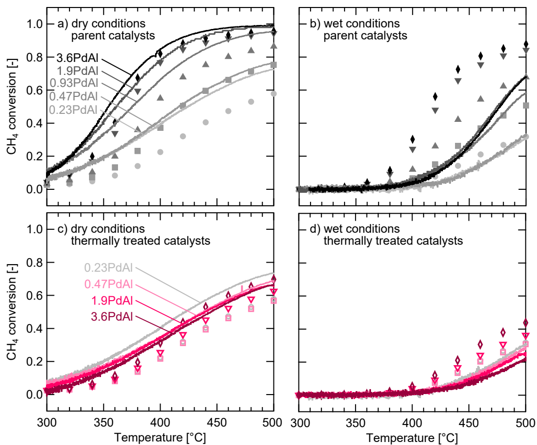
Figure 4.13: Experimental and simulated methane extinction profiles. Top row: parent samples of 0.23, 0.47, 0.93, 1.9 and 3.6 wt.-% Pd/Al 2 O 3 . Bottom row: Thermally treated samples with similar palladium areas but varied ratios of bulk-to-interface palladium sites. Left column: Dry oxidation of 0.1 % CH 4 in 2 % O 2 . Right column: Oxidation of 0.1 vol.-% CH 4 in 2 vol.-% O 2 + 10 vol.-% H 2 O.
