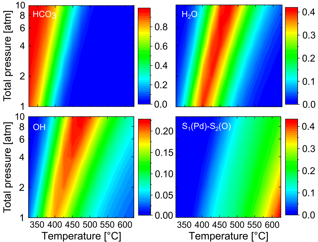
Figure 4.6: The equilibrium coverages of bicarbonate, water, hydroxyl species and the fraction of available S 1 (Pd)-S 2 (O) site configurations according to the microkinetic model. The bulk gas is comprised of 0.1 vol.-% CH 4 , 10 vol.-% O 2 , 5 vol.-% H 2 O and 5 vol.-% CO 2 .
