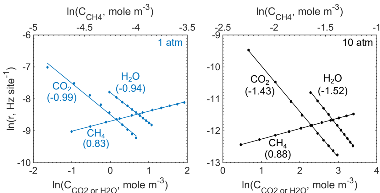
Figure 4.11: Reaction orders for methane, carbon dioxide and water at 1 (blue) and 10 (black) atm. The reaction orders are determined using the 2D multiscale model for a gas composition of 0.1 vol.-% CH 4 , 10 vol.-% O 2 , 10 vol.-% H 2 O and 5 vol.-% CO 2 balanced in Ar at a total inlet flow rate of 1500 mL min -1 .
