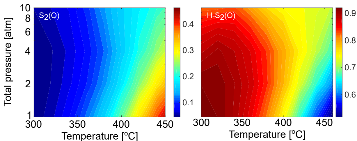
Figure 4.4: The fraction of unoccupied under-coordinated oxygen sites (left) and the coverage of adsorbed hydrogen on the S_2(O) site (right) at varying temperatures and total pressures according to the microkinetic model.
