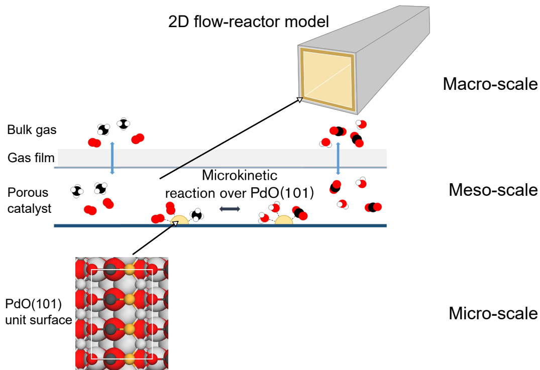
Figure 3.5: An illustration of the 2D multiscale model.
