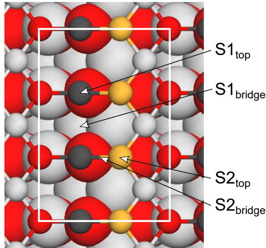
Figure 3.3: The structure of the PdO(101) surface with arrows indicating the different adsorption locations. S1 and S2 denote adsorption on palladium and oxygen, respectively. Adsorption events are possible at a top or a bridged configuration for each surface atom. Atoms in the top-most layer are visualised with smaller balls for clarity. The white box indicates the surface unit cell. Black is a threefold coordinated Pd, yellow is a threefold coordinated O while gray and red are the fourfold coordinated arrangements of Pd and O, respectively.
