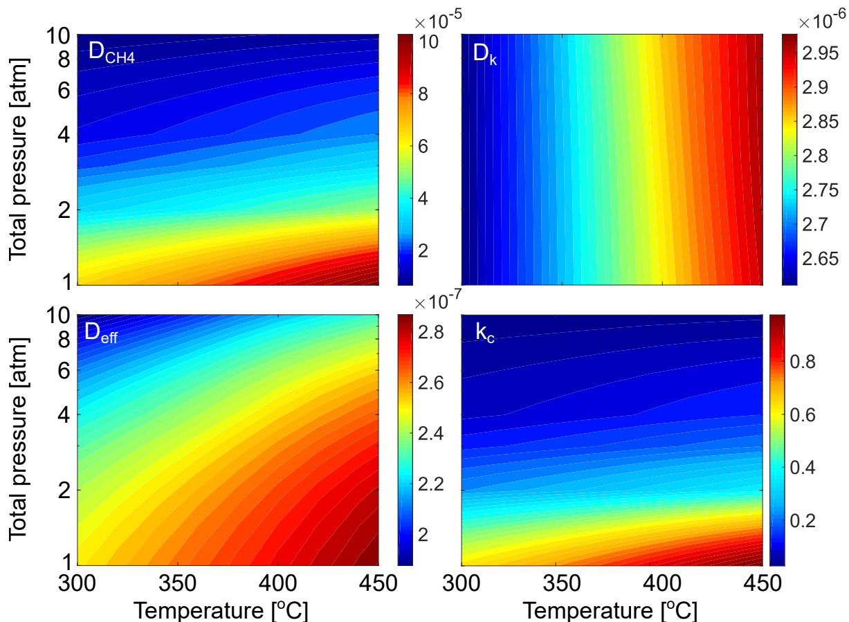
Figure 4.3: The bulk molecular diffusion (a), Knudsen diffusion (b) and the effective diffusivity (c) for CH_4 at inlet conditions according to the multiscale model.
