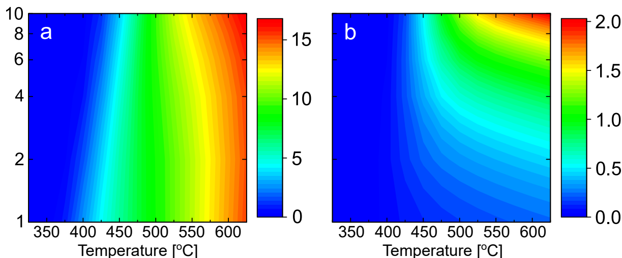
Figure 4.7: The significance of internal (a) and external (b) mass transport for complete methane oxidation in a Pd/Al 2 O 3 washcoat at varying temperature and total pressure. The simulated exhaust gas is comprised of 0.1 vol.-% CH 4 , 10 vol.-% O 2 , 5 vol.-% H 2 O and 5 vol.-% CO 2 .
