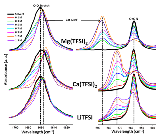
Figure 5. IR spectra of DMF-based electrolytes as a function of \text{Mg}(\text{TFSI})_2 , \text{Ca}(\text{TFSI})_2 , and LiTFSI salt concentrations.
