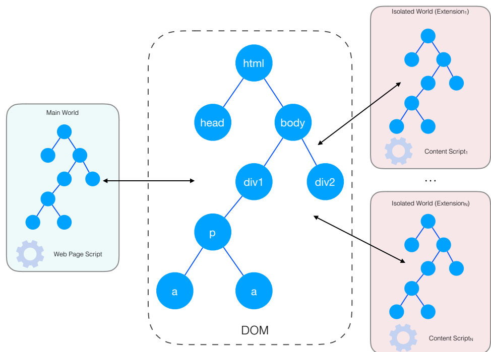
Fig. 5 Chromium’s execution model for extensions
