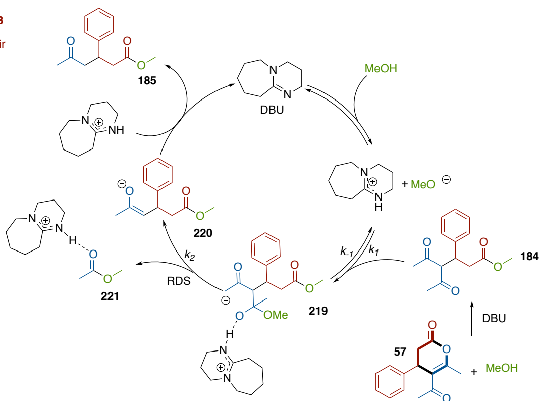
Scheme 29. The two proposed mechanism for the ring-opening and retro-Claisen fragmentation of dihydropyranones. Both options are consistent with the observed rate law.
