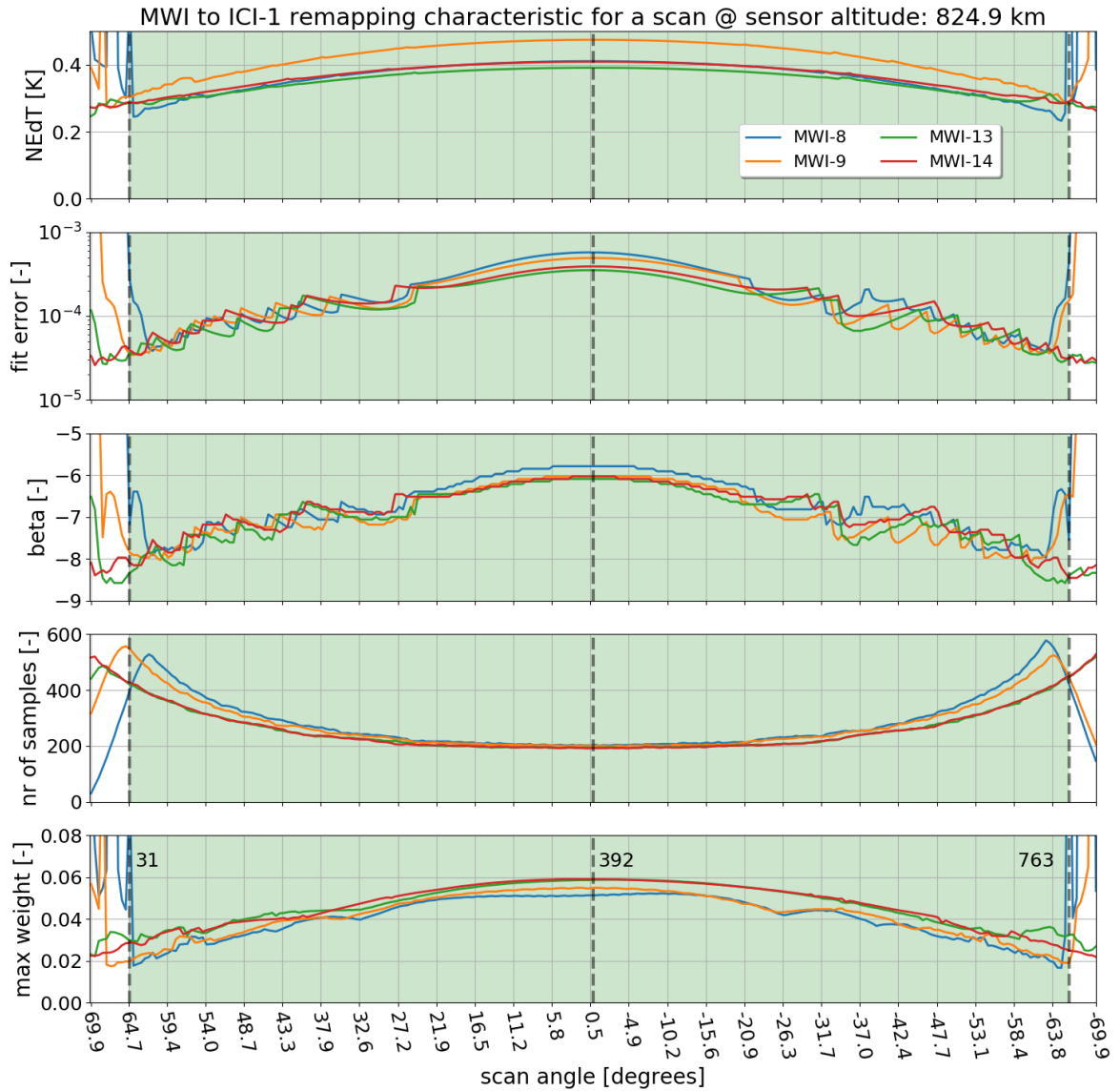
Figure 57: Trade off analysis data as function of scan angle / scan position for MWI to ICI-1 remapping. The two upper panels show the obtained noise error and fit error. The middle panel shows the optimal value of the smoothing parameter deployed in the BG methodology. The fourth panel shows the number of samples that are found within 30[km] from the geolocation of the center of the target footprint, and used in the remapping calculation. The bottom panel shows the maximum weight given to a single sample.
