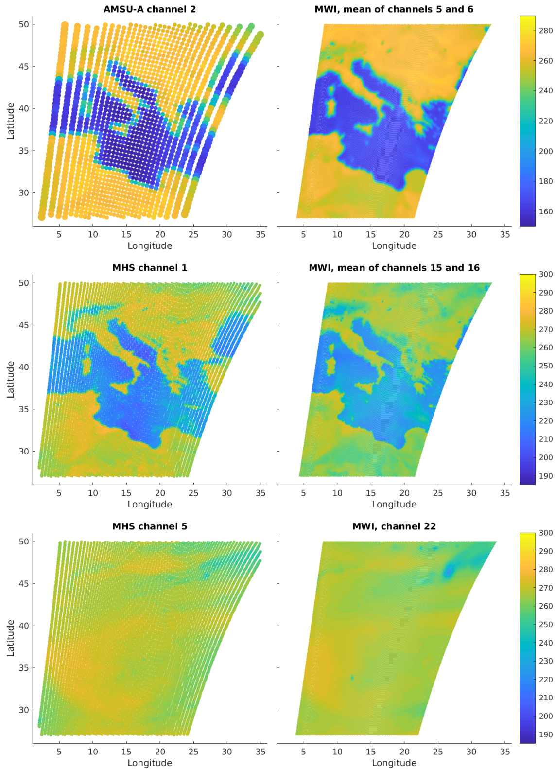
Figure 17: Observations by AMSU and MHS (left column) and MWI simulations (right column) for part of orbit 6895. The observation and simulations are not directly comparable, mainly due to different scanning patterns. See the text for details.
