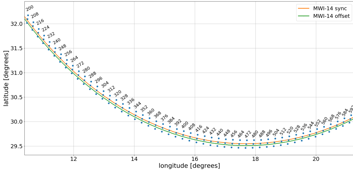
Figure 59: Gelocations of sample positions in the center part of three consecutive scans for ICI-1 samples (blue dots), and for sample positions of a "single" scan for MWI-14. Two versions of the this "single" scan are displayed, one where the start time of the MWI-14 and the center ICI scan is synchronized, and one where the MWI-14 scan is delayed by half the scan duration time.
