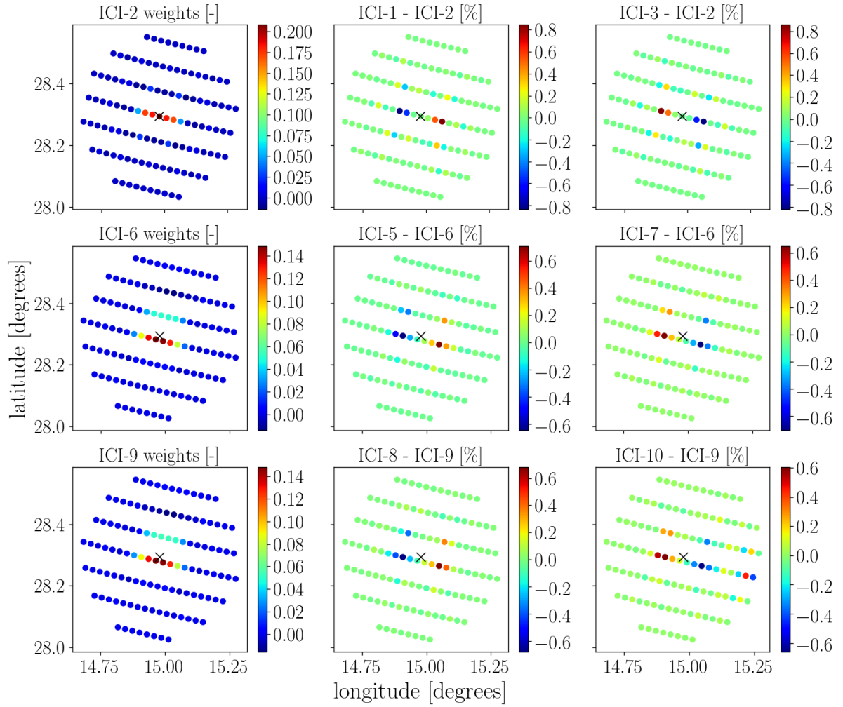
Figure 52: Difference in weighting coefficients for channels with similar characteristic. The left column show derived weighting coefficients for samples within 30[km] from the geolocation of the target footprint (marked with x) for ICI-2, ICI-6, and ICI-9. The middle and right panel in upper row show difference of derived weighting coefficients for ICI-1 and ICI-3, respectively, relative to that of the max value of weighting coefficients for ICI-2. The middle and lower row show corresponding data for ICI-5/ICI-7 and ICI-8/ICI-10.
