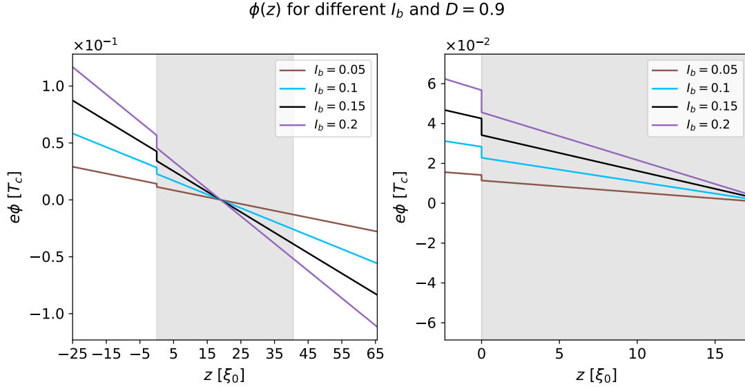
Figure 3.7: Chemical potential \phi(z) for the normal-metal system with a left-interface transparency D = 0.9 . Left: \phi(z) over the whole range of the system. Right: Enlargement of the interface region with the potential jump. The grey area marks the "central" region between the interfaces.
