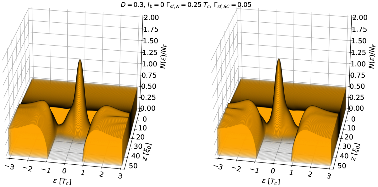
Figure 4.21: Spin-resolved, equilibrium density of states for an SAI with small transparency of D_{\downarrow} = D_{\uparrow} = 0.3 and a spin-mixing angle of \vartheta = 0.66 \pi . Spin-up DOS on the left, spin-down DOS on the right.
