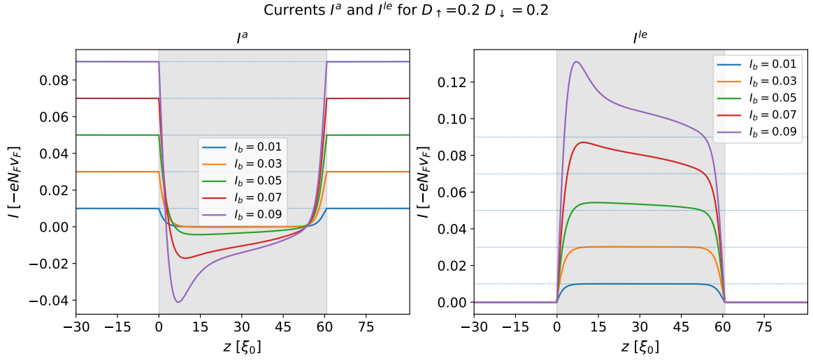
Figure 3.20: Conversion from normal-state “anomalous” current into supercurrent over the system with a left-interface transparency D = 0.2 . The dotted lines show the respective boundary current.
