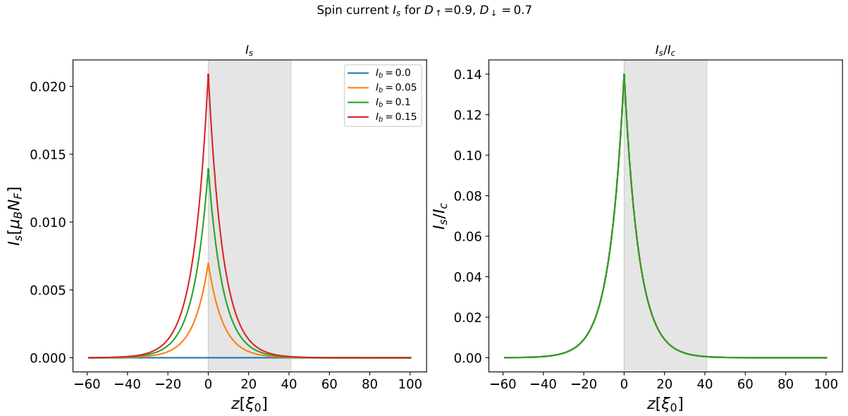
Figure 4.11: Left plot: Spin current I_s near the interface. Right plot: Current polarization P = I_s/I_c near the interface.
