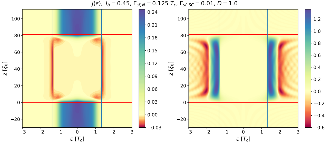
Figure 3.14: Current density for a large current in the NIS system. Left: anomalous current, right: local-equilibrium current. Red horizontal lines indicate the beginning of the superconducting region, while blue vertical lines indicate the value of the bulk spectral gap.
