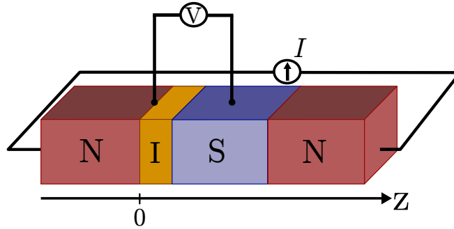
Figure 3.23: Sketch of a voltage-drop measurement in the NIS system.
