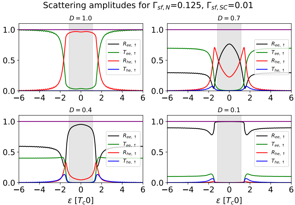
Figure 3.4: Physical scattering amplitudes on the normal side for a small impurity concentration in the SC. The purple horizontal line is the sum of all four contributions which is equal unity by current conservation.
