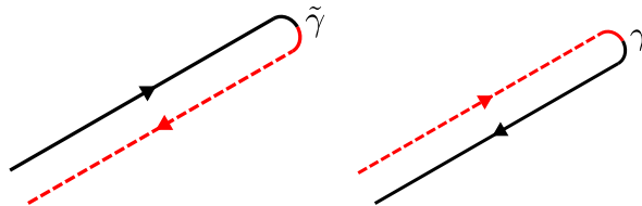
Figure 2.2: Elementary branch conversion e \rightarrow h ( h \rightarrow e ) mediated by \tilde{\gamma} ( \gamma ).
