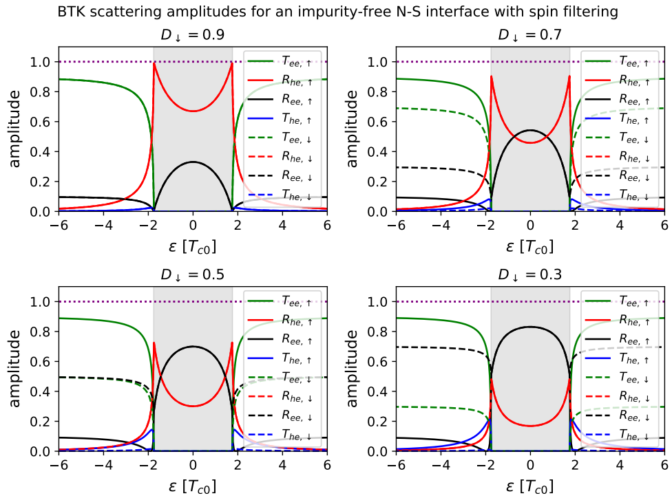
Figure 4.15: Transport amplitudes for spin filtering. The sum of all four contributions has to add to unity (purple line). In the subgap region the amplitudes for normal and Andreev reflection are degenerate for spin up and spin down quasiparticles.
