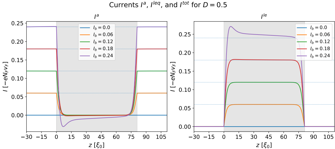
Figure 3.16: Conversion from normal-state "anomalous" current into supercurrent over the system with a left-interface transparency D = 0.5 . The dotted lines show the respective boundary current.
