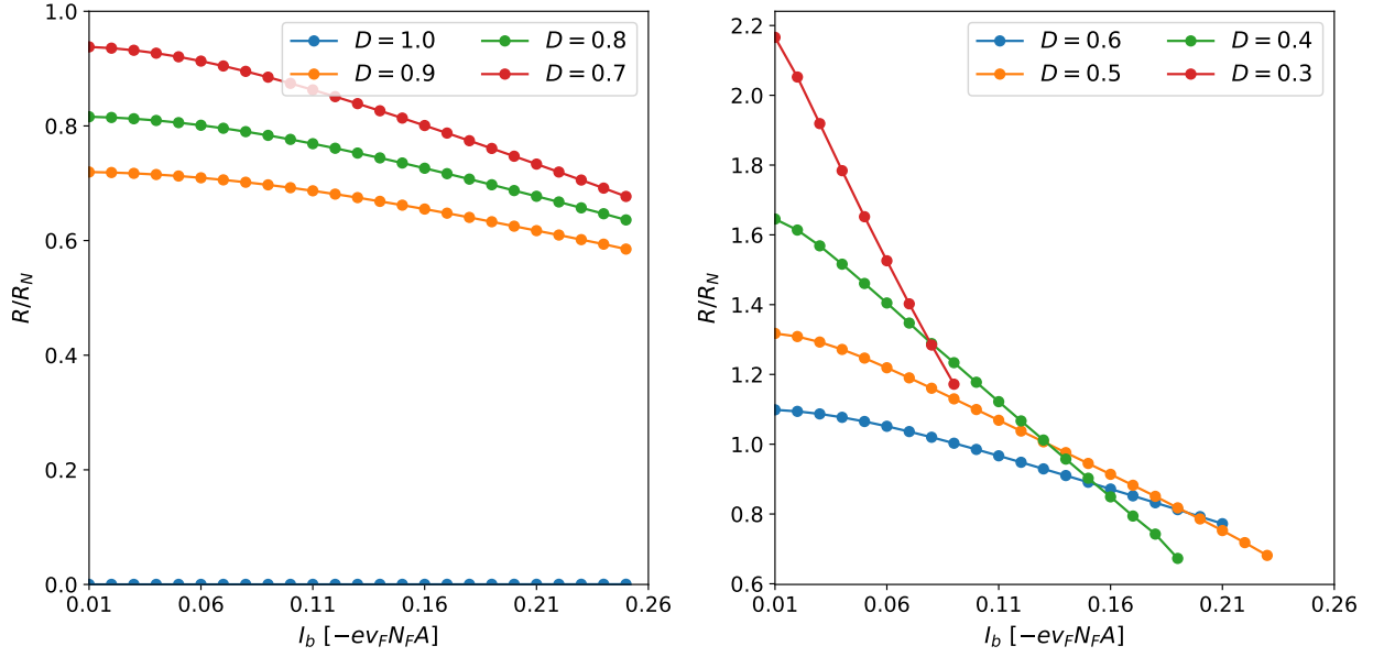
Figure 3.24: Interface resistance R_{I,SC} normalized to normal-state resistance as function of applied current for different transparency D .
