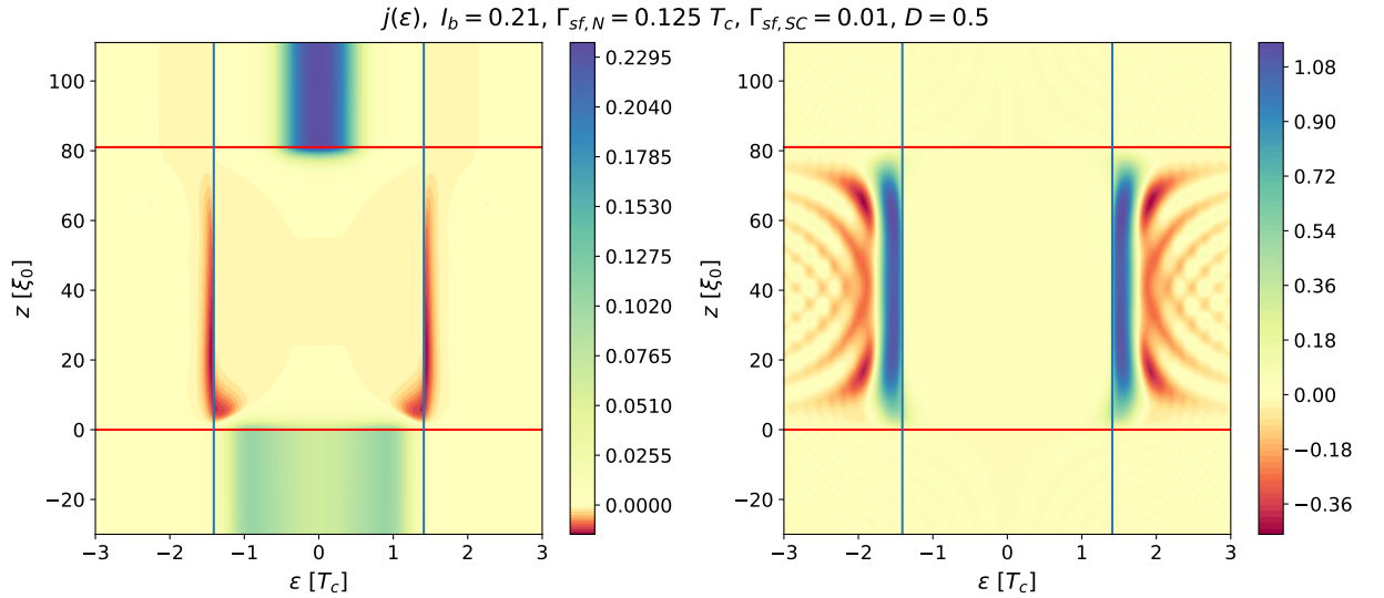
Figure 3.18: Current density for a large current in the NIS system with a left-interface transparency D = 0.5 . Left: anomalous current, right: local-equil. current. Red horizontal lines indicate the beginning of the superconducting region, while blue vertical lines indicate the value of the bulk order parameter.
