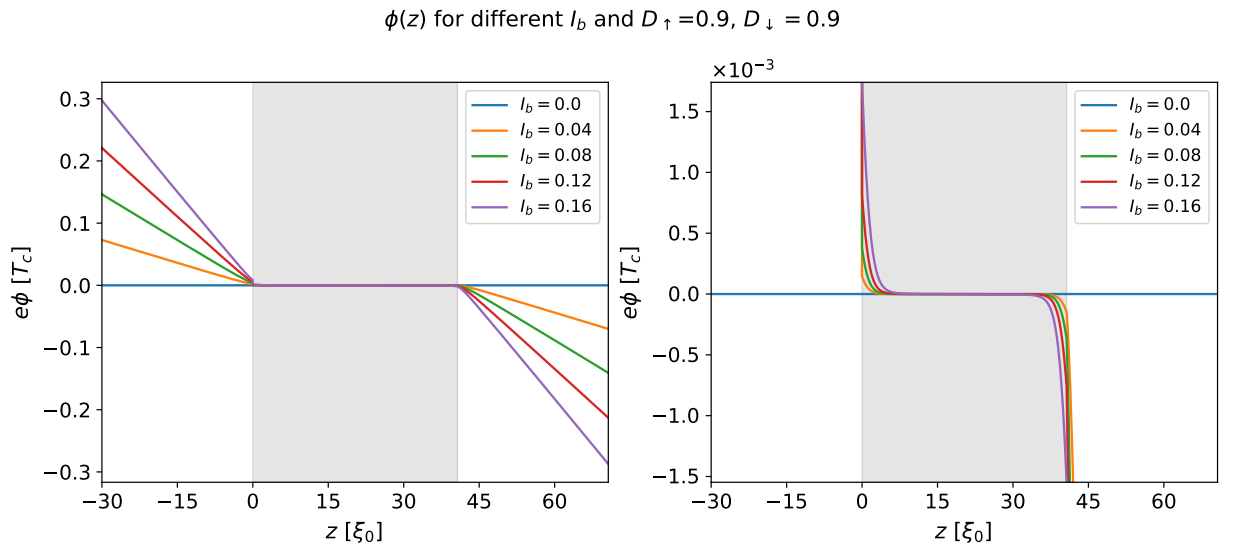
Figure 4.26: Chemical potential \phi(z) for spin-filtering in the N-SAI-S system with D_\uparrow = D_\downarrow = 0.9 and \vartheta = 0.66 \pi . Left: \phi(z) over the whole range of the system. Right: Enlargement of the central superconducting region.
