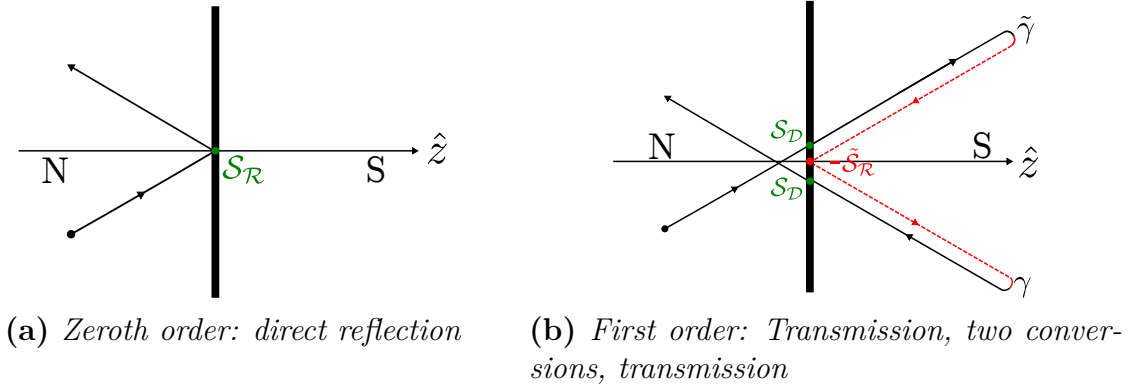
Figure 2.5: First two orders of the left-side electron reflection process r_{ee}^R
