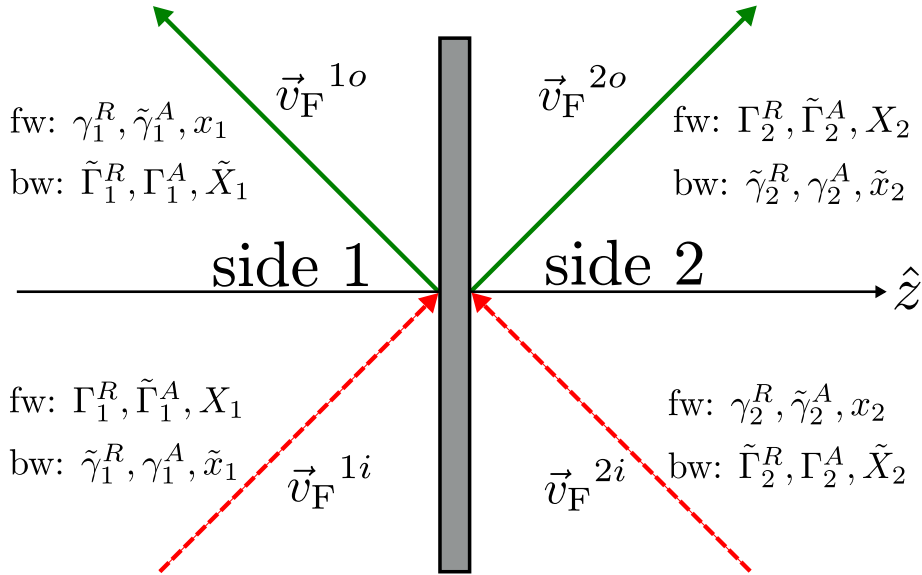
Figure 2.1: Sketch of an interface connecting two subsystems 1 and 2.
