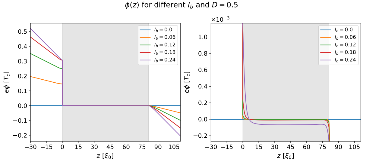
Figure 3.17: Chemical potential \phi(z) for the NIS system with a left-interface transparency D = 0.5 . Left: \phi(z) over the whole range of the system. Right: Enlargement of the central superconducting region.
