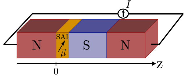
Figure 4.1: Sketch of an normal-metal/superconductor hybrid system with spin-active interface. The central S region can also be replaced by a normal conductor, referred to as NIN system.
