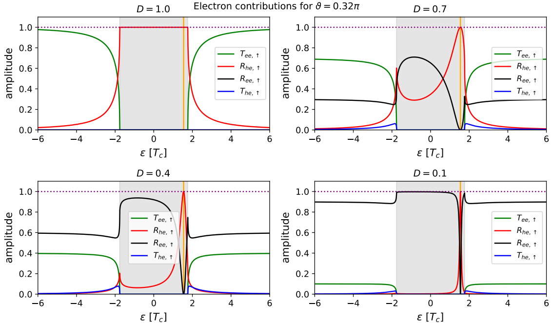
Figure 4.6: Physical mechanisms for charge transport at the N-S interface on the normal side. The purple-dotted line is the sum of all four contributions which has to equal unity according to Eq. (2.77), the orange line is the position of the ABS.
