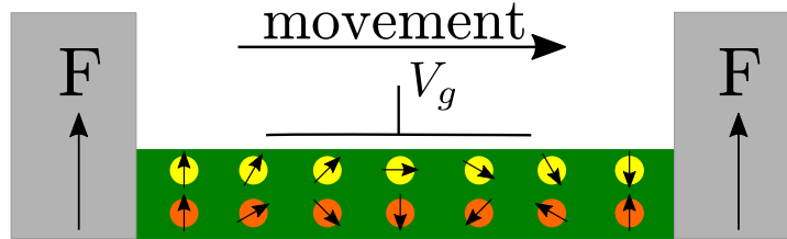
Figure 1.1: Working principle of a spin transistor, based on Ref.[17]. Depending on the gate-voltage dependent spin-orbit coupling in the central (green) 2DEG, the final spin orientation will be parallel or antiparallel to the right-hand magnetization, allowing or disallowing transport.
