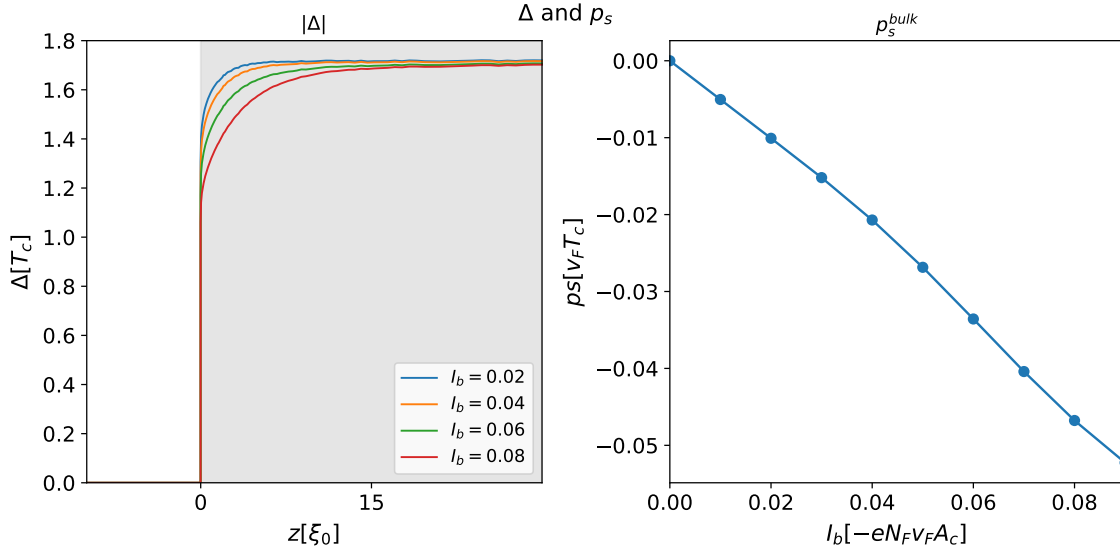
Figure 3.22: Spatial dependence of the order parameter (left) and bulk value of the superflow p_s (right) for small currents with a left-interface transparency D = 0.5
