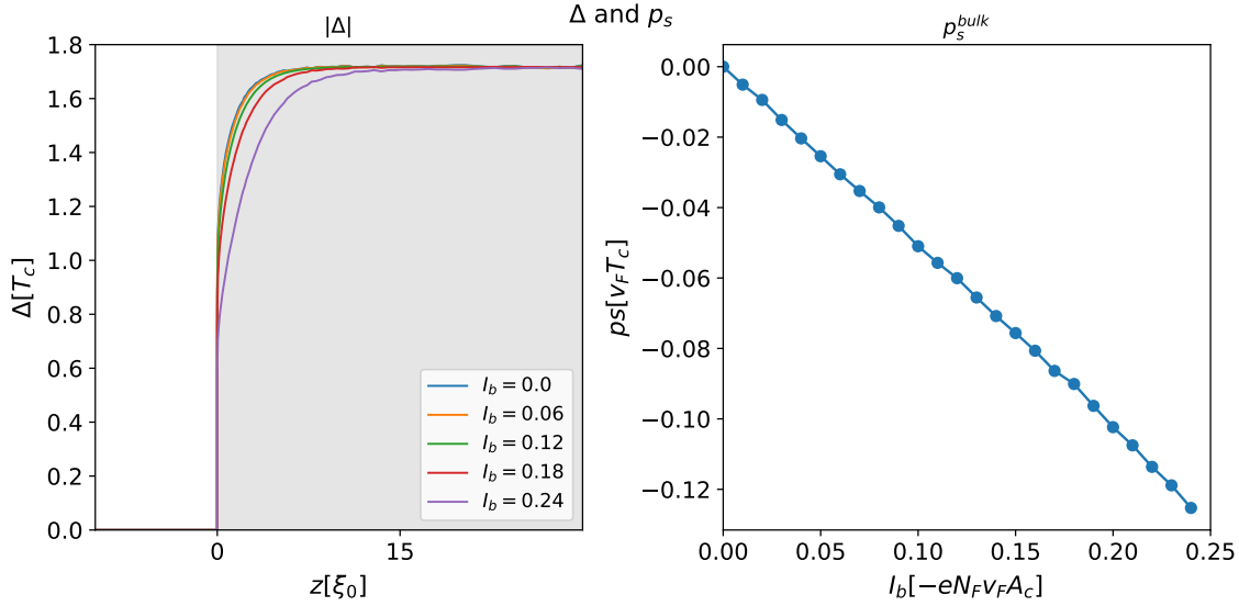
Figure 3.19: Spatial dependence of the order parameter (left) and bulk value of the superflow p_s (right) for small currents with a left-interface transparency D = 0.5
