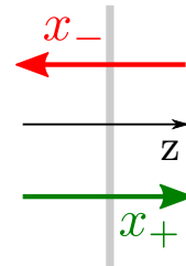
Figure 2.6: Current flow and distribution functions x .
