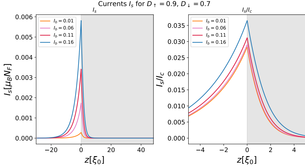
Figure 4.20: Spin current and current polarization in the superconducting system with D_\uparrow = 0.9 and D_\downarrow = 0.7 .
