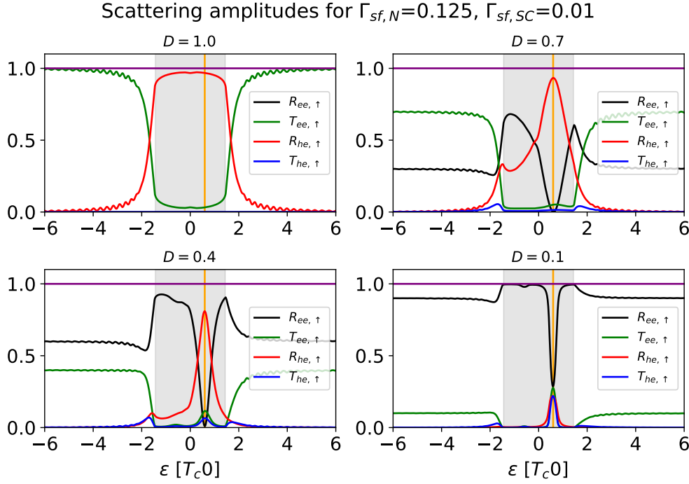
Figure 4.7: Physical mechanisms for charge transport at the N-S interface on the normal side with small impurity concentration. The purple-dotted line is the sum of all four contributions which has to equal unity according to Eq. (2.77), the orange line is the position of the ABS.
