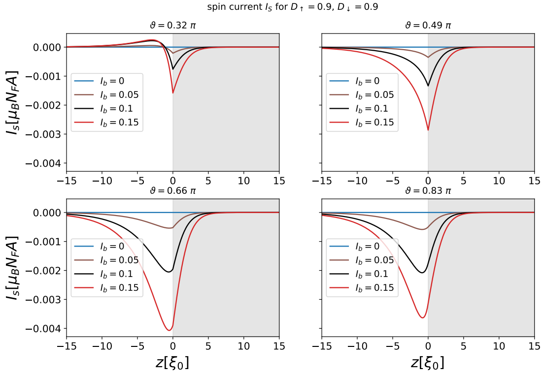
Figure 4.29: Spin current in the NSN system with D_\uparrow = 0.9 and D_\downarrow = 0.9 for different spin-mixing angle \vartheta and currents I_b . The grey area marks the superconducting region.
