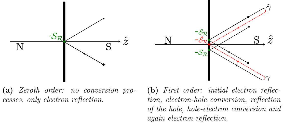
Figure 2.3: First two orders of the electron reflection process \bar{r}_{ee}^R
