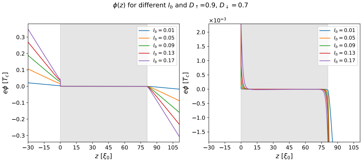
Figure 4.13: Chemical potential \phi(z) for spin-filtering in the NSN system with a left-interface transparency D_{\uparrow} = 0.9 and D_{\downarrow} = 0.7 . Left: \phi(z) over the whole range of the system. Right: Enlargement of the central superconducting region.
