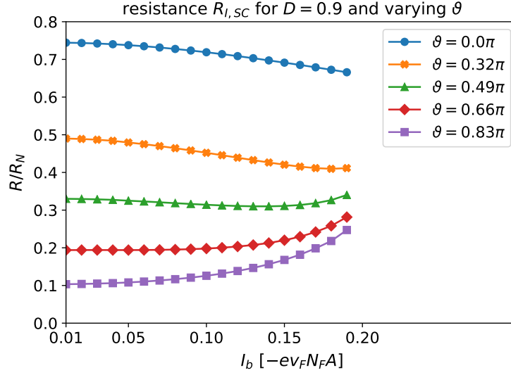
Figure 4.27: Resistance R_I at the SAI for D_{\uparrow,\downarrow} = 0.9 for different spin-mixing angle \vartheta and currents I .
