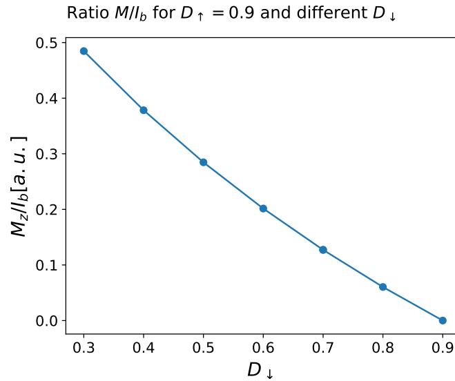
Figure 4.12: Ratio of Magnetization over current, M_z/I_b , for varying transmission D_{\downarrow} at fixed D_{\uparrow} = 0.9 .
