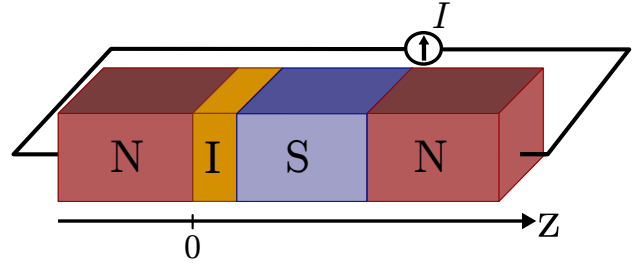
Figure 3.1: Sketch of an normal-metal/superconductor hybrid system with an insulating barrier, that will be parametrized by a normal-state transparency D . The central S region can also be replaced by a normal conductor, referred to as NIN system.
