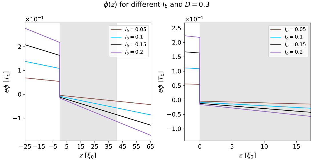
Figure 3.8: Chemical potential \phi(z) for the normal-metal system with a left-interface transparency D = 0.3 . Left: \phi(z) over the whole range of the system. Right: Enlargement of the interface region with the potential jump. The grey area marks the "central" region between the interfaces.
