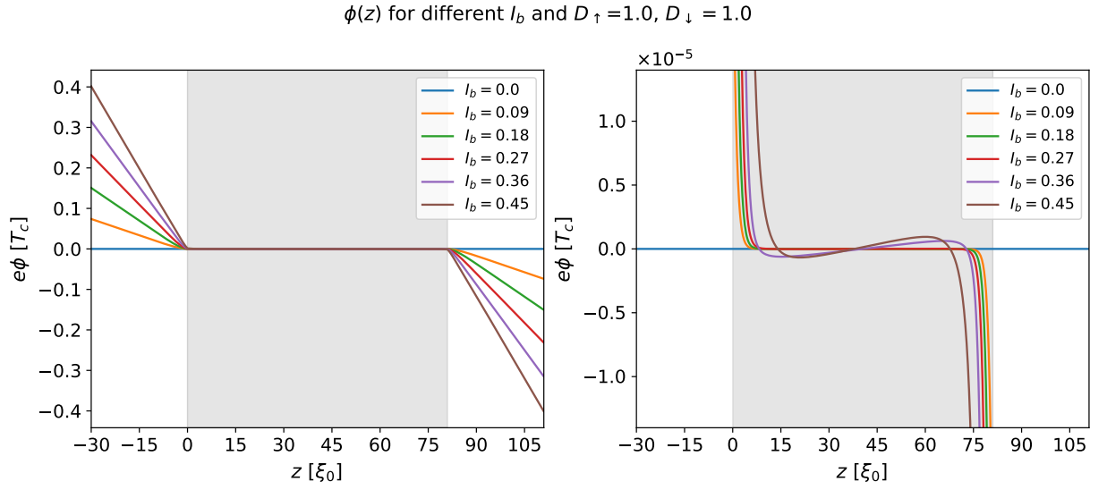
Figure 3.10: Chemical potential \phi(z) for the spin-degenerate NIS system with a left-interface transparency D = 1.0 . Left: \phi(z) over the whole range of the system. Right: Enlargement of the central superconducting region. The grey area marks the superconducting region.
