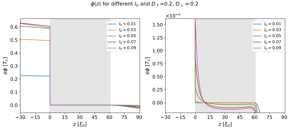
Figure 3.21: Chemical potential \phi(z) for the NIS system with a left-interface transparency of D = 0.2 . Left: \phi(z) over the whole range of the system. Right: Enlargement of the central superconducting region.
