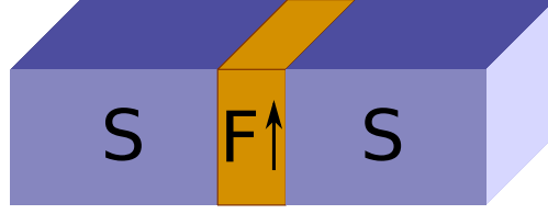
Figure 1.2: A ferromagnetic Josephson junction.
