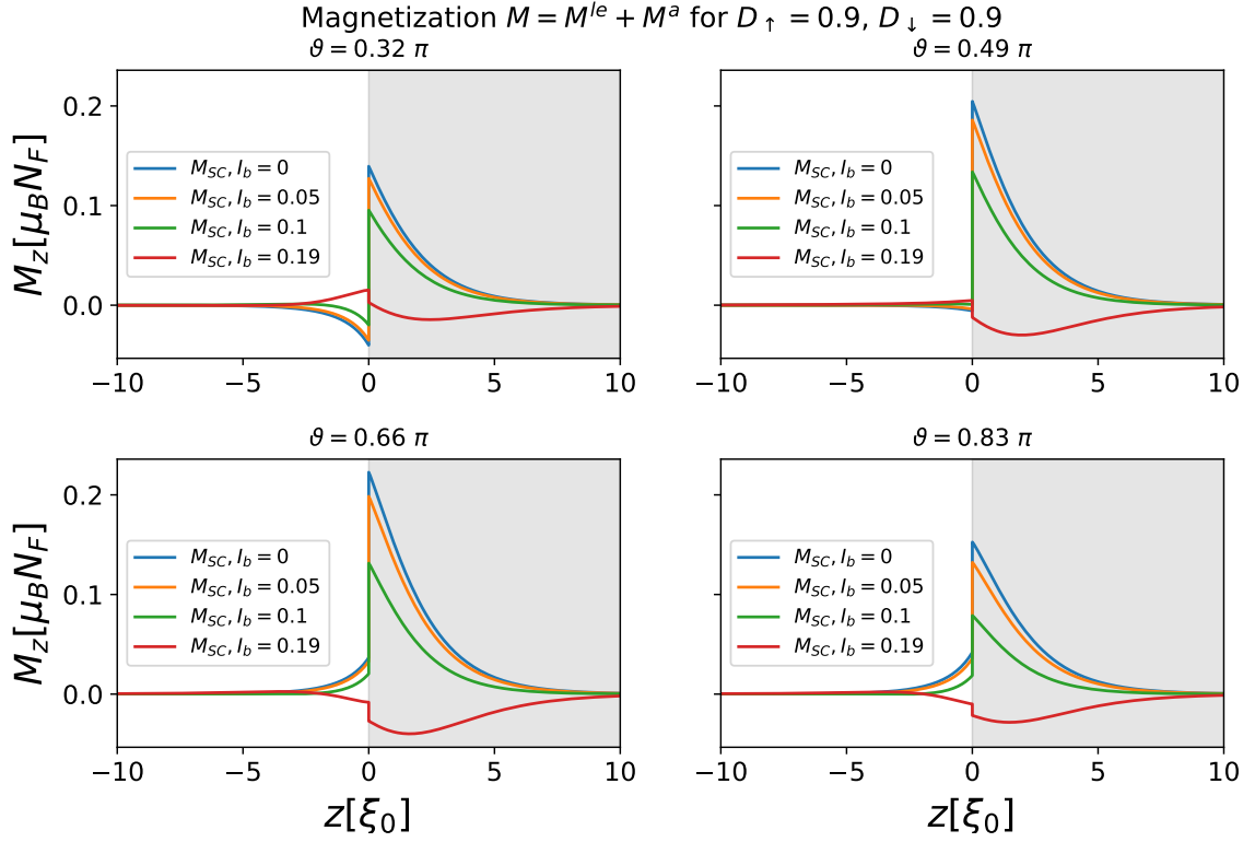
Figure 4.22: Magnetization at the SAI for high transparency of D = 0.9 and different spin-mixing angle \vartheta . The grey area marks the superconducting region.
