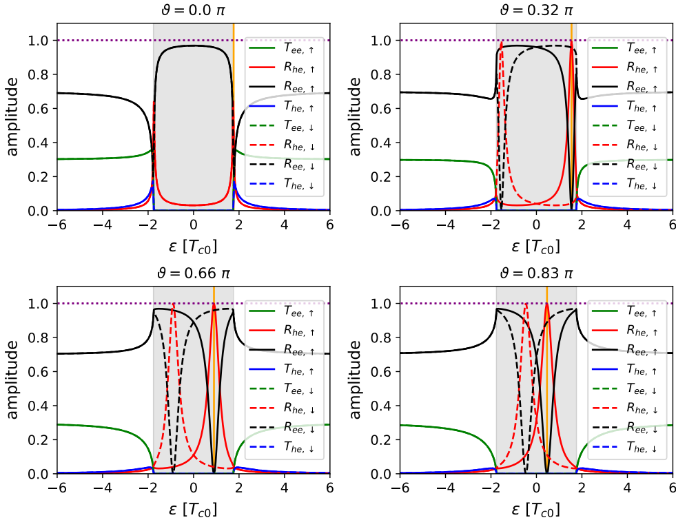
Figure 4.31: Scattering amplitudes for a small-transparency ( D = 0.3 ) SAI for different spin-mixing angles. The purple-dotted line is the sum of all four contributions which has to equal unity to ensure probability current conservation, the orange line is the position of the ABS.
