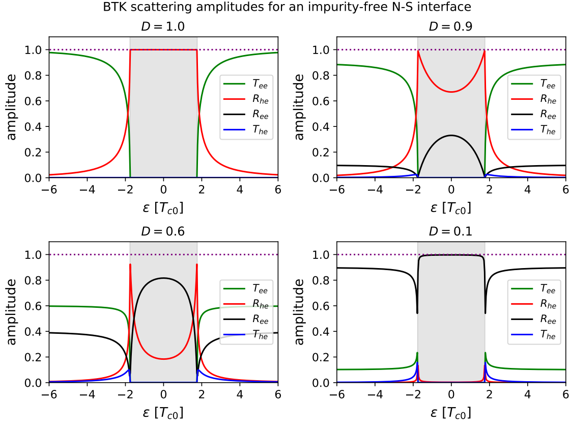
Figure 3.3: Different physical mechanisms for charge transport at the N-S interface on the normal side. The purple-dotted horizontal line is the sum of all four contributions which has to equal unity according to Eq. (2.77).
