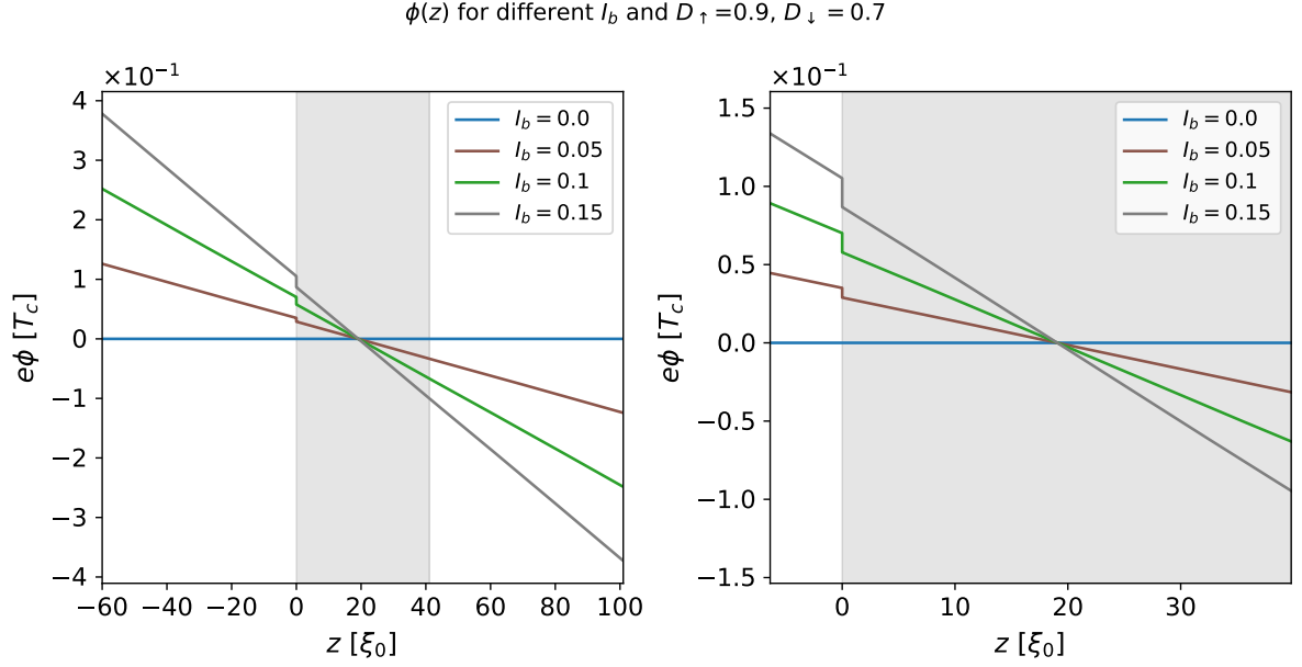
Figure 4.8: Chemical potential \phi(z) for spin-filtering in the NIN system. Left: Drop of \phi over the whole range of the system. Right: Enlargement of the central region with the potential jump at the interface, always for the respective top figure.
