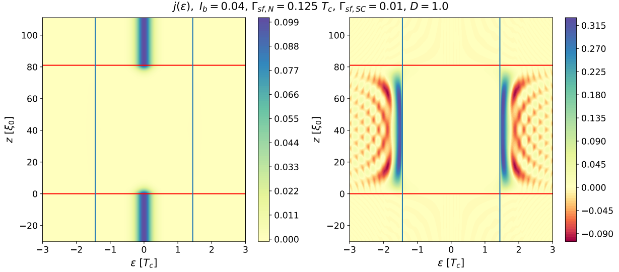
Figure 3.12: Current density for a small current in the NSN system. Left: anomalous current, right: local-equilibrium current. Red horizontal lines indicate the beginning of the superconducting region, while blue vertical lines indicate the value of the bulk order parameter.
