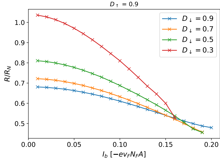
Figure 4.14: Interface resistance R_I normalized to respective normal-state resistance at the SAI for D_{\uparrow} = 0.9 , different transparency D_{\downarrow} and currents I_b .
