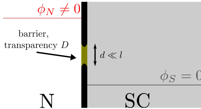
Figure 1.4: Sketch of a Sharvin contact: Only a contact of size d much smaller than the electron mean free path l is open for particle transmission with probability D . Directly at the contact, the potential drops from the normal-metal "reservoir" value \phi_N to potential \phi_S of the (grounded) superconductor.
