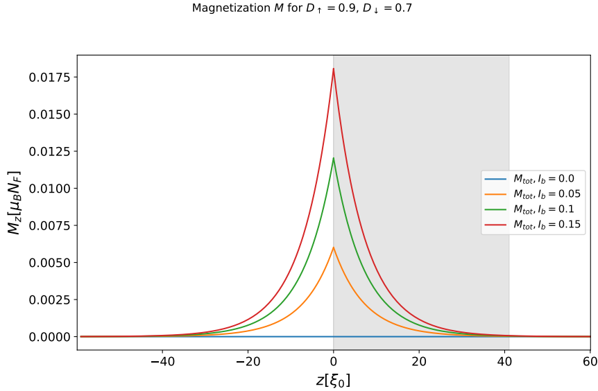
Figure 4.10: Magnetization M(z) induced by the SAI, at z = 0 \xi_0 , for small spin-filtering. The grey area marks the central region.
