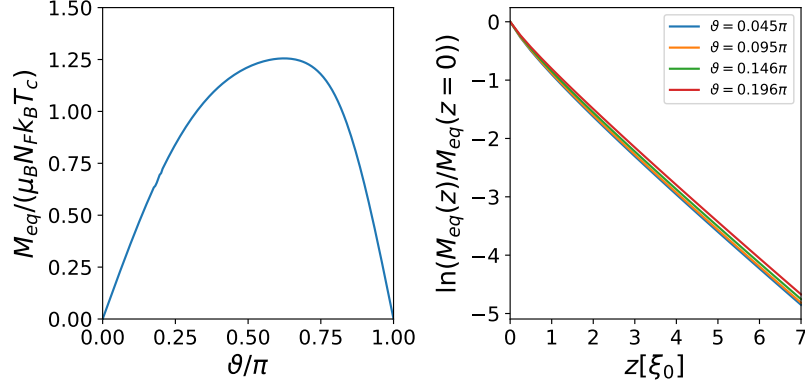
Figure 4.5: Equilibrium magnetization at the SAI as function of spin-mixing angle \vartheta (left) and decay into the bulk of the SC (right).
