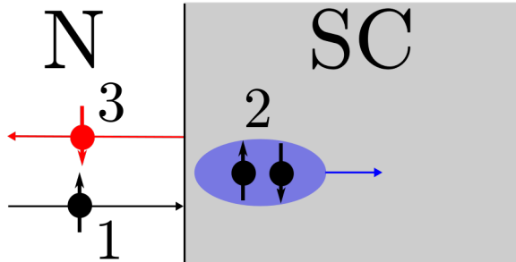
Figure 3.2: Andreev reflection at an NS interface: When an electron in the normal metal (1) reaches a perfectly transmitting interface to a SC region, an excess Cooper pair (2) is created in the superconductor, while a hole is "reflected" back into the normal metal (3). Note that the hole will have opposite spin compared to the electron so that angular momentum is conserved in the entire process.
