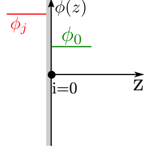
Figure 2.7: Potentials at the system edge.
