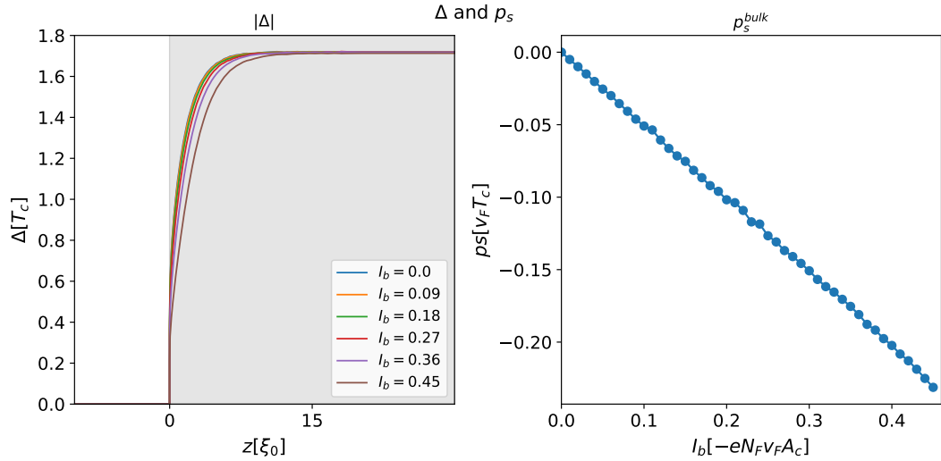
Figure 3.15: Spatial dependence of the order parameter (left) and bulk value of the superflow p_s (right) for small currents and transparency D = 1 .
