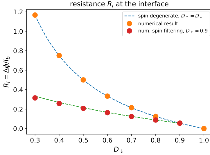
Figure 4.9: Resistance R_I at the SAI for spin filtering with different transparency D_{\downarrow} .
