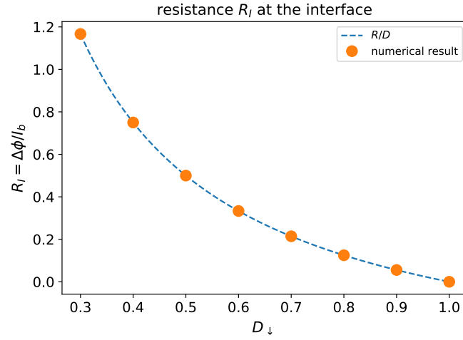
Figure 3.9: Resistance R_I at the interface for different transparency D .
