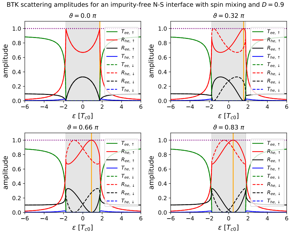
Figure 4.28: Scattering amplitudes for a SAI with D = 0.9 for different spin-mixing angles. The purple-dotted line is the sum of all four amplitudes and equal to unity, ensuring probability current conservation, the orange line is the position of the ABS.
