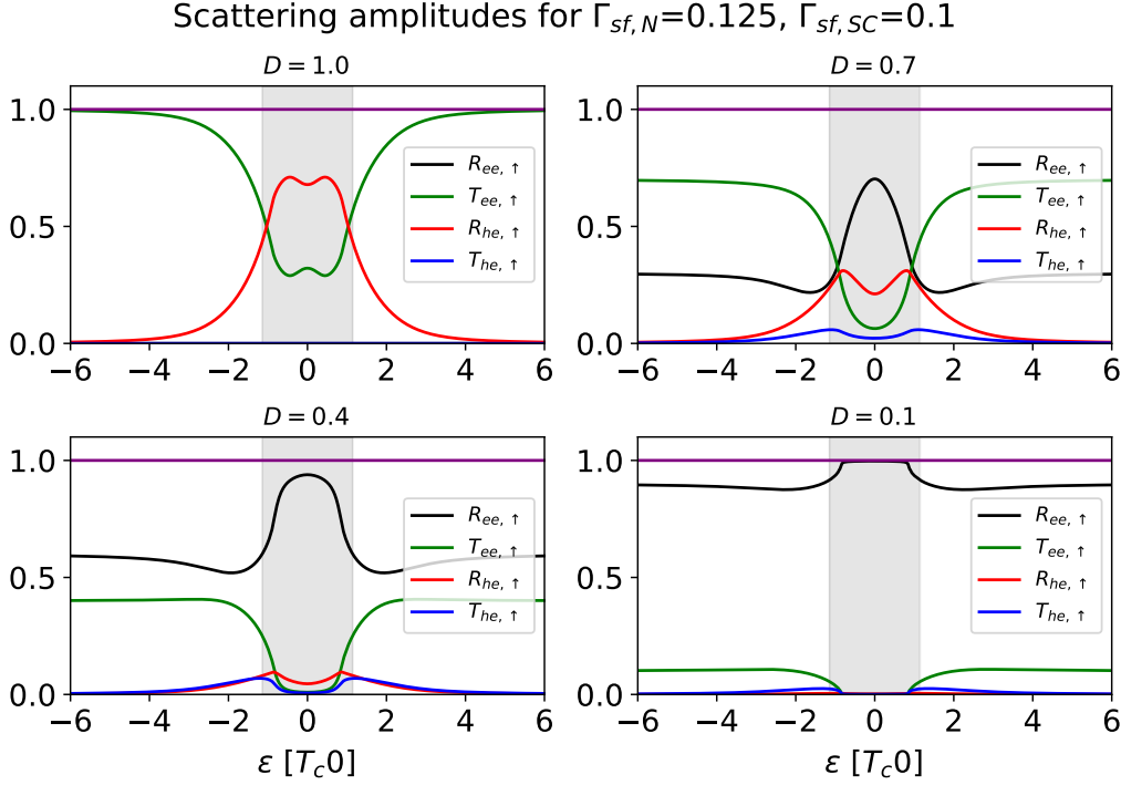
Figure 3.5: Physical scattering amplitudes on the normal side for a high impurity concentration in the SC. The purple horizontal line is the sum of all four contributions which is equal unity by probability current conservation.
