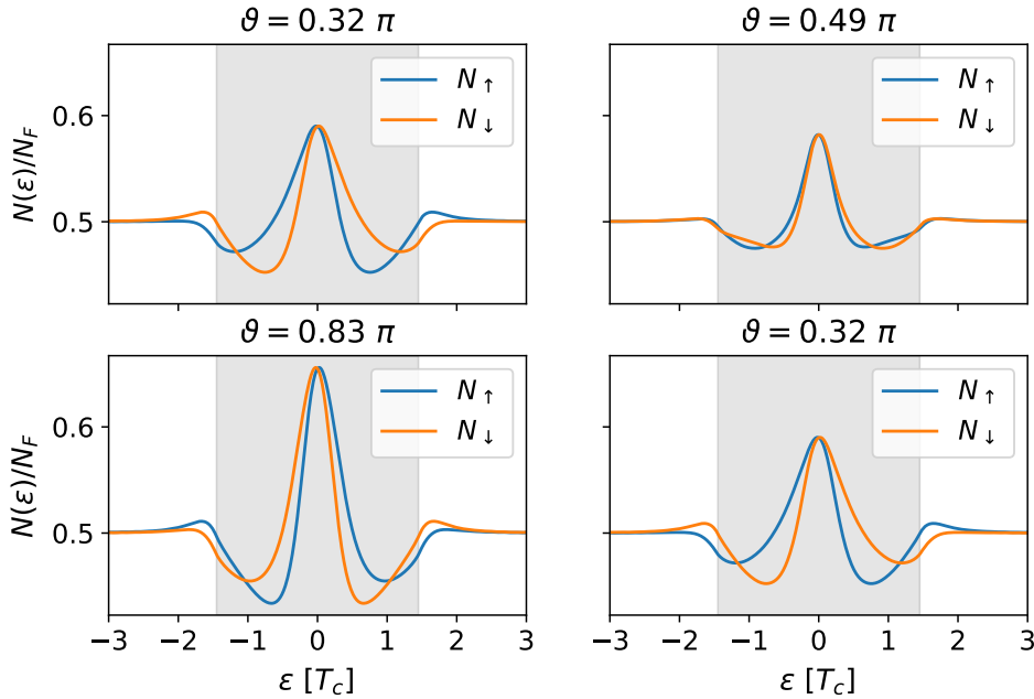
Figure 4.24: Normal-side density of states the SAI for a high transparency of D = 0.9 and different values of the spin-mixing angle \vartheta . The grey area marks the width of the bulk mean-field energy gap in the superconductor.
