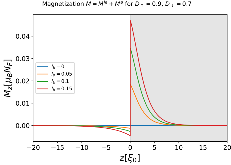
Figure 4.16: Magnetization M(z) for spin-filtering and subsequent decay with distance to the SAI located at z = 0 \xi_0 . The gray area marks the superconducting region.
