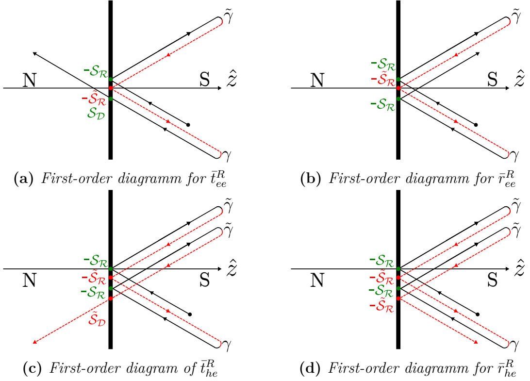
Figure 2.4: First-order processes for all four amplitudes \bar{t}_{ee}^R , \bar{r}_{ee}^R , \bar{t}_{he}^R , \bar{r}_{he}^R
