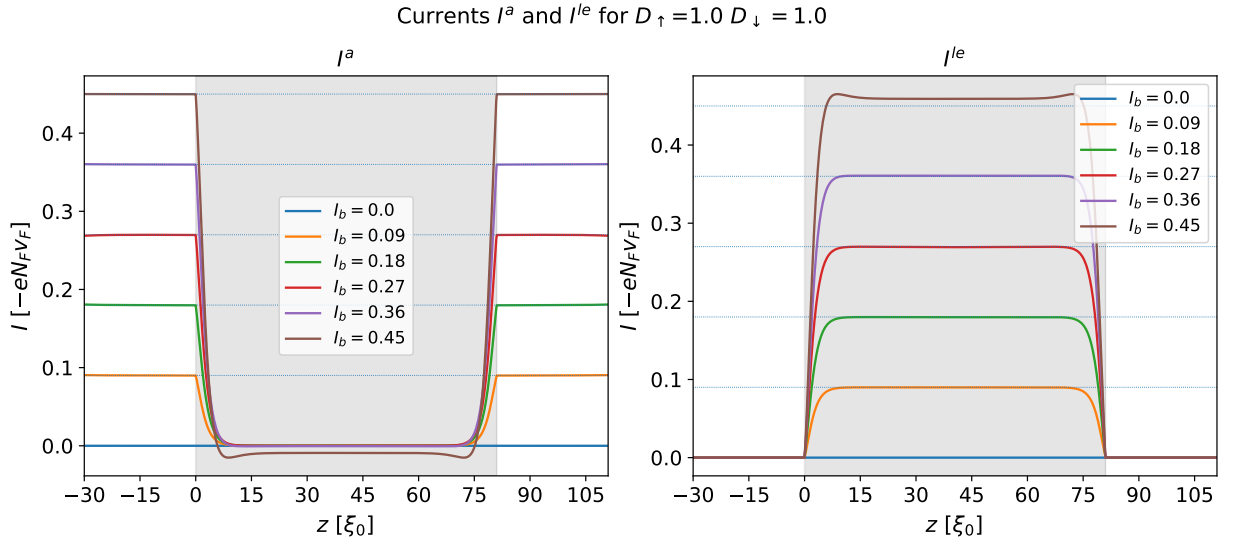
Figure 3.11: Conversion from normal-state "anomalous" current into supercurrent over the system. The dotted lines show the respective boundary current.
