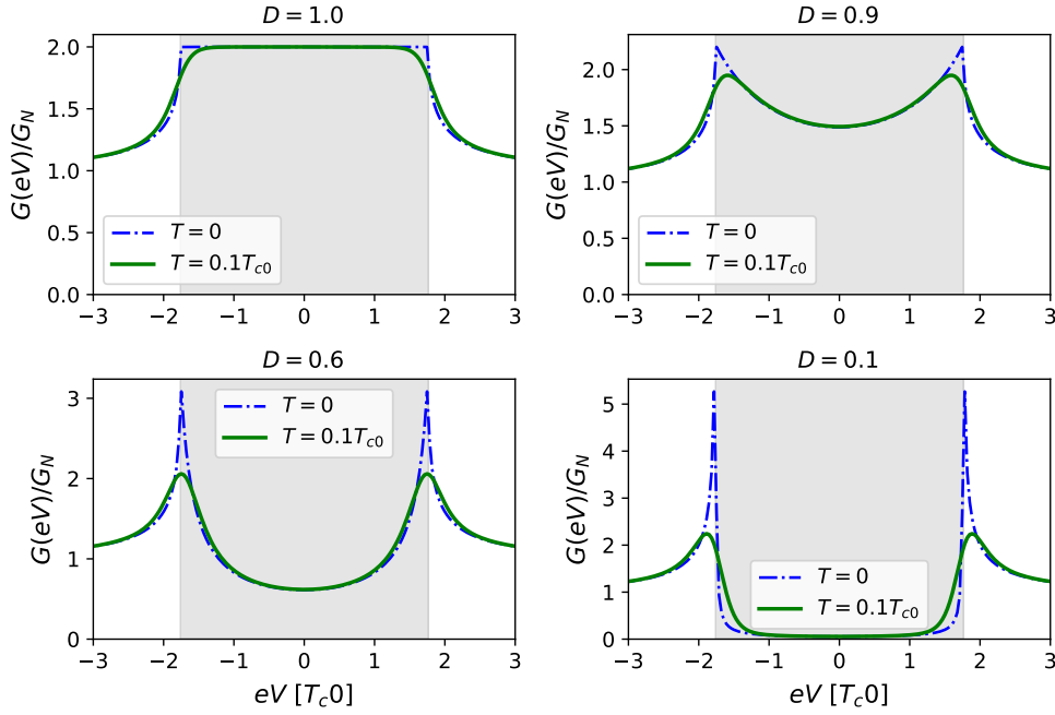
Figure 3.6: Normalized differential conductance at the NS-interface for T = 0 and T = 0.1 T_{c0} . The grey area marks the superconducting energy gap.
