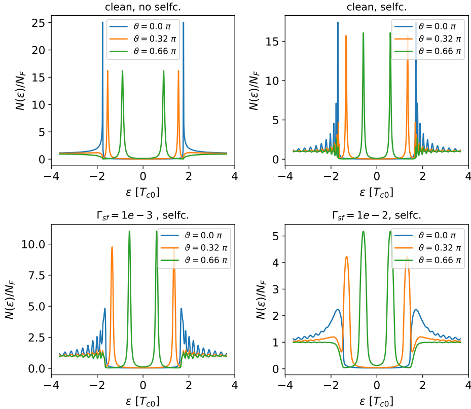
Figure 4.3: Density of states at the SAI for D = 0.06 , different impurity strengths in the SC and spin-mixing angle. The oscillations are so-called Tomasch oscillations that are suppressed by high impurity concentration and average out if more trajectories are included in the calculation.
