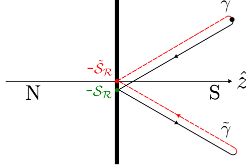
Figure 4.2: Formation of an Andreev bound state: An electron starting in the black dot (top right) gets reflected at the SAI ( \mathcal{S}_R ), gets converted to a hole ( \tilde{\gamma} ) that gets reflected again ( \tilde{\mathcal{S}}_R ) and gets converted back to an electron ( \gamma ), forming a closed loop.
