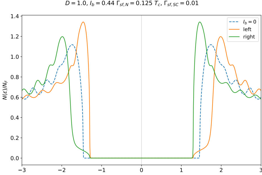
Figure 3.13: Momentum-resolved density of states in the presence of superflow for I_b = 0.44 .
