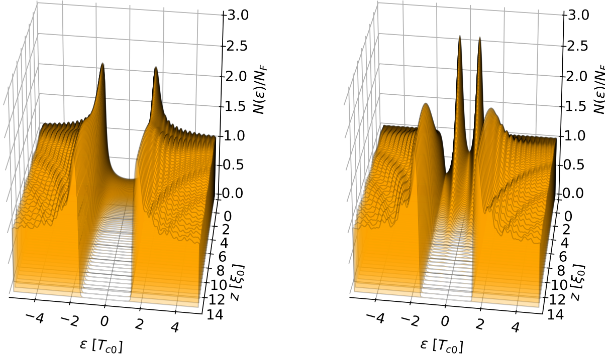
Figure 4.4: Density of states as function of energy and distance from the SAI (at z = 30\xi_0 ) for a spin-mixing angle of \vartheta = 0 (left plot) and \vartheta = 0.49\pi (right plot).
