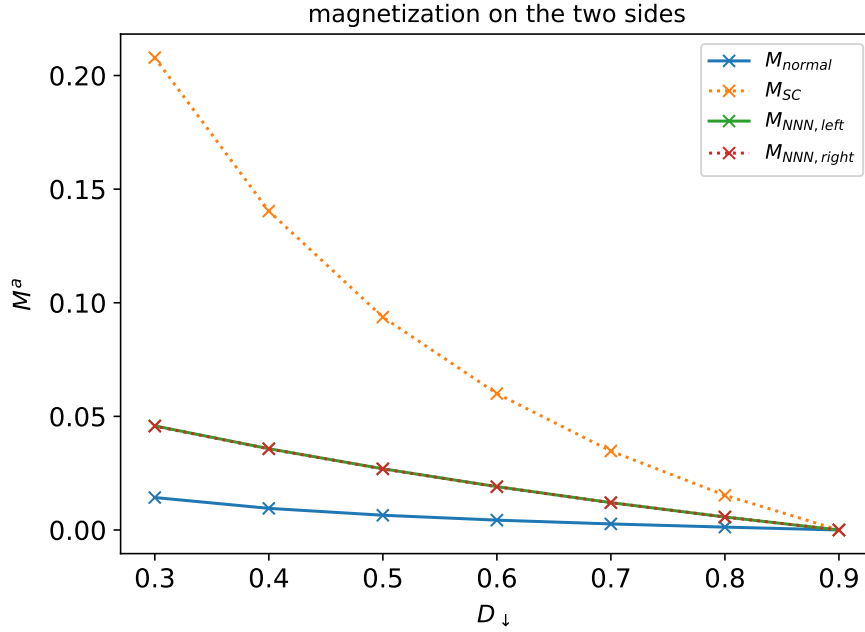
Figure 4.19: Magnitude of M^a(z) for the left and right side of the SAI in the NIN and NIS system for a medium current of I = 0.1 .
