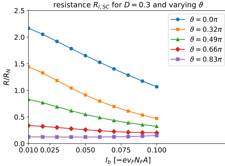
Figure 4.30: Resistance R_I at the SAI for D_{\uparrow} = D_{\downarrow} = 0.3 for different spin-mixing angle \vartheta and currents I .
