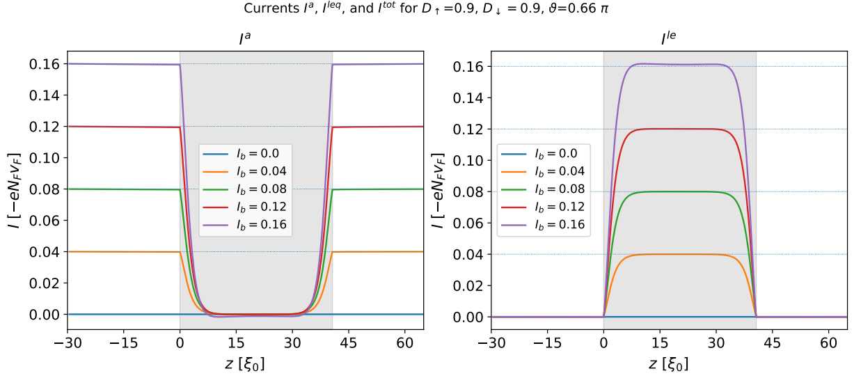
Figure 4.25: Conversion from normal-state "anomalous" current into supercurrent over the system. The dotted lines show the respective boundary current. The grey area marks the superconducting region.
