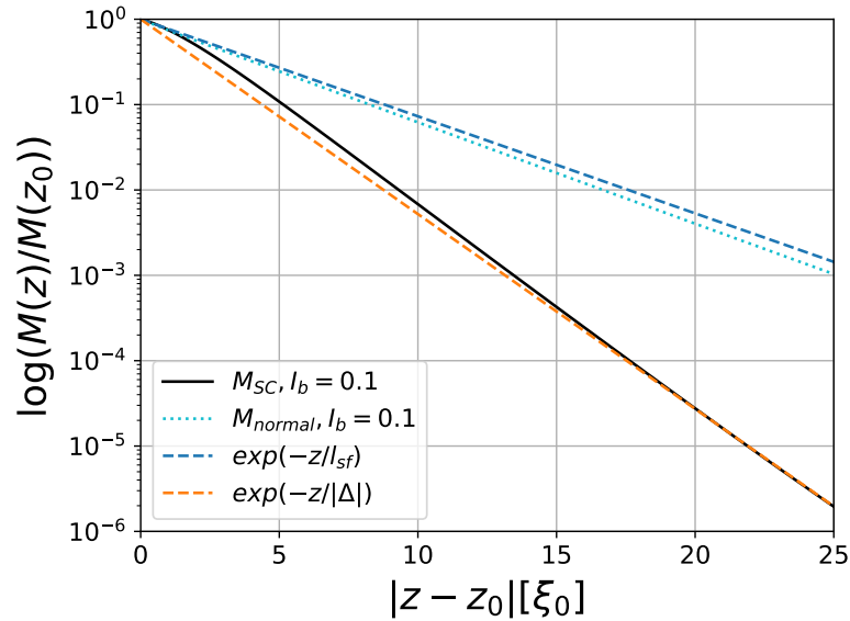
Figure 4.18: Decay of the magnetization M(z) away from the interface at z_0 = 0 into the normal and superconducting regions. The dashed lines are approximately the expected behaviour.
