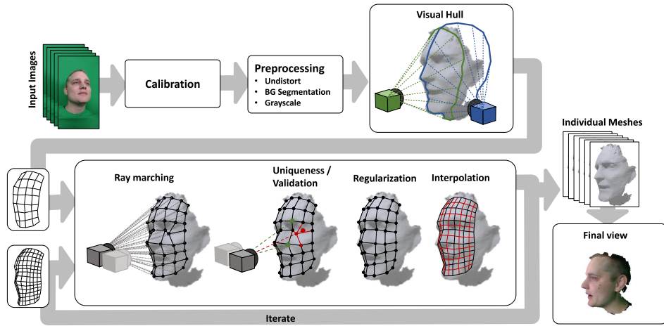
Figure 7: An overview of our real-time pipeline.
