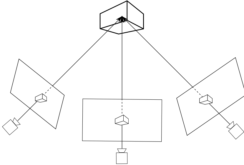
Figure 4: A position in world space can be computed by triangulating its position using two or more cameras.
