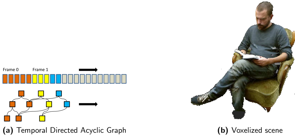
Figure 6: In a): the structure of the temporal DAG, where each frame has its own root node. Exploiting coherence in time, identical nodes can be found in previous frames and reused. In b): a frame from a scene voxelized from a recording using three Microsoft KinectV2 depth cameras.
