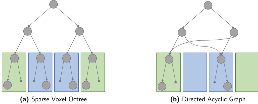
Figure 3: The Sparse Voxel Octree in a) is a hierarchical structure that only stores voxels where there is geometry. The Directed Acyclic Graph in b) is a compact version of this structure, where identical subtrees are merged and replaced by a pointer to its first occurrence.
