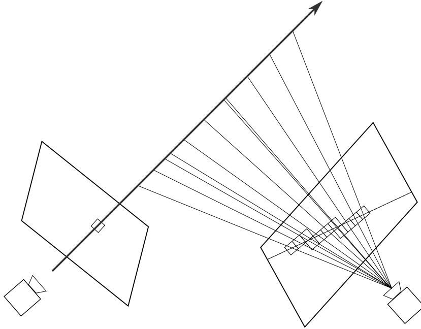
Figure 5: The depth resolution of a stereo reconstruction is dependent of the angle between the cameras and the resolution of each of the two cameras.
