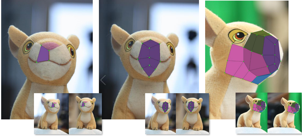
Figure 9: In the left-most image, the user starts modeling by placing a quad just at the front of the model, which is automatically aligned given two views. In the middle image, further quads have been placed out in the same views. In the right-most image, other views with better visibility have been chosen, signified by a unique color.
