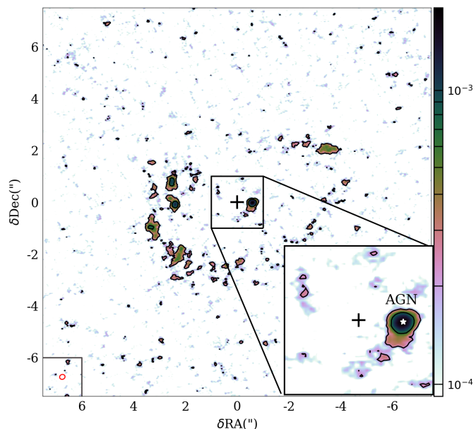
Fig. 2. Continuum emission at 0.87 \text{ mm} . The central 15'' \times 15'' are shown in the main panel, the zoom-in of the central 2'' \times 2'' is shown in the bottom right corner . The cross indicates the phase center, while the white star indicates the new center adopted in Table 1. The color scale is in \text{Jy/beam} . The beam size ( 0.21'' \times 0.19'' ) is shown in the red ellipse in the bottom left corner .
