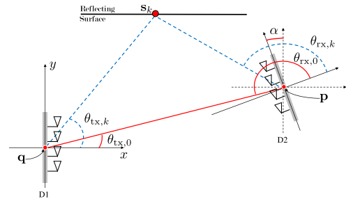
FIGURE 1. Two-dimensional MIMO system model with a D1 with known position and orientation, and a D2 with unknown position (p) and orientation (alpha), with reflective surface.
