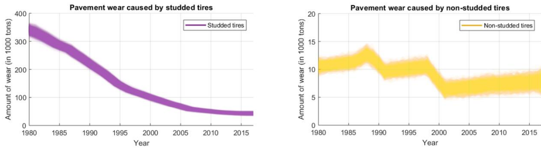
Fig. 18: Amount of pavement wear between 1980 and 2017
