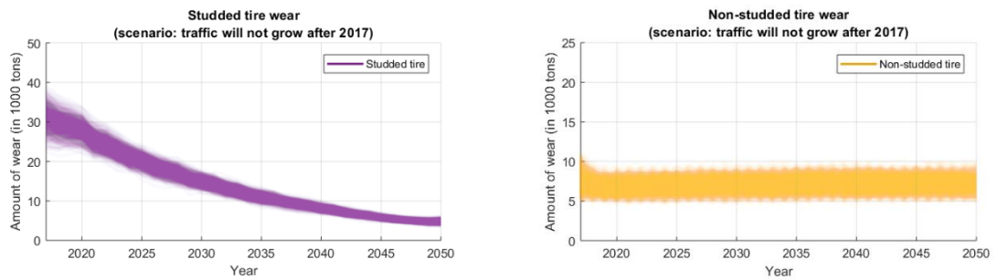
Fig. 19: Amount of pavement wear between 2018 and 2050 based on Scenario 1
