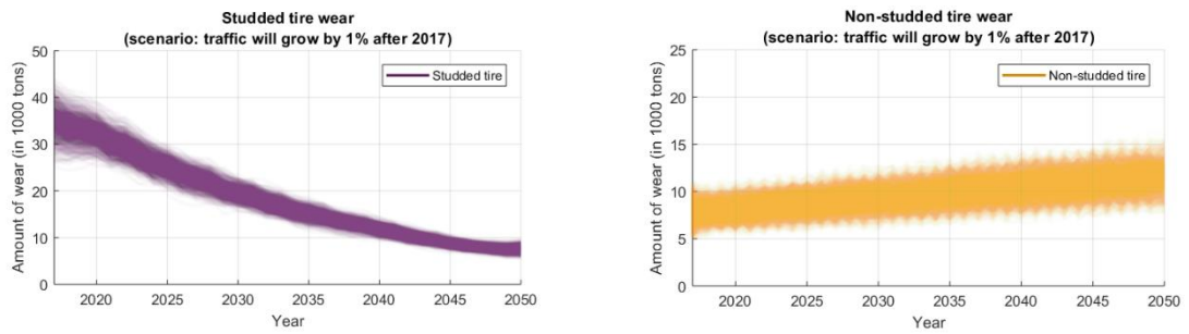
Fig. 20: Amount of pavement wear between 2018 and 2050 based on Scenario 2
