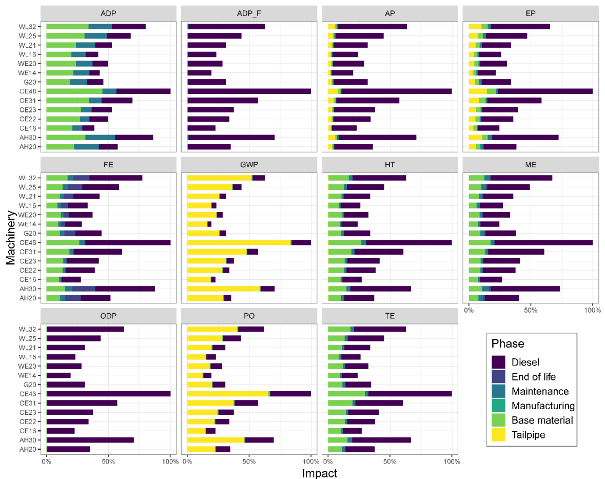
Fig. 11: Normalized impact assessment of results
