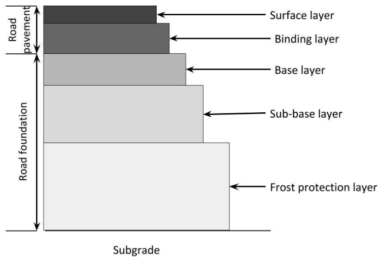
Fig. 15: Common layered structure for a road infrastructure, adapted from a published report (NPRA, 2014)
