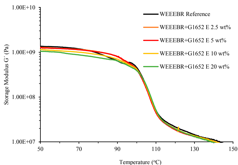
Figure 5. Storage modulus as a function of temperature for WEEEER with different amounts of compatibilizer.
