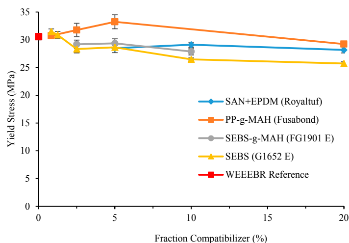
Figure 4. Yield stress of WEEEER with the compatibilizers used and non-compatibilized WEEEER. The error bars represent the standard deviation.
