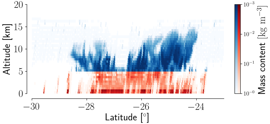
Figure 3.1: Mass content of frozen (blue) and liquid hydrometeors retrieved from the radar reflectivities show in Fig. 1.2
