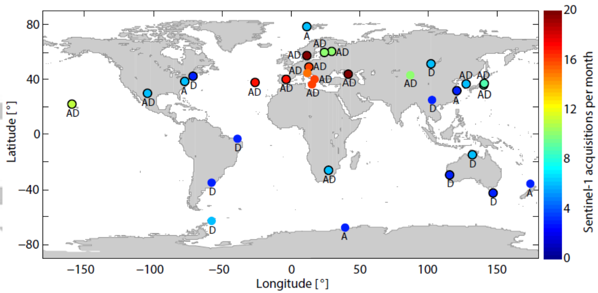
Figure 1: The global network of the International VLBI Service (IVS) telescopes. Circles with black outlines indicate sites where next generation VLBI Global Observing System (VGOS) instruments will be, or are already, located. All telescopes are imaged by the European Space Agency SAR satellite constellation Sentinel-1 in either (or both) a south to north ascending orbit (labelled A) or north to south descending orbit (labelled D) at a repeat frequency of between one and 12 days.
