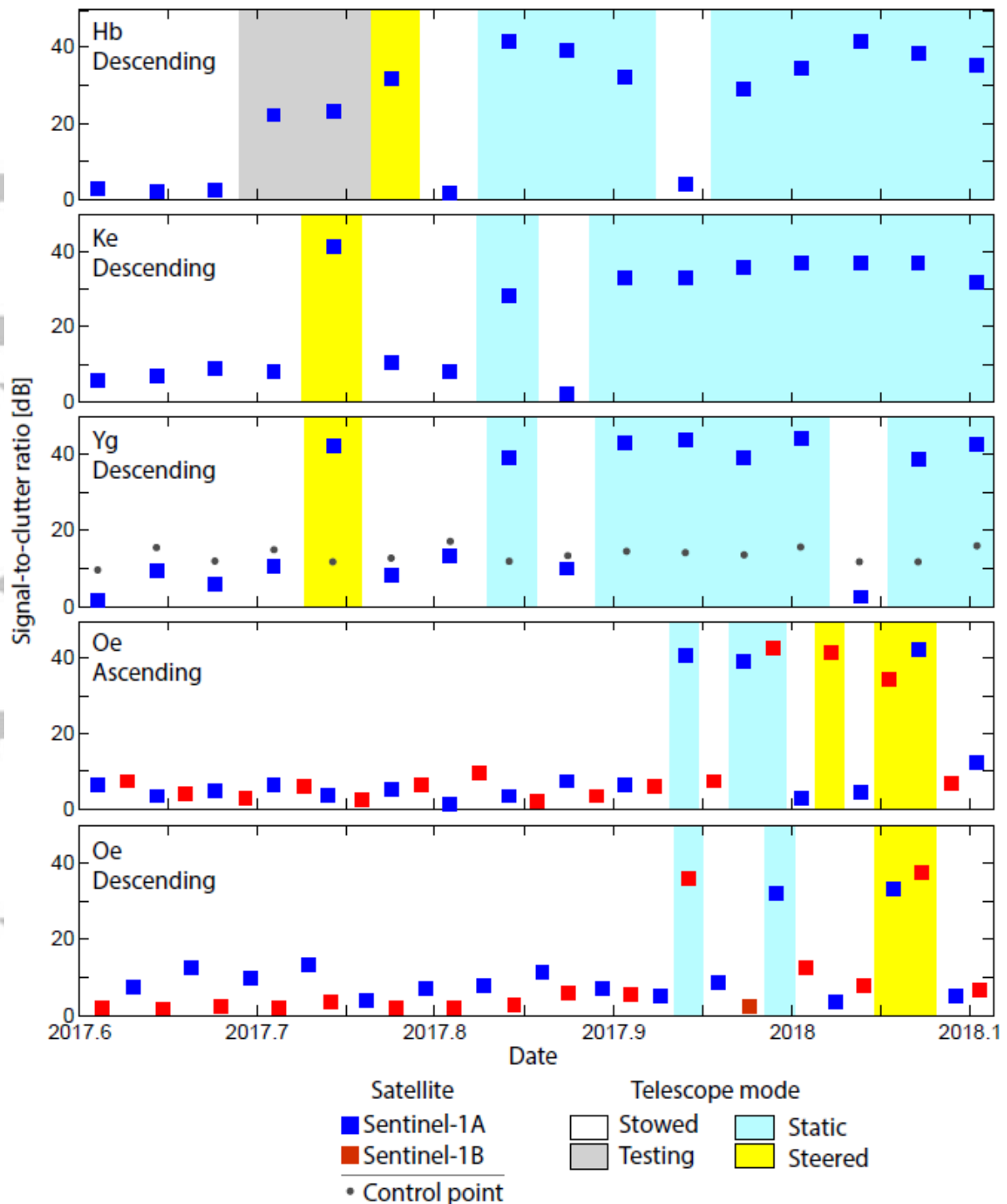
Figure 3: Time series of signal-to-clutter ratios at four VLBI telescopes. Hb (Hobart), Ke (Katherine) and Yg (Yarragadee) are located in Australia. Oe is located in Sweden. The initial testing phase at Hb was undertaken to ensure protection of receiver electronics. The ground control point show for Yg is a man-made building situated ~300 m from the telescope.
