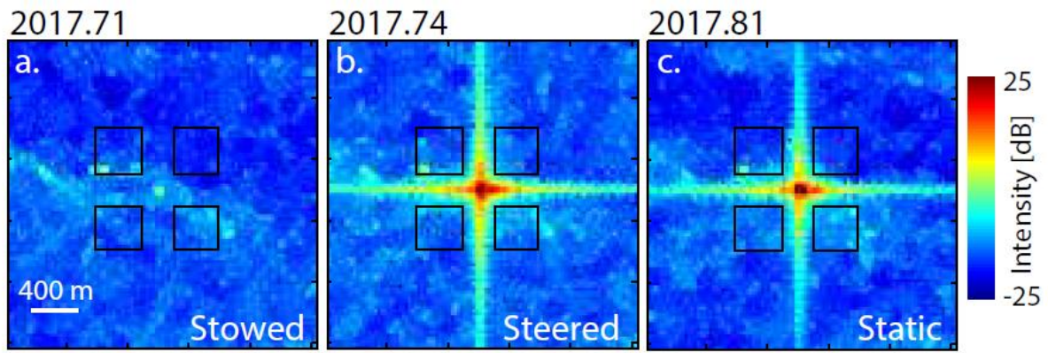
Figure 2: SAR intensity imagery for different telescope tracking modes. Results are for telescope Yg (Yarragadee, Australia) showing (a) the telescope stowed in the near-zenith stowed position and the impulse response observed when tracking Sentinel-1A via (b) steered and (c) static orientations. Black windows show the region used to calculate the background “clutter”. Images are in radar co-ordinates.
