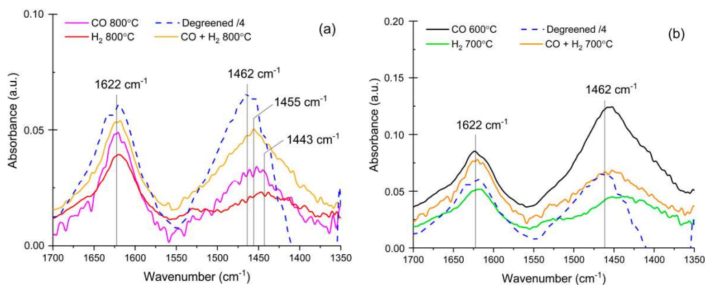
Figure 7. DRIFT spectra of NH 3 adsorption at 150 °C (1000 ppm, 20 min) recorded after pretreatment at 500 °C (8% O 2 in Ar, 30 min). (a) Catalysts aged at 800 °C and (b) catalysts aged at 700 °C and 600 °C. The degreened catalyst signal was divided by 4, and the aged catalysts were crushed monolith, containing ca. 75 wt % cordierite.
