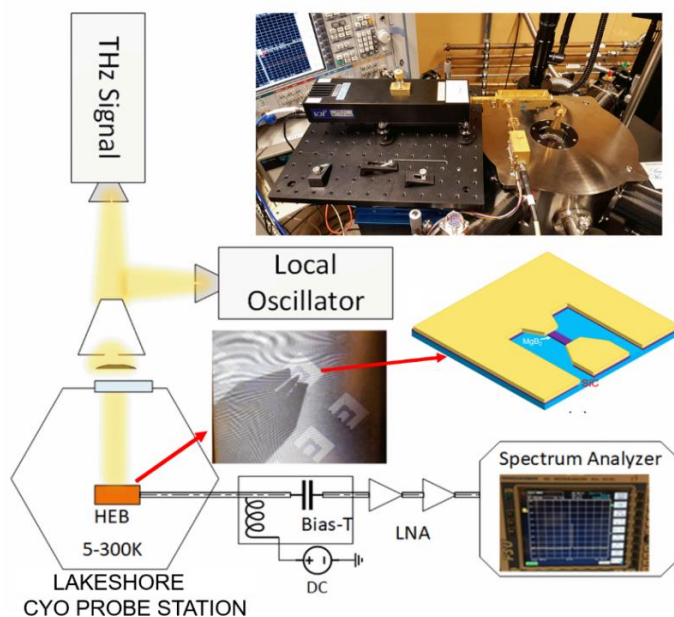
Fig. 1 Experimental set up for both the noise and the gain bandwidths of NbN and MgB 2 HEB mixers. The microwave probe with ground-signal-ground (GSG) contacts and schematic of CPW contact pad along with HEB are shown in the middle. The photograph of the actual set up and the Lakeshore cryo probe station is shown on the top.
