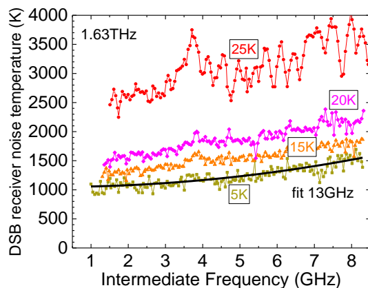
Fig. 2 DSB receiver noise temperature of MgB 2 HEB measured at a 1.63 THz LO, at various temperatures from 5 K to 25 K. The solid curve at 5 K represents the fit for f_N = 13 GHz noise bandwidth.
