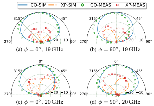
Fig. 7. Normalized radiation pattern at 19 GHz on (a) \phi = 0^\circ and (b) \phi = 90^\circ , and at 20 GHz on (c) \phi = 0^\circ and (d) \phi = 90^\circ .
