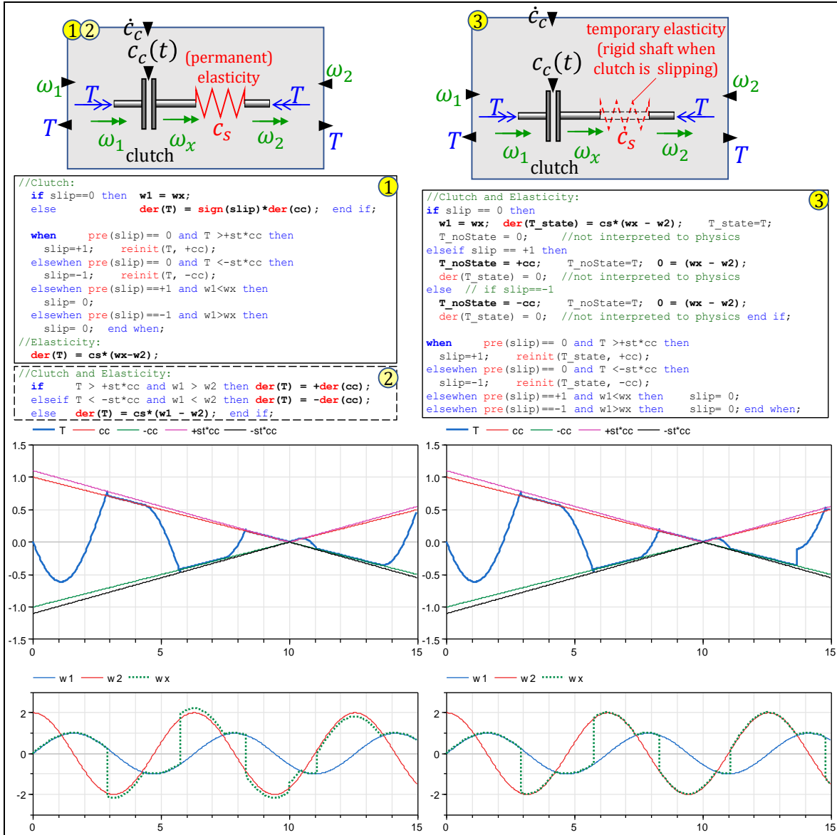
Figure 2-70: Model of clutch and elasticity in series, modelled for speed input from both sides. Implemented in Modelica. Implementation 2 (without discrete state and without when ) only works well (without chattering) for st = 1.0 . Implementation 3 uses a different physical model which has different number of states depending on the discrete state slip ; elasticity is modelled only when slip = 0 .
