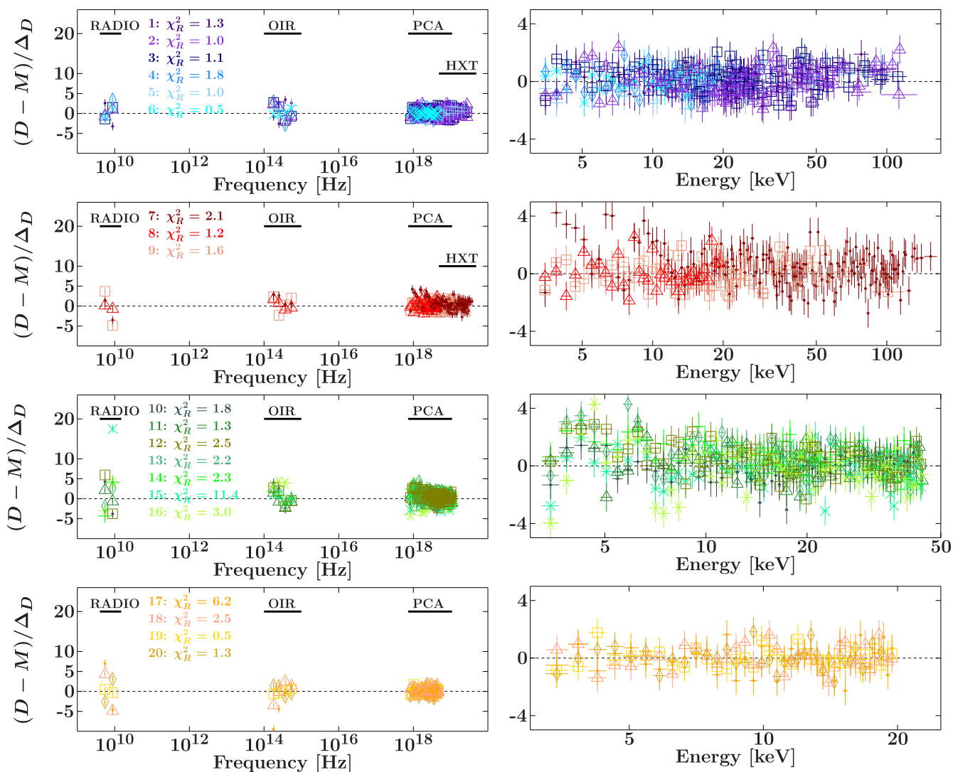
Figure 10. Standardized residuals [(\text{data}-\text{model})/\text{uncertainty}] of fits to all 20 broad-band spectra of GX 339–4 with Model B2 (coronal IC-dominated X-ray spectra): \text{tbabs} \times [\text{reflect}(\text{agnjet}+\text{nthcomp}) + \text{Gaussian}] , with typical \chi_R^2 \sim 1 –2, with some outliers. Each panel shows fits to observations within 2005, 2007, 2010, and 2011, respectively. Radio, OIR, and X-ray data are labelled, and different symbols/colours indicate the broad-band data-model residuals for each fit. The coronal emission ( \text{nthcomp} ) dominates the X-ray spectra, with SSC and IC scattering of disc photons in the jet contributing, and all emission reflecting off the disc.
