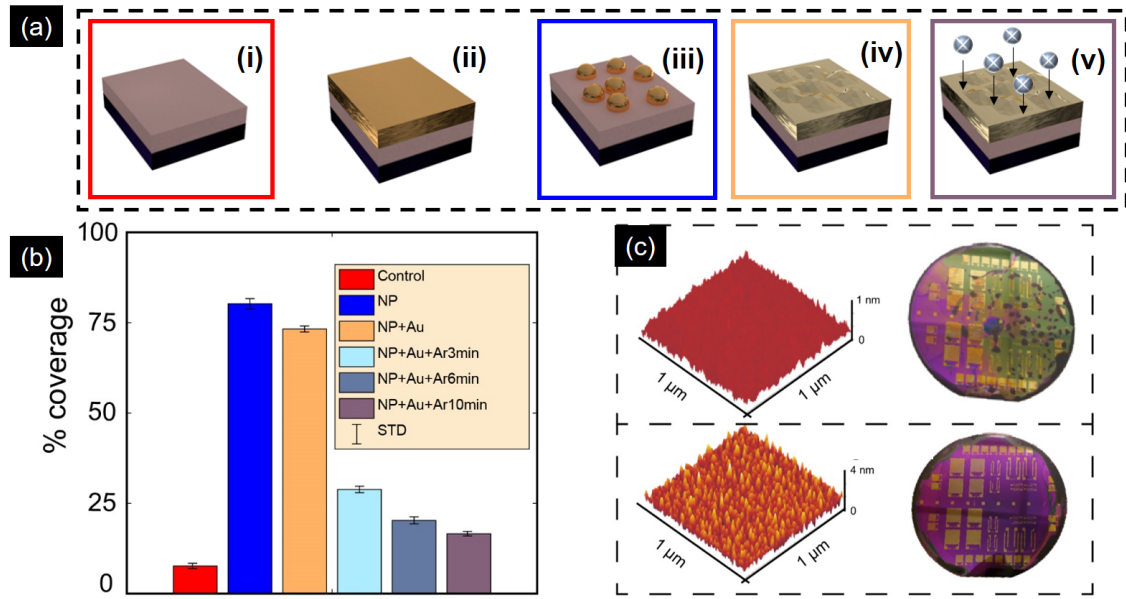
Figure 3.9: (a) Schematic fabrication process for the surface optimization of MSCs for an improved spin coating process. (b) Coverage of the wafer surface after using different optimization techniques. (c) (a) AFM comparison of roughened and non-roughened sample surfaces along with optical microscopy images showing the coverage of the electrode spin-coating.
